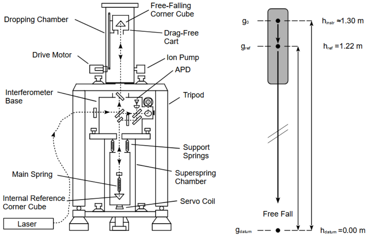
Figure 3: FG5 sketch adapted from Micro-g Solutions (1999) showing the height of the top of the drop position (e.g., h_{\text{instr}}=1.30 m) in the dropping chamber above the ground floor marker ( h_{\text{datum}}=0.00 m) and height adopted as common reference ( h_{\text{ref}}=1.22 m) for the time series of gravity values at Brest (see text).
