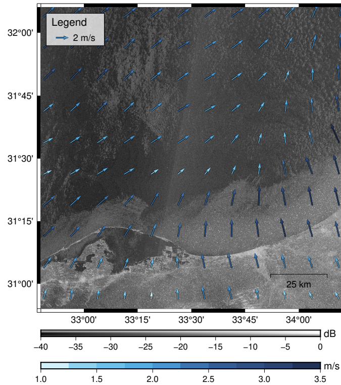
Figure 8. An example of land breeze fronts in the SAR scenes taken at 03:44 on 2 August 2023 near Egypt, plotted with the simulated wind speed at 04:00 obtain from CMEMS (c). The figure contains modified Copernicus Sentinel data [2023]. The plotted coastline was obtained from Wessel and Smith (1996).
