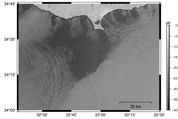
(a) Sentinel-1 SAR
