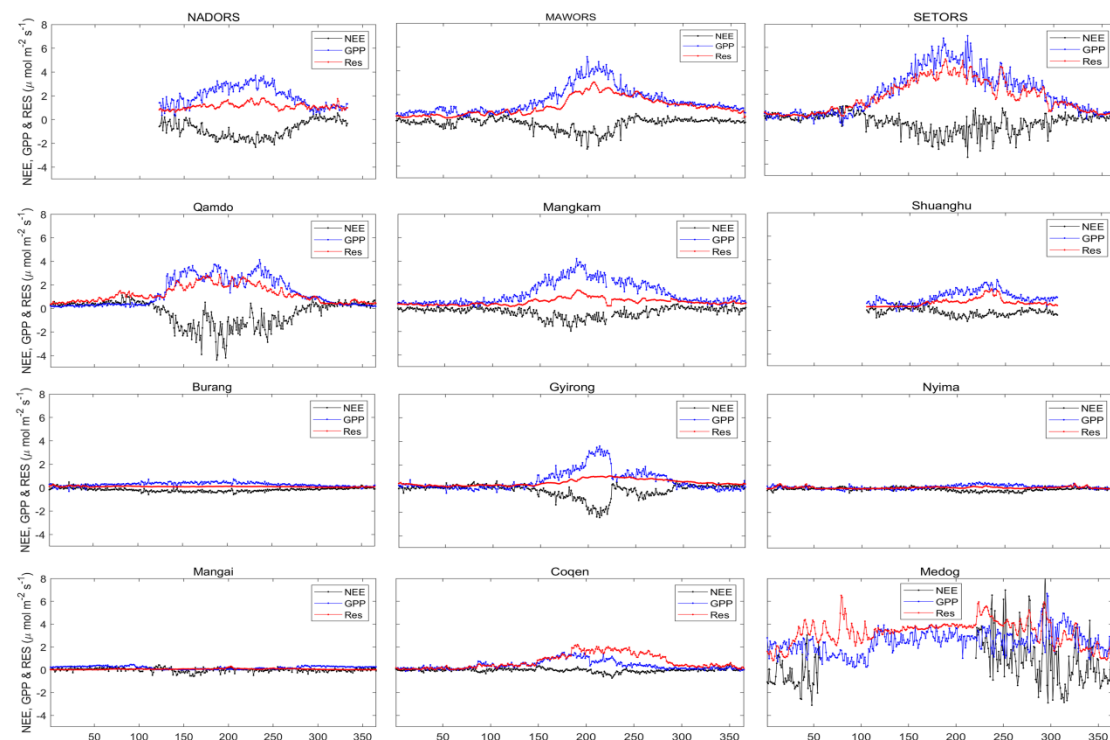
Figure 6. The seasonal variations in GPP , Re , NEE across different sites. The negative NEE values indicated a net uptake of \text{CO}_2 . (The black, blue and red line stand for daily NEE , GPP and Re , respectively).
