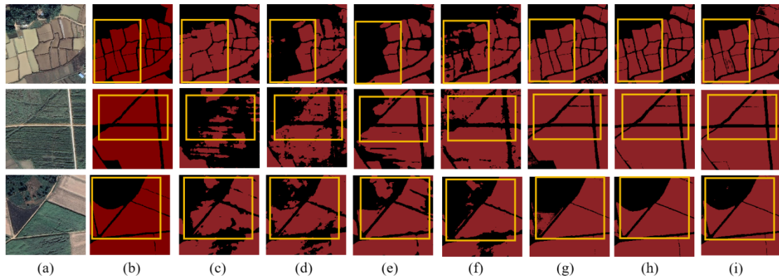
605 Fig. 26 Farmland segmentation results of different methods in Yungui Plateau . (a)Original image. (b)groundtruth. (c)U-Net. (d)Deeplabv3. (e)FCN. (f)SegFormer. (g)PixelLM. (h)LaSagna. and (i)LISA.
