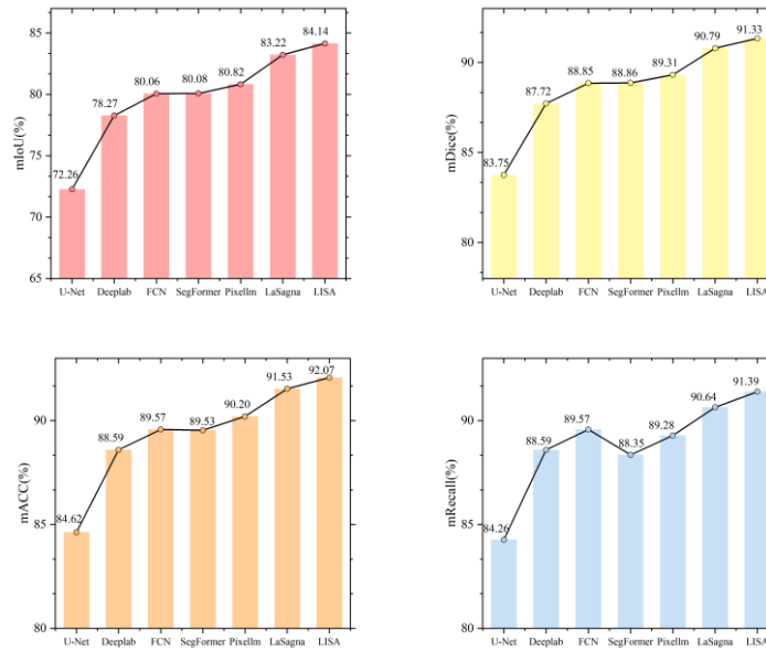
Fig. 15. Farmland segmentation results of different methods in Yangtze River Middle and Lower Reaches Plain.
