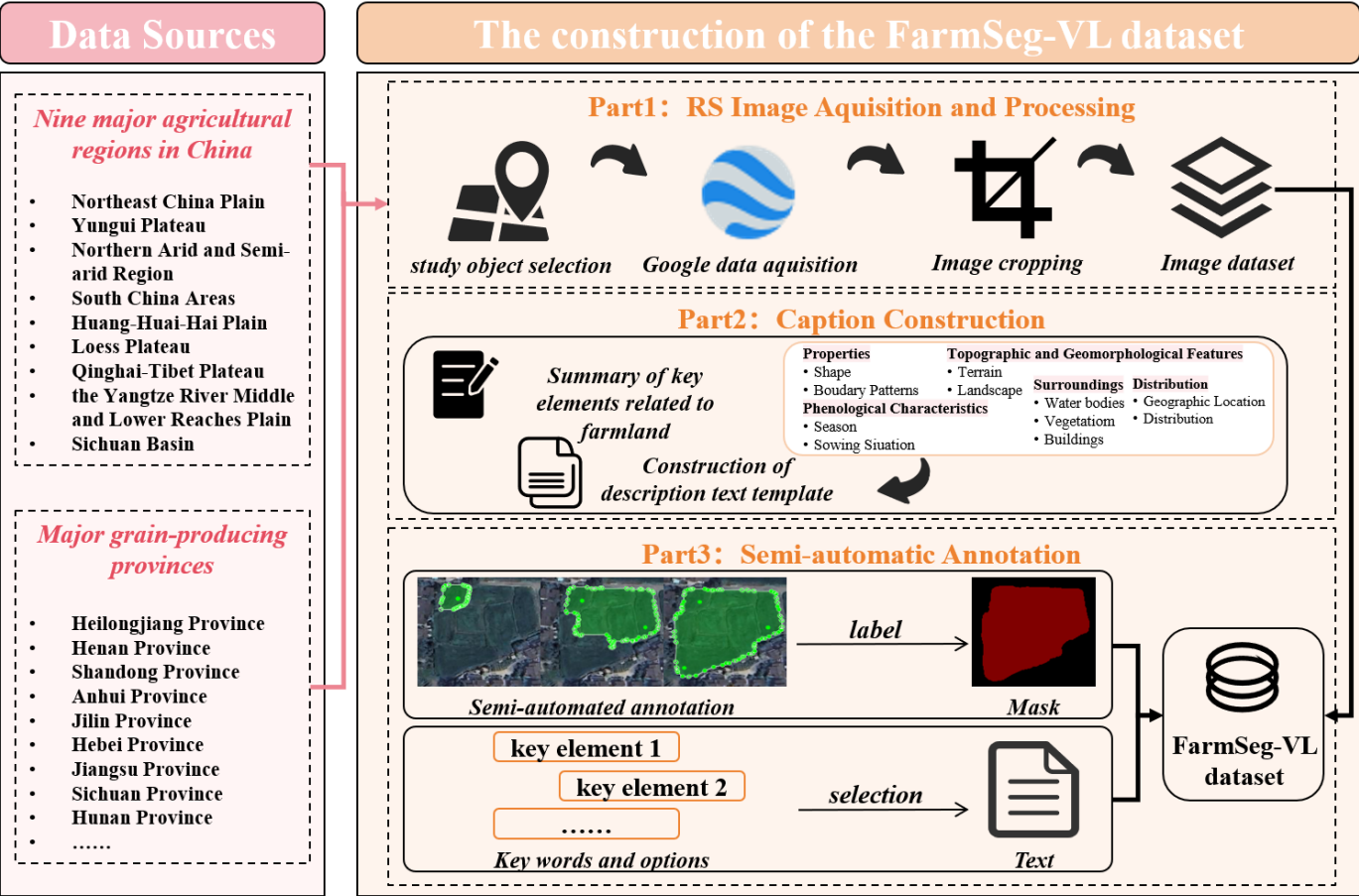
Fig. 1. Dataset construction.
