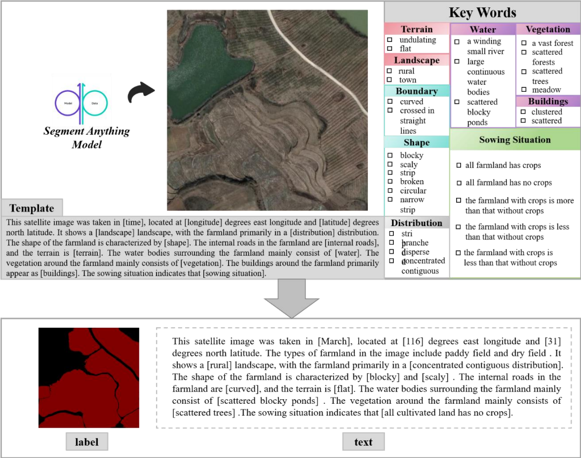
Fig. 5. Farmland semi-automated annotation framework.
