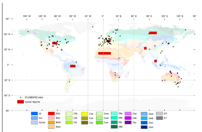
Figure 1. Spatial distribution of PLUMBER2 sites considered in this study and their corresponding climate zones, as well as the eight typical regions selected for seasonal comparisons and showing diurnal characteristics of FluxHourly data.
