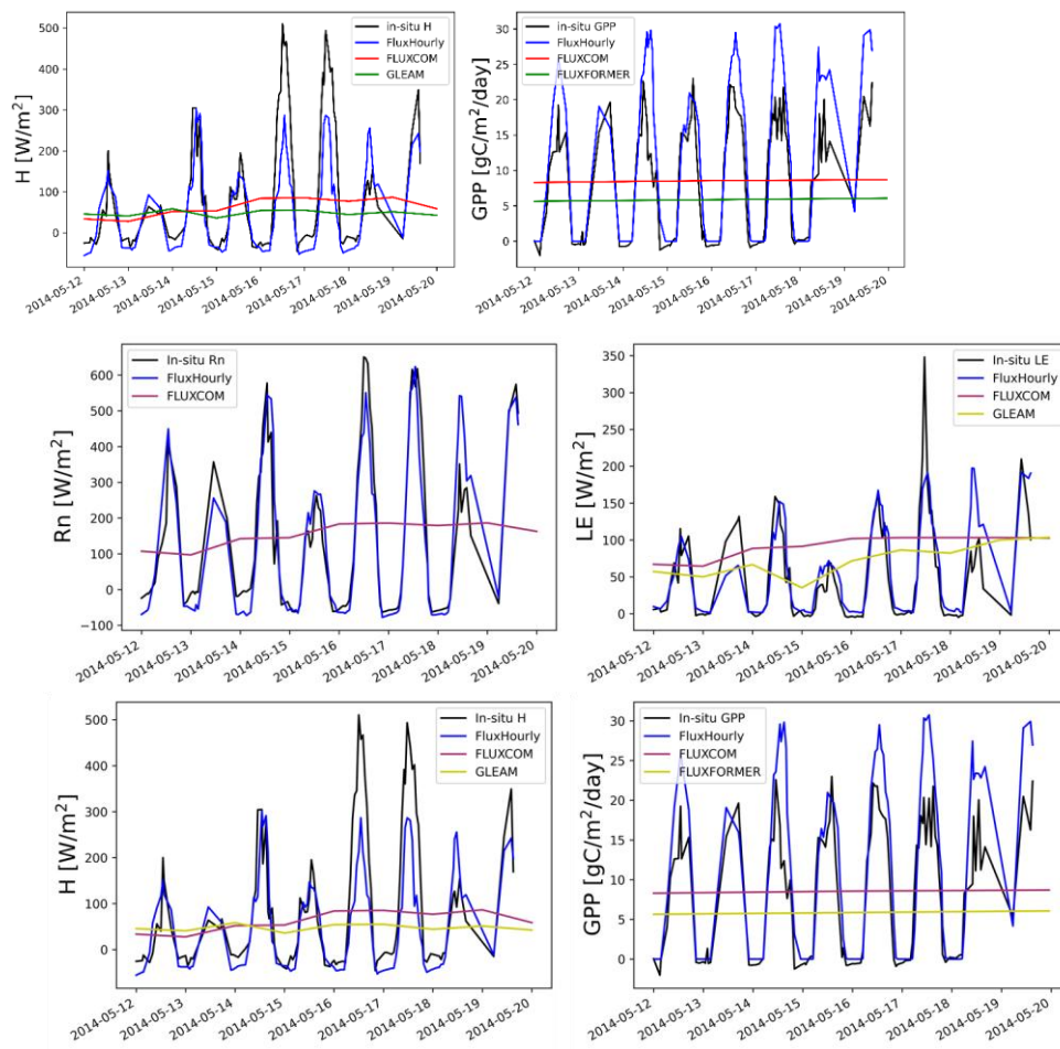
245 Figure- 5. Hourly FluxHourly, daily/monthly FLUXCOM and FLUXFORMER, daily GLEAM in at station BE-Vie: R_n , LE , H , GPP (Time is local time)
