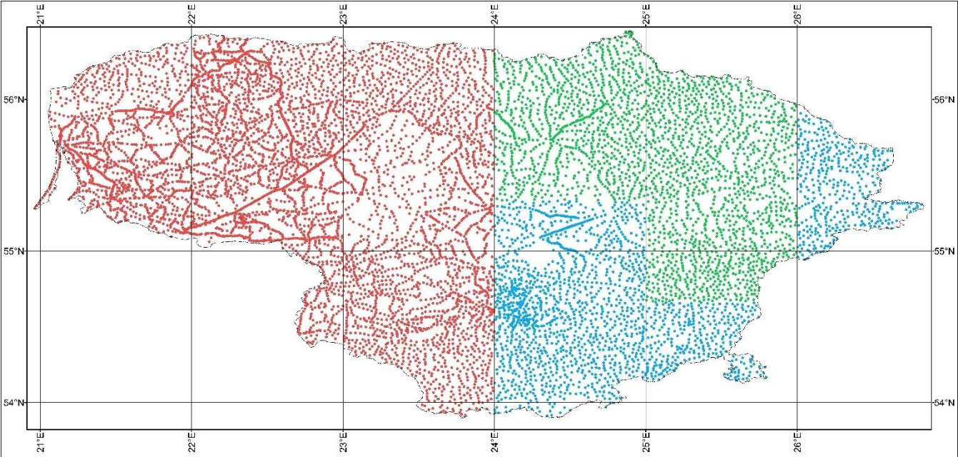
Figure 1: Distribution of the historical gravimetric points in the territory of investigation and compilation. Colours indicate the types of normal heights used in the compilation (see Figure 5).
