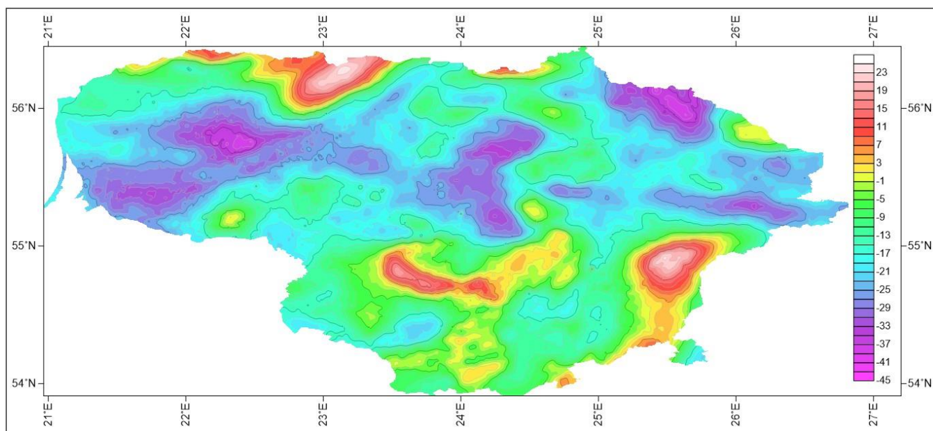
Figure 12. Bouguer anomaly map (contour interval is 2 mGal).
