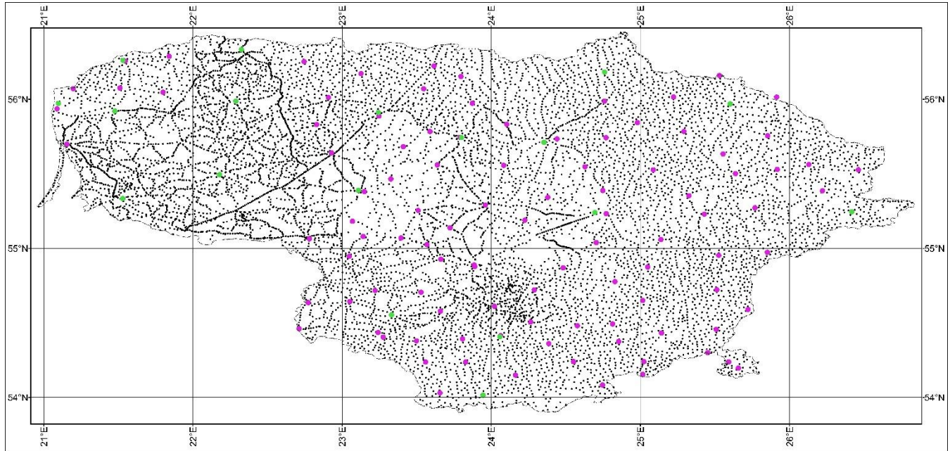
265 Figure 11. Spatial distribution of gravimetric points of all historical gravity data set (green dots – second order stations; magenta dots – third order stations; black dots – gravity survey points).
