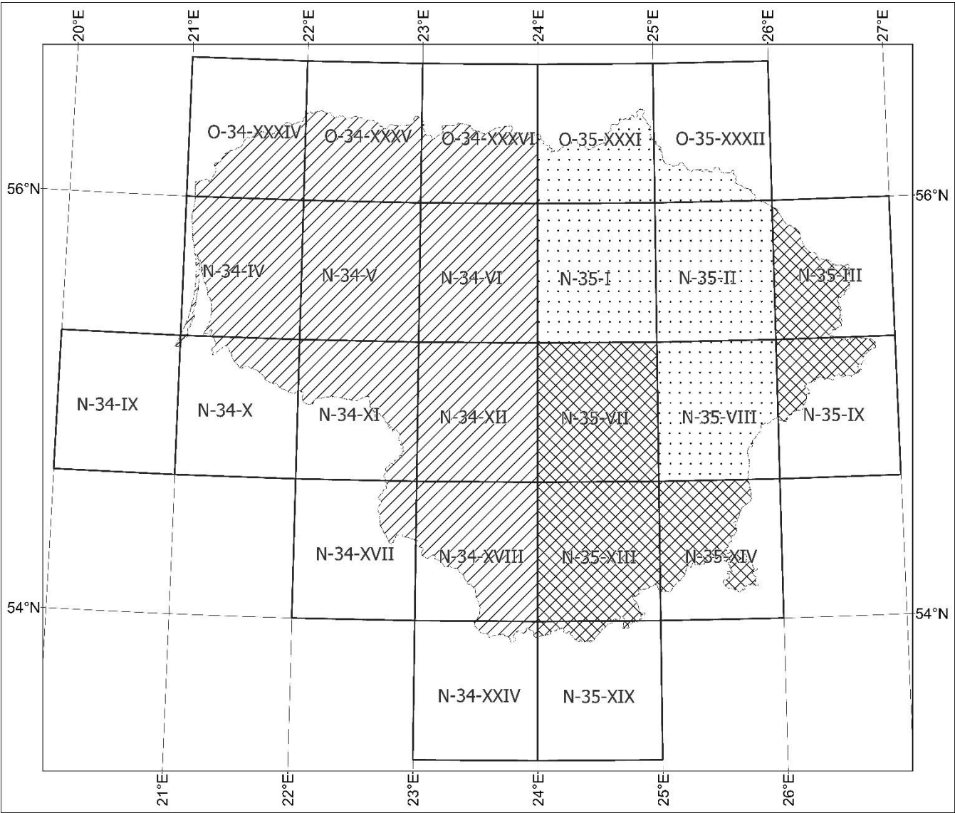
Figure 5: Types of map sheets to detect the normal heights of the gravimetric points. Patterns indicate the types of map sheets used in the compilation: dots – map sheets containing the normal heights; cross-lines – normal heights derived from Bouguer anomalies and free air anomalies; lines – normal heights interpolated from topographic map.
