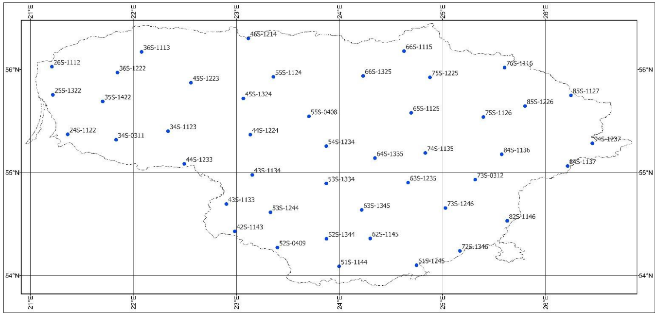
145 Figure 9: Distribution of geodetic points used for the transformation parameters calculation
