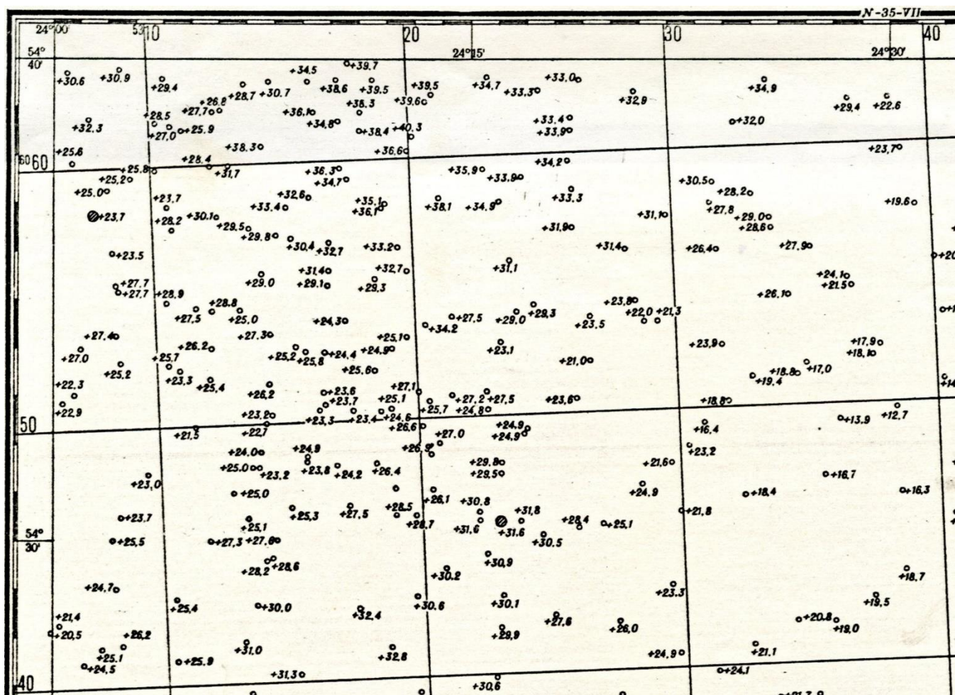
Figure 6: Example of a map sheet containing the free air anomalies (in mGal). (The firm, 1965).
