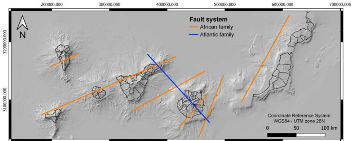
Figure 3. Volcano-tectonic lines of the Canary Islands' region. Source: adapted from Bosshard & Macfarlane (1970), and Mezcua et al. (1992). *Note: Orange lines = African family of faults; blue lines = Atlantic family of faults. Fault traces are not to scale nor is the location accurate, but are indicative. 145
