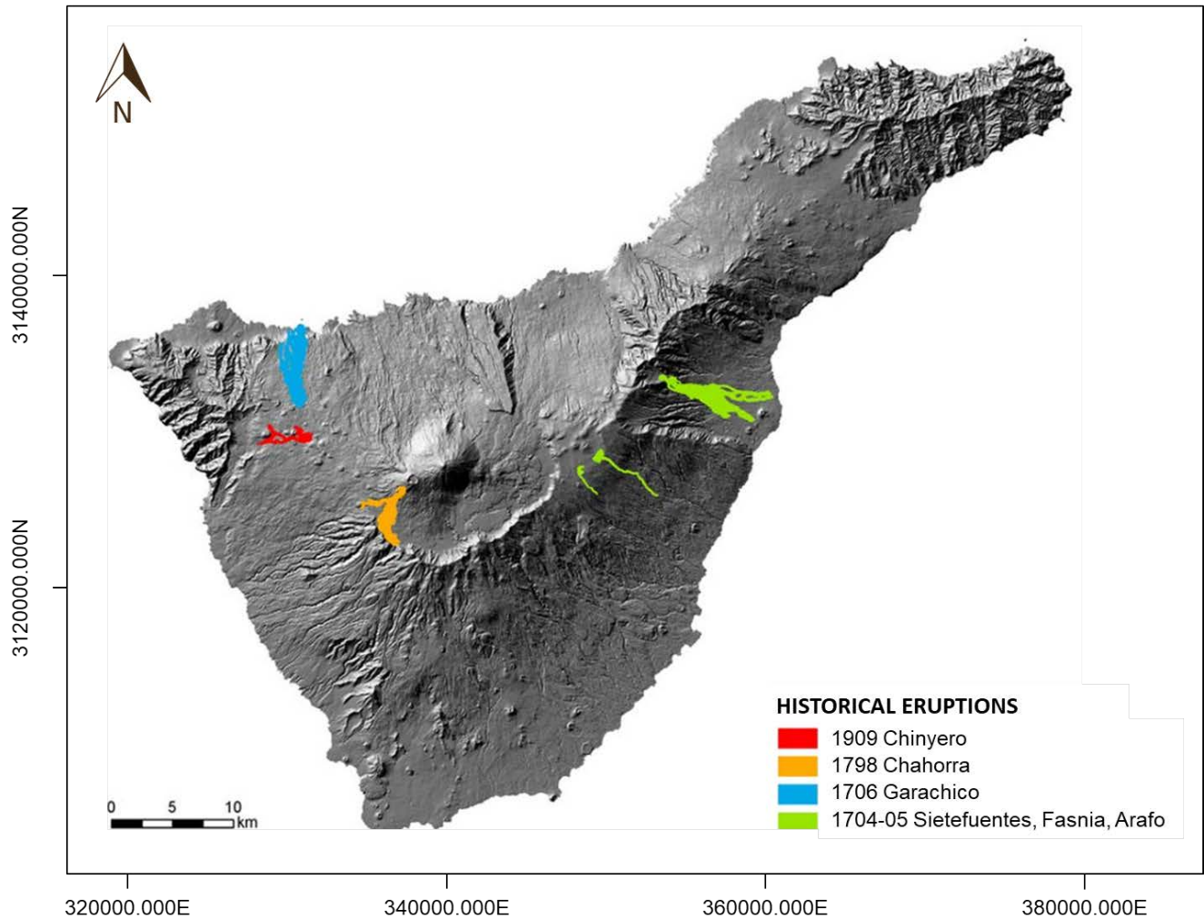
125 Figure 2. Map of the historical eruptions of Tenerife (Canary Islands). Source: adapted from IGN (n.d.).
