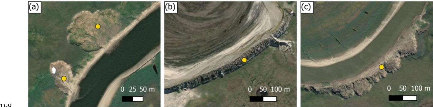
168 169 Figure 6 Examples of the three main RTS morphologies mapped in West Siberia: (a) Two thermocirques (yellow dots); (b) A 170 large thermoterrace (yellow dot); (c) A combined RTS morphology of merged thermocirques or merged thermocirque and a 171 thermoterrace (yellow dot). ESRI basemap used has the following credits: Esri, DigitalGlobe, GeoEye, i-cubed, USDA FSA, USGS, 172 AEX, Getmapping, Aerogrid, IGN, IGP, swisstopo, and the GIS User Community.
