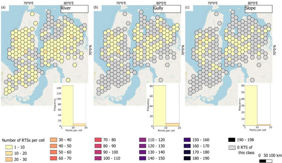
Figure A1. Density maps of RTS points counted per 30 x 30 km hexagonal grid cell located at the (a) river, (b) gully, and (c) slope. Projection: WGS 84 UTM Zone 43. Basemap: OSM Standard.
