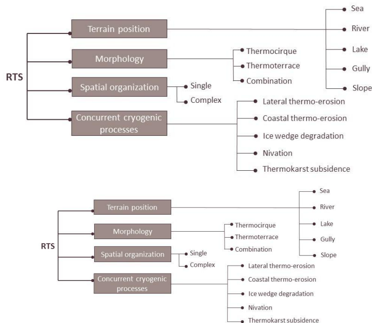
Figure 5 RTS classification scheme with four main criteria (shown as grey blocks) and 15 variables.
