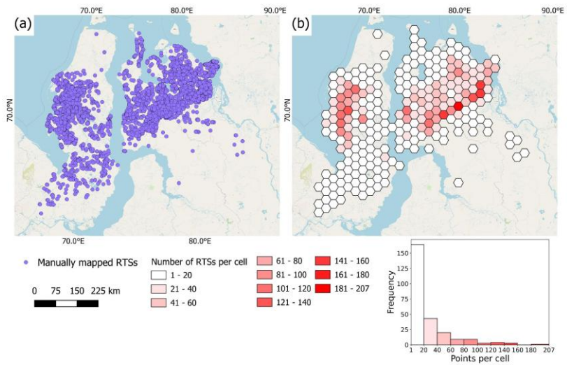
257 Figure 10 Distribution of all mapped RTSs: (a) Manually mapped RTSs (purple dots); (b) Density map of RTSs per 30 × 30 km 258 hexagonal grid cell. Projection: WGS 84 UTM Zone 43. Basemap: OSM Standard. 259
