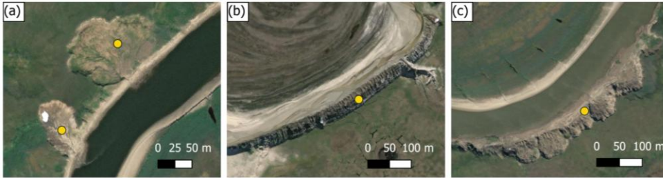
Figure 6 Examples of the three main RTS morphologies mapped in West Siberia: (a) Two thermocirques (yellow dots); (b) A single large thermoterrace (yellow dot); (c) A combined RTS morphology of merged thermocirques or merged thermocirque and a thermoterrace (yellow dot). ESRI basemap used has the following credits: Esri, DigitalGlobe, GeoEye, i-cubed, USDA FSA, USGS, AEX, Getmapping, Aerogrid, IGN, IGP, swisstopo, and the GIS User Community.
