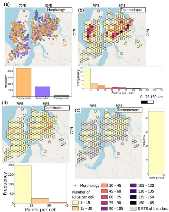
278 Figure 12 Distribution of all mapped RTSs: (a) Manually mapped RTSs classified by morphology; Density maps of RTSs per 30 × 279 30 km hexagonal grid cell classified as (b) thermocirque, (c) thermoterrace, and (d) a combination of both. Projection: WGS 84 280 UTM Zone 43. Basemap: OSM Standard.
