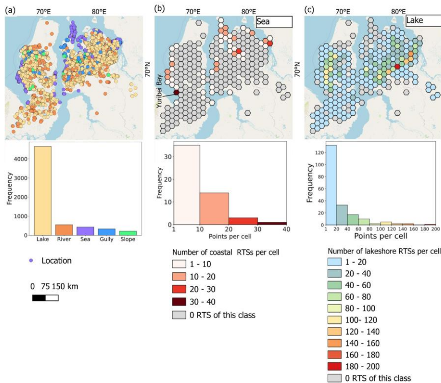
268 269 Figure 11 Distribution of all mapped RTSs: (a) Manually mapped RTSs classified by location; Density maps of RTSs per 30 × 30 270 km hexagonal grid cell located along the (b) seacoast and (c) lakeshores. Projection: WGS 84 UTM Zone 43. Basemap: OSM 271 Standard.
