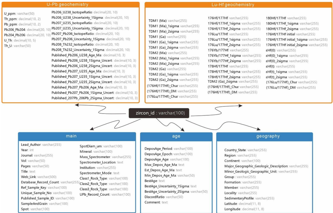
620 Figure 2: Schematic of the OneDZ relational schema. The three core tables (blue) and two geochemical tables are linked by the primary key zircon_id (varchar 100). Black underlines indicate primary keys; arrows denote foreign-key relationships.
