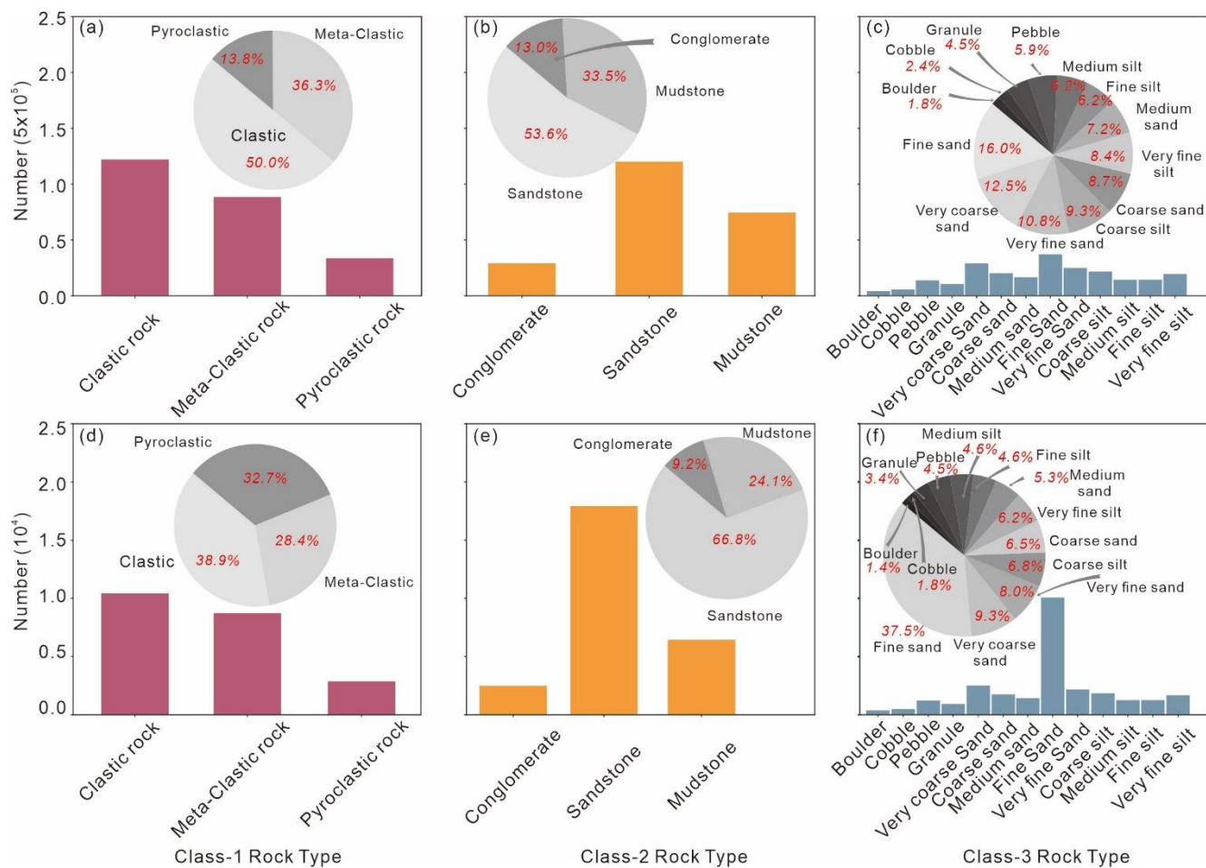
Figure 6: Statistics of the rock types. (a) Class-1 type in U-Pb database; (b) Class-2 type in U-Pb database; (c) Class-3 type in U-Pb database; (d) Class-1 type in Lu-Hf database; (e) Class-2 type in Lu-Hf database; (f) Class-3 type in Lu-Hf database.
