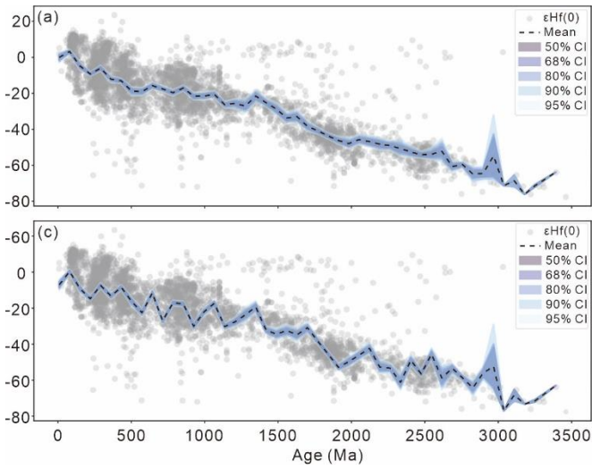
Figure 13: Temporal variations of \epsilon_{\text{Hf}} uncertainties in Lu-Hf dataset. (a) \epsilon_{\text{Hf}}(0) with bootstrap resampling; (b) \epsilon_{\text{Hf}}(t) with bootstrap resampling; (c) \epsilon_{\text{Hf}}(0) with Monte-Carlo resampling; (d) \epsilon_{\text{Hf}}(t) with Monte-Carlo resampling.
