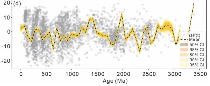
Figure 13: Temporal variations of \epsilon_{\text{Hf}} uncertainties in Lu-Hf dataset. (a) \epsilon_{\text{Hf}}(0) with bootstrap resampling; (b) \epsilon_{\text{Hf}}(t) with bootstrap resampling; (c) \epsilon_{\text{Hf}}(0) with Monte-Carlo resampling; (d) \epsilon_{\text{Hf}}(t) with Monte-Carlo resampling.
