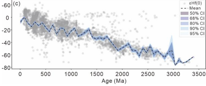
Figure 13: Temporal variations of \epsilon_{\text{Hf}} uncertainties in Lu-Hf dataset. (a) \epsilon_{\text{Hf}}(0) with bootstrap resampling; (b) \epsilon_{\text{Hf}}(t) with bootstrap resampling; (c) \epsilon_{\text{Hf}}(0) with Monte-Carlo resampling; (d) \epsilon_{\text{Hf}}(t) with Monte-Carlo resampling.
