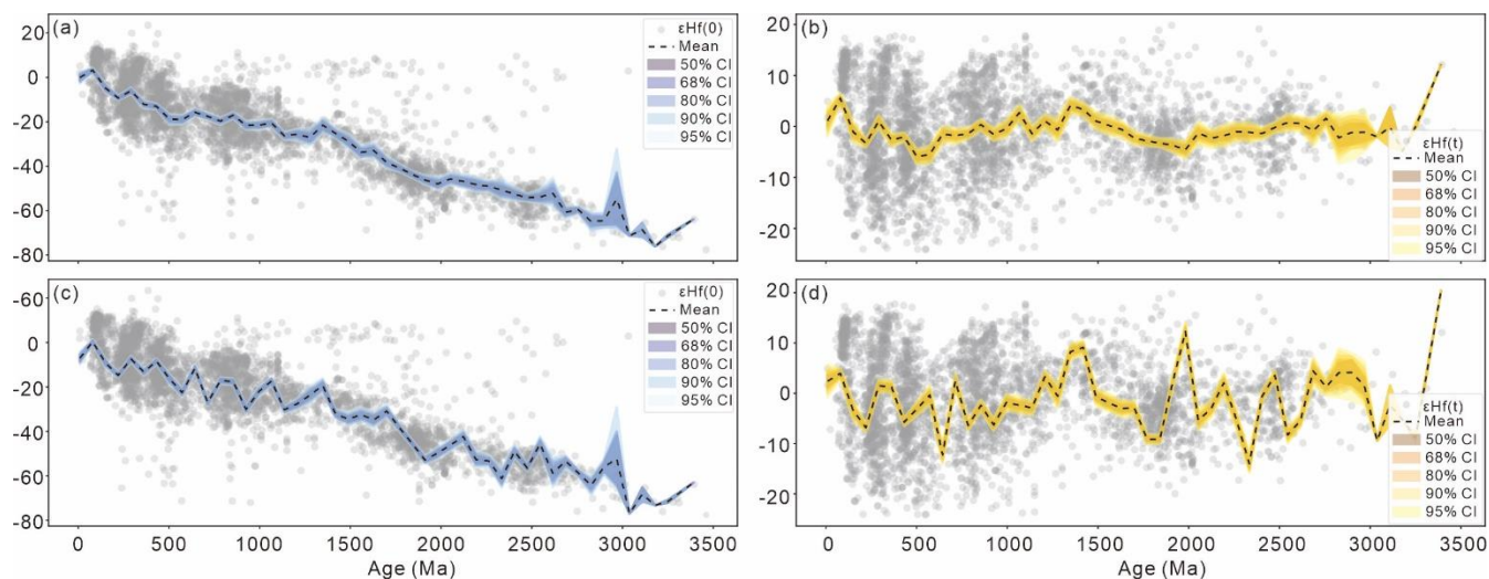
Figure 12: Temporal variations of \epsilon\text{Hf} uncertainties in Lu-Hf dataset. (a) \epsilon\text{Hf}(0) with bootstrap resampling; (b) \epsilon\text{Hf}(t) with bootstrap resampling; (c) \epsilon\text{Hf}(0) with Monte-Carlo resampling; (d) \epsilon\text{Hf}(t) with Monte-Carlo resampling.
