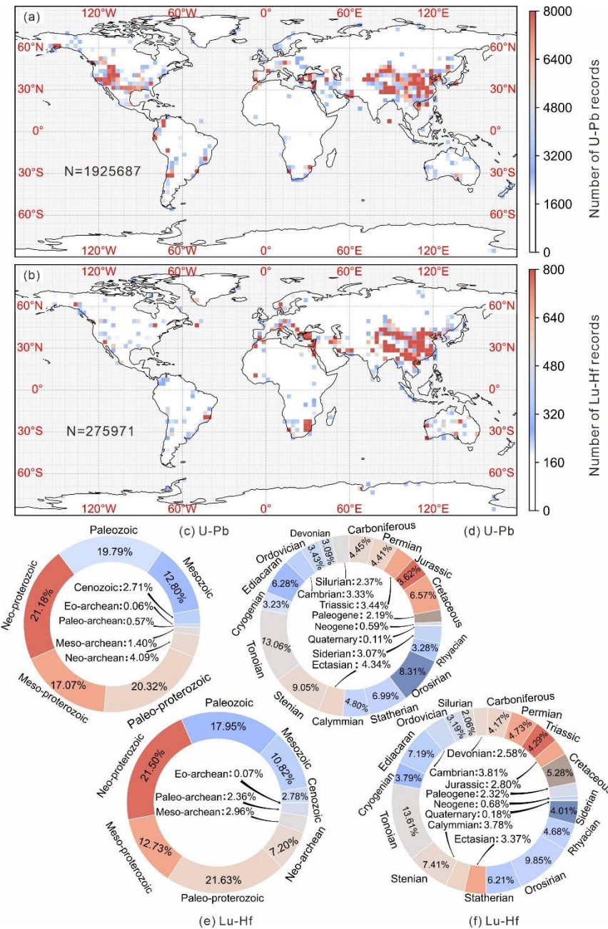
Figure 2: Temporal distributions of U-Pb and Lu-Hf isotopic records. (a) Kernel density estimate map of U-Pb records (the spatial resolution is 1^\circ \times 1^\circ ); (b) Kernel density estimate map of Lu-Hf records (the spatial resolution is 1^\circ \times 1^\circ ); (c) Era-based distribution of U-Pb samples; (d) Period-based distribution of U-Pb samples; (e) Era-based distribution of Lu-Hf samples; (f) Period-based distribution of Lu-Hf samples.
