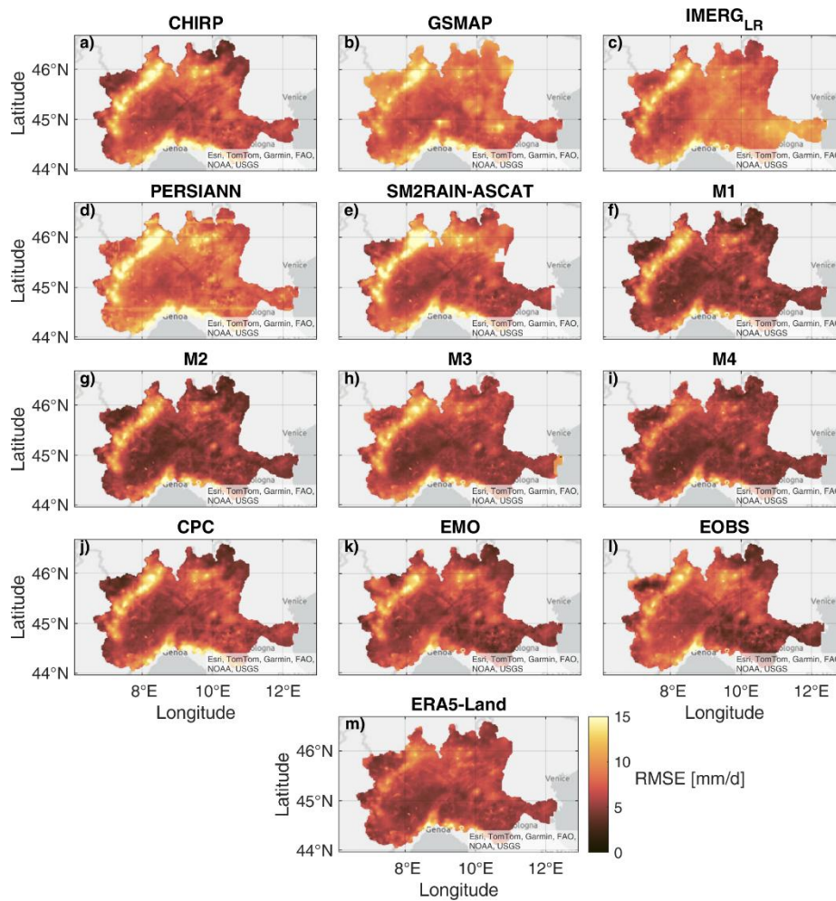
505 Figure 8: Root Mean Square Error (RMSE) of the selected precipitation datasets against MCM observations for the Po River basin area.
