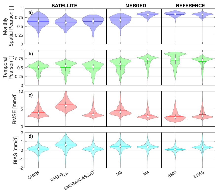
575 Figure 10: Spatial Pearson's correlation at monthly scale, Temporal Pearson's correlation, BIAS error and RMSE at daily scale for the full study area against E-OBS benchmark (10 km spatial sampling). For each violin, the white dot is the average value, the dark line the median value, and the shape of the violin reflects the data distribution.
