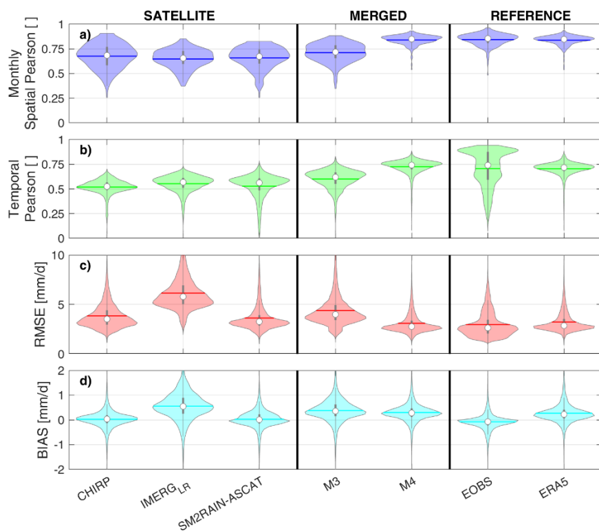
570 Figure 9: Spatial Pearson's correlation at monthly scale, Temporal Pearson's correlation, BIAS error and RMSE at daily scale for the full study area against EMO benchmark (10 km spatial sampling). For each violin, the white dot is the average value, the dark line the median value, and the shape of the violin reflects the data distribution.
