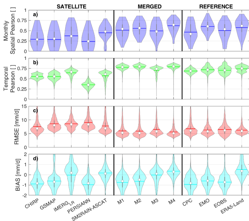
440 Figure 2: Spatial Pearson's correlation at monthly scale, Temporal Pearson's correlation, BIAS error and RMSE at daily scale for the Po River basin against MCM benchmark (1 km spatial resolution). For each violin, the white dot is the average value, the dark line the median value, and the shape of the violin reflects the data distribution.
