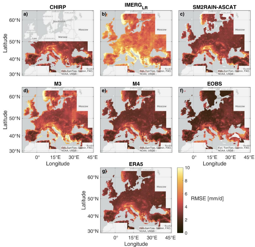
590 Figure 14: Root Mean Square Error (RMSE) of the selected precipitation datasets against EMO observations for the full study area. All the datasets are aggregated at 10 km spatial resolution.
