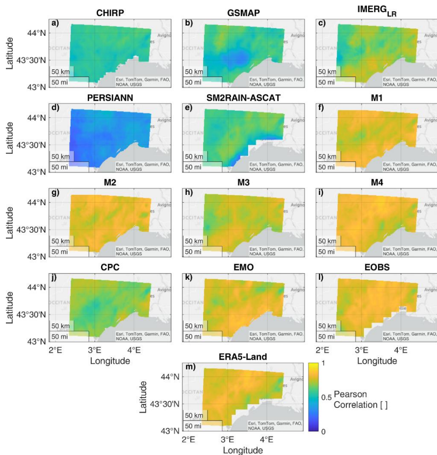
735 Figure B2: Daily temporal Pearson's correlation of the selected precipitation datasets against COMEPHORE observations for the Hérault River basin area.
