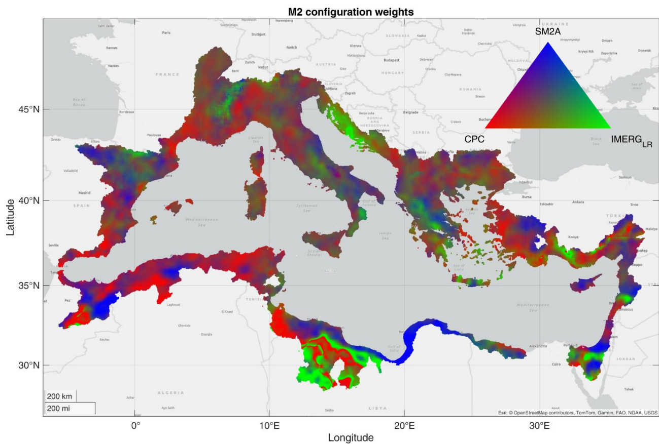
715 Figure A2 Weights distribution for configuration M2: areas colored in red, green and blue highlight the pixels where CPC, IMERG- LR and SM2RAIN-ASCAT have the greater weight, respectively.
