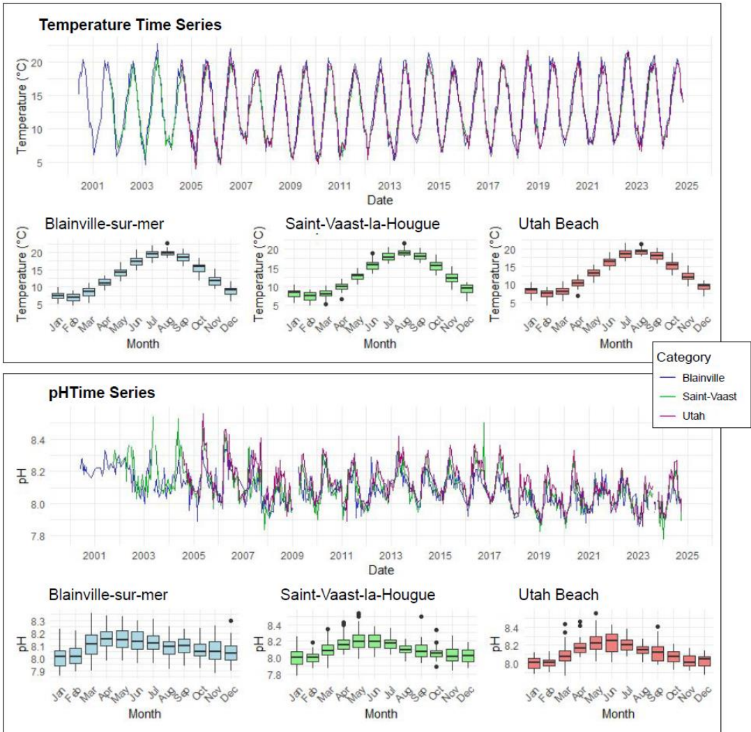
Figure 2: Time Series and Monthly Averages of Temperature (°C) (top) and pH (bottom) from 2000 to 2024 at Blainville-sur-Mer, Saint-Vaast-la-Hougue, and Utah Beach. Boxplots show the 25th–75th percentile range (interquartile range, IQR), with the median as a horizontal line. Whiskers extend to 1.5 \times \text{IQR} ; points beyond are outliers.
