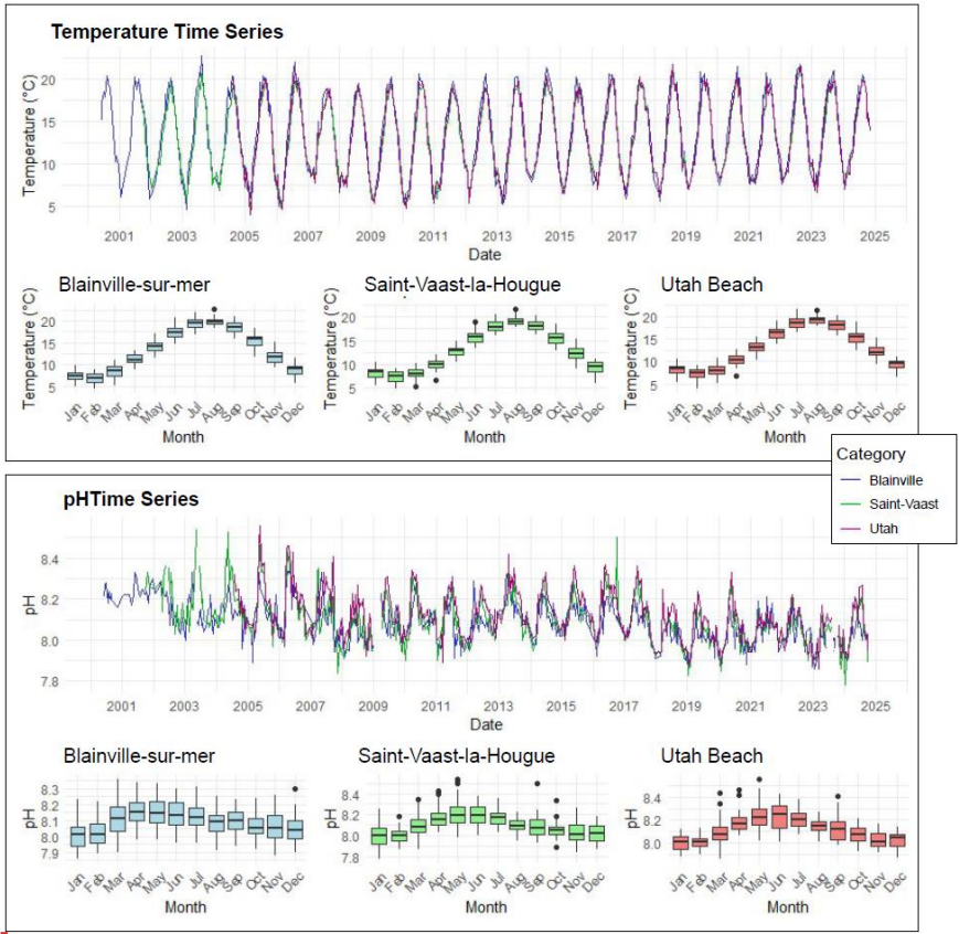
Figure 2: Time Series and Monthly Averages of Temperature (°C) (top) and pH (bottom) Parameters from 2000 to 2024 at Blainville-sur-Mer, Saint-Vaast-la-Hougue, and Utah Beach.
