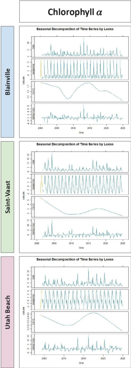
Figure 7: Seasonal Decomposition of Chlorophyll-a Concentrations (µg L⁻¹) from 2000 to 2024 at Blainville-sur-Mer, Saint-Vaast-la-Hougue, and Utah Beach.
