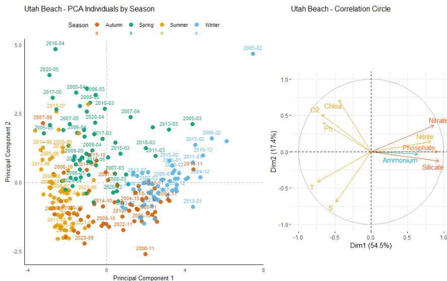
Figure 12: Principal Component Analysis of seasonal variability in physicochemical parameters and dissolved nutrients at Utah Beach. Left: Projection of sampling dates (2000–2024) on the first two principal components. Samples are colored by season: blue (winter), green (spring), yellow (summer), and orange (autumn). Right: Correlation circle showing the contribution of environmental variables: nutrients (nitrate, nitrite, ammonium, phosphate, silicate), dissolved oxygen (O 2 ), pH, chlorophyll a (Chlo a), temperature (T), salinity (S).
