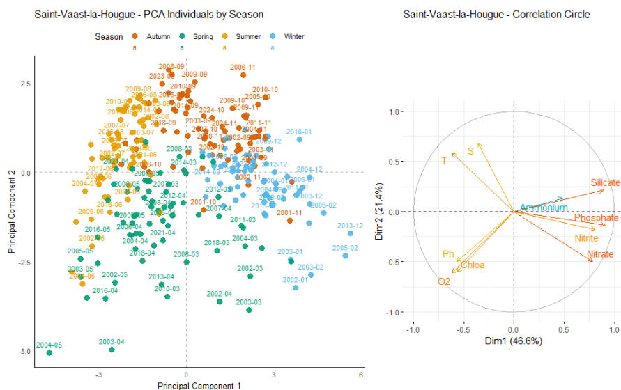
Figure 11: Principal Component Analysis of seasonal variability in physicochemical parameters and dissolved nutrients at Saint-Vaast-la-Hougue. Left: Projection of sampling dates (2000–2024) on the first two principal components. Samples are colored by season: blue (winter), green (spring), yellow (summer), and orange (autumn). Right: Correlation circle showing the contribution of environmental variables: nutrients (nitrate, nitrite, ammonium, phosphate, silicate), dissolved oxygen (O 2 ), pH, chlorophyll a (Chlo a), temperature (T), salinity (S).
