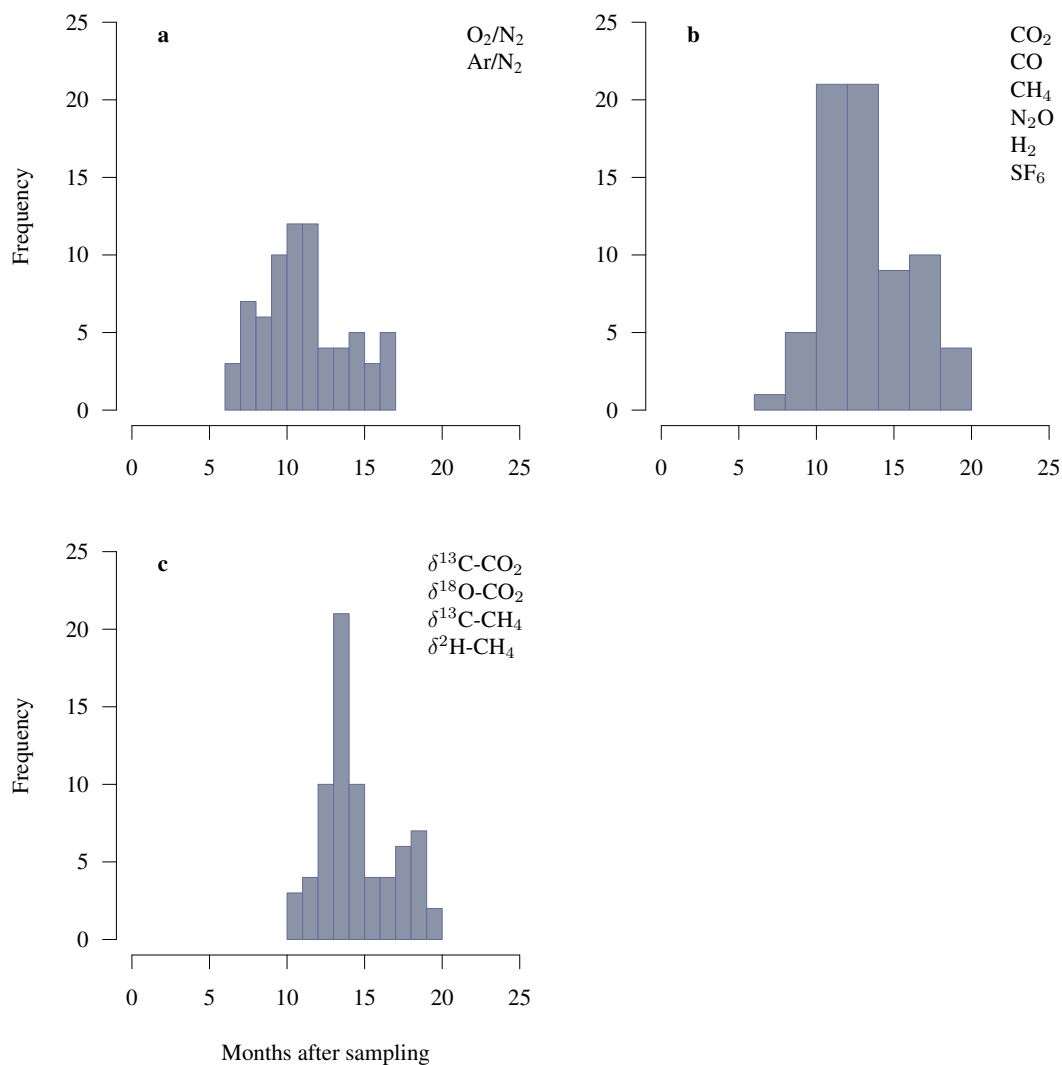
Figure 3. Frequency distributions of storage times of flasks in days months since sampling until laboratory analysis for (a) O 2 /N 2 and Ar/N 2 ratios, (b) GC measurements of trace gases, (c) IRMS measurements of stable isotopes.
