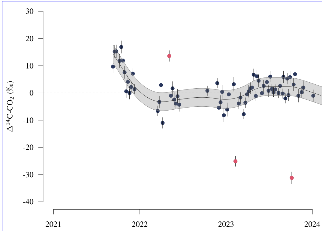
Figure 6. Radiocarbon in atmospheric carbon dioxide ( \Delta^{14}\text{C}-\text{CO}_2 ) measured in flasks at a height of 324 m agl at the Amazon Tall Tower Observatory. Error The line at the center of the gray area represents the smoothing cubic-splines fitted to all data points of individual species through an iterative process that removes outliers (red points) until all observations left are inside the range of three times the root mean squared deviation. The uncertainty range represented by the gray area represents the smoothing spline \pm the root mean squared deviation of the fitting. Vertical error bars, when visible, represent analytical-measurement uncertainty.
