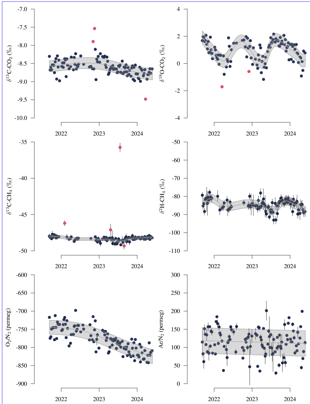
Figure 5. Gas species measured by mass spectrometry in flask samples from the Amazon Tall Tower Observatory. Lines represent the line at the center of the gray area represents the smoothing cubic-splines-cubic-splines fitted to all data points of individual species through an iterative process that removes outliers (red points) until all observations left are inside the range of three times the root mean square error squared deviation. Outliers, The uncertainty range represented as red points, are not reliable observations for determining background conditions at by the local level gray area represents the smoothing spline \pm the root mean squared deviation of the fitting. Error Vertical error bars, when visible, represent analytical-measurement uncertainty.
