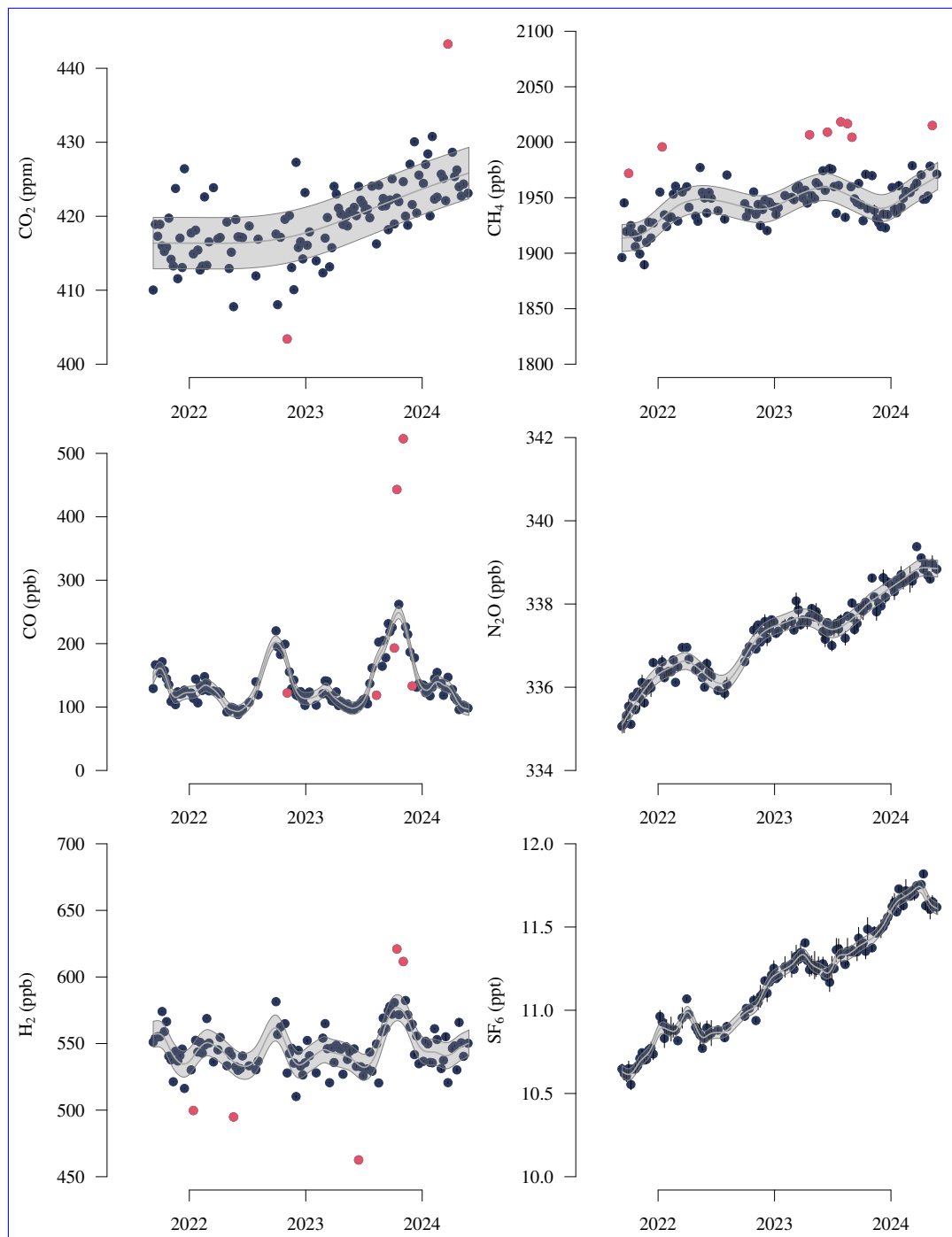
Figure 4. Gas species measured by gas chromatography in flask samples from the Amazon Tall Tower Observatory. Lines represent The line at the center of the gray area represents the smoothing cubic-splines fitted to all data points of individual species through an iterative process that removes outliers ( red points ) until all observations left are inside the range of three times the root mean squared deviation. Outliers- The uncertainty range represented as red points, are not reliable observations for determining background conditions at by the local level gray area represents the smoothing spline \pm the root mean squared deviation of the fitting. Error- Vertical error bars, when visible, represent analytical measurement uncertainty.
