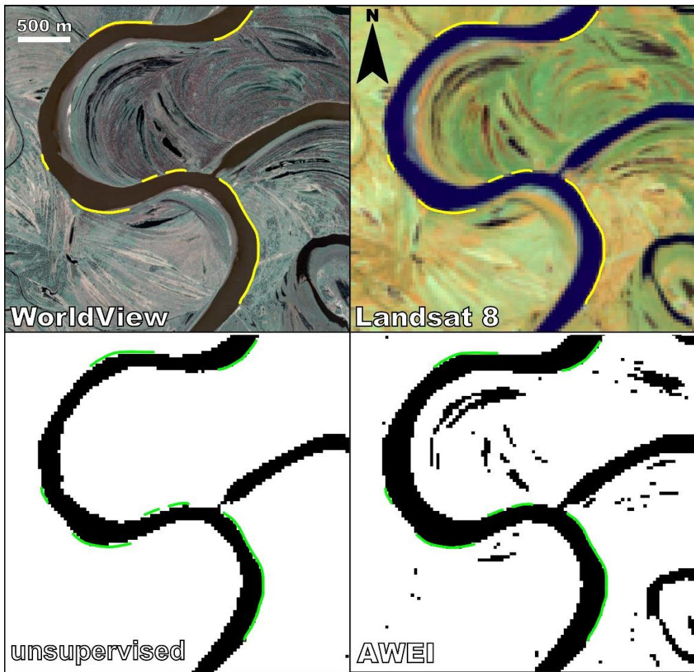
375 Fig. 6. Yana River section near Batagay settlement on satellite images from June 21, 2021 with digitized position of the riverbanks 380 in the erosion area (top, yellow lines) and an example of their automatic detection by automatic classification (bottom left) and with application of the AWEI index (bottom right) with manual digitized bank positions imposed (green lines).
