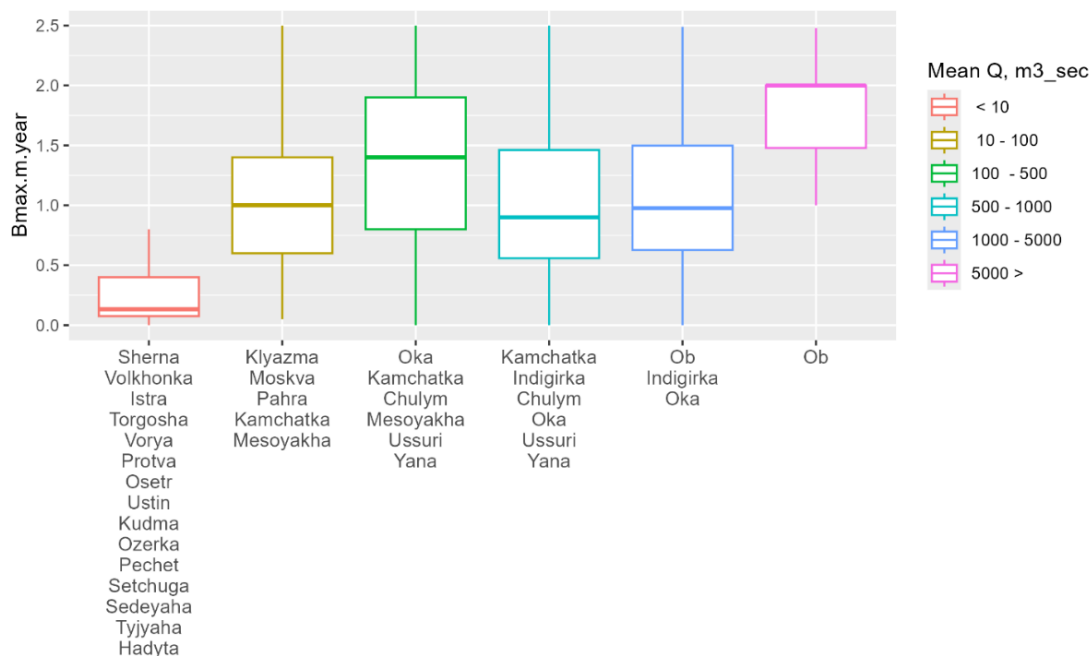
530 Fig. 12. Boxplot of site-averaged bank retreat rates with respect to river size (annual discharge Q [m³/s])
