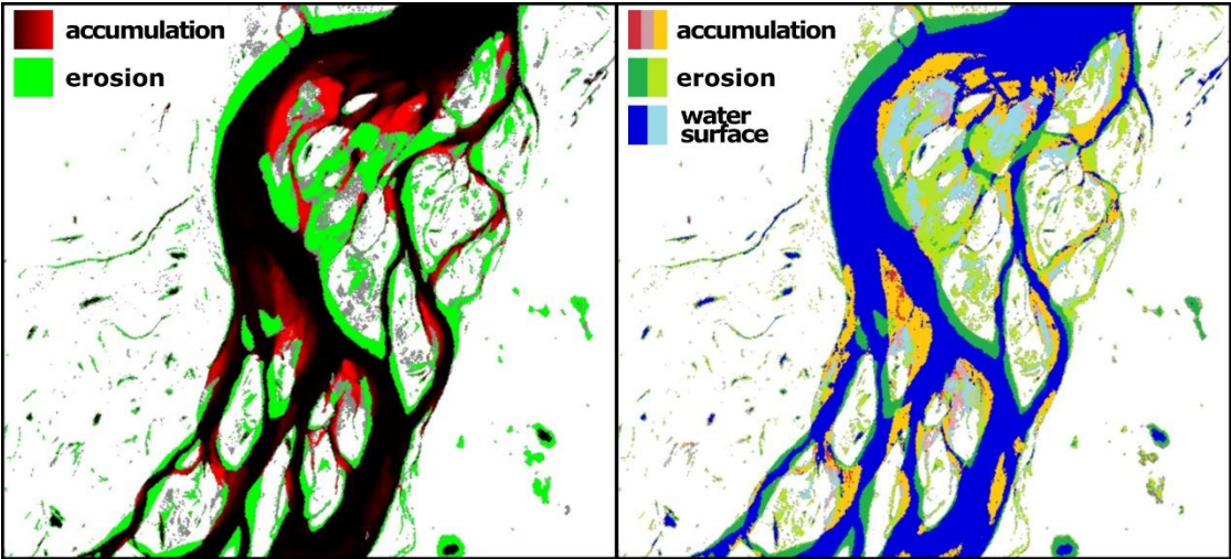
Fig. 5. Bank erosion classification according to GSWE map – change intensity (left) and transitions (right) (Lena River case study) Explanations: change intensity layer classify water surface from Landsat imagery collection into three types – stable water surface, erosion and accumulation areas (accumulation color is more saturated for more permanent areas over time). Transition 320 layers classify water surface more detailed according to seasonality, which allow to separate erosion and accumulation for stable banks and shoals, sandbanks etc.
