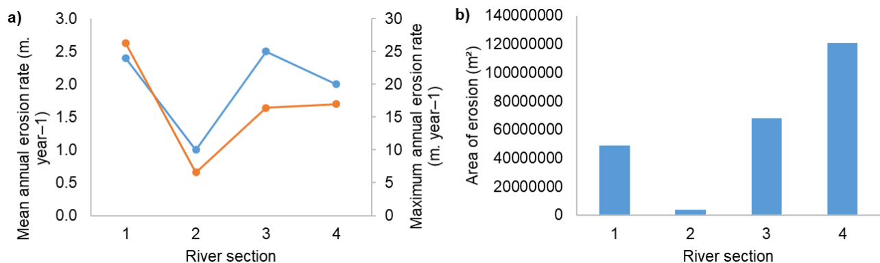
545 Fig. 13. Riverbank erosion of the Ob River: a – erosion rate, b – area of erosion. 1 – Upstream Ob River, 2 – Middle stream of Ob River (from the Novosibirsk reservoir to the confluence of the Ob River and the Tom River), 3 – Middle stream Ob River (from the confluence of the Ob River and the Vakh River to the confluence of the Ob River and the Irtysh River), 4 – Downstream Ob River (from the confluence of the Ob River and the Irtysh River to the city of Salekhard)
