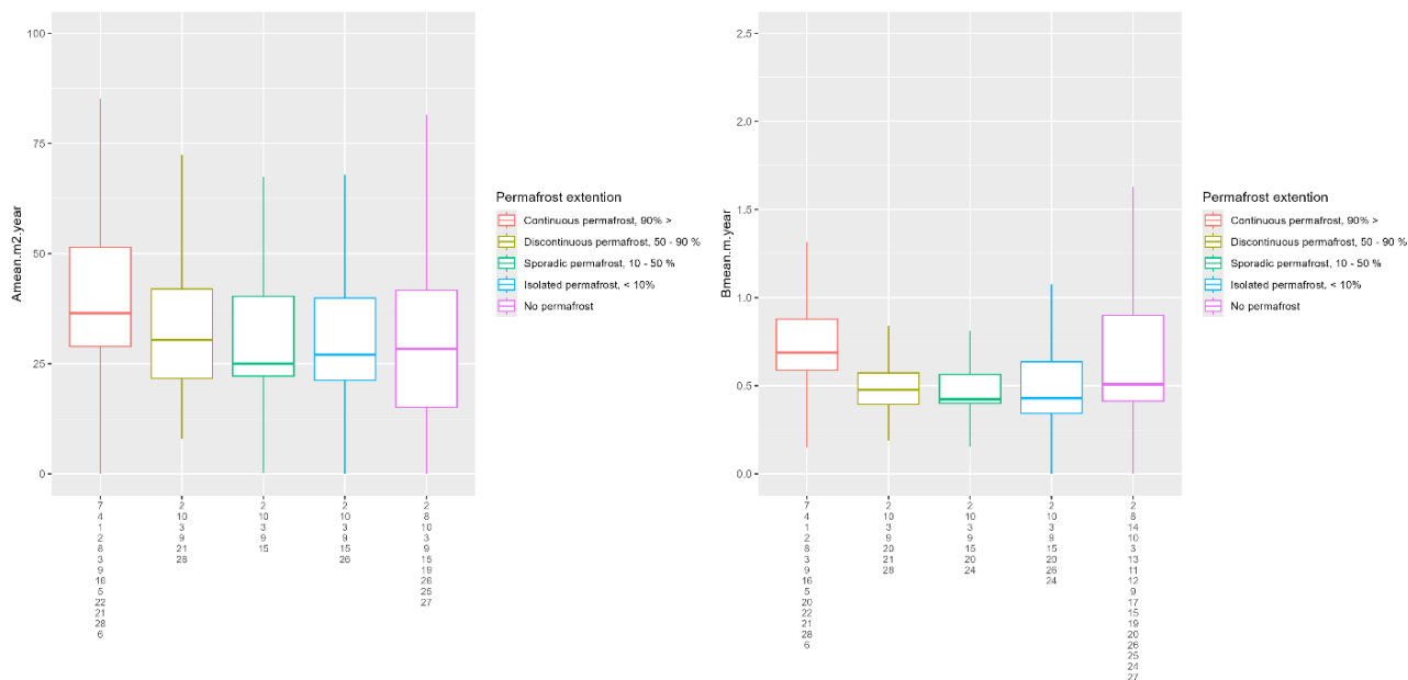
Fig. 15. Boxplot of site-averaged bank retreat rates with respect to permafrost (left – bank areas destroyed by bank erosion; right – average rates of bank erosion)
