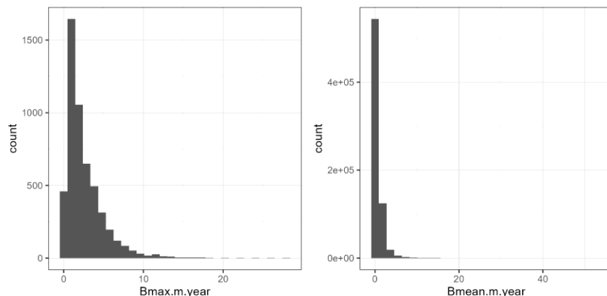
Fig. 9. Distribution of observed riverbank erosion rates in Northern Eurasia (left – maximal bank retreat B [m/year]; right – annual bank retreat B [m/year])
