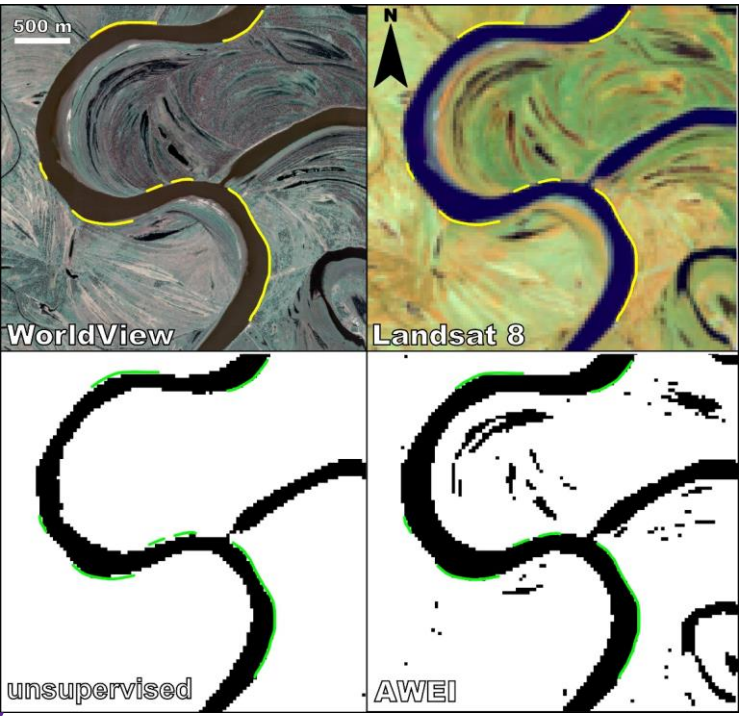
Fig. 6. Yana River section near Batagay settlement on satellite images from June 21, 2021 with digitized position of the riverbanks in the erosion area (top, yellow lines ) and an example of their automatic detection by automatic classification (bottom left) and with application of the AWEI index (bottom right) with manual digitized bank positions imposed (green lines) .
