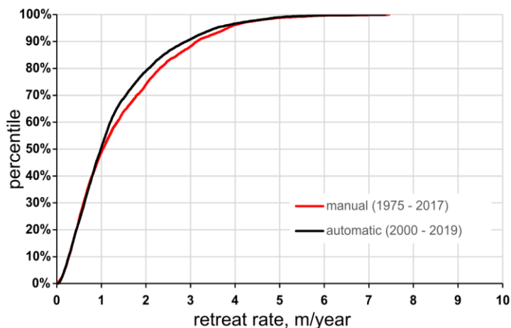
Fig. 7. Percentile curves of the retreat rates for manual and semi-automatic delineation of banks on the similar section of the Indigirka River.
