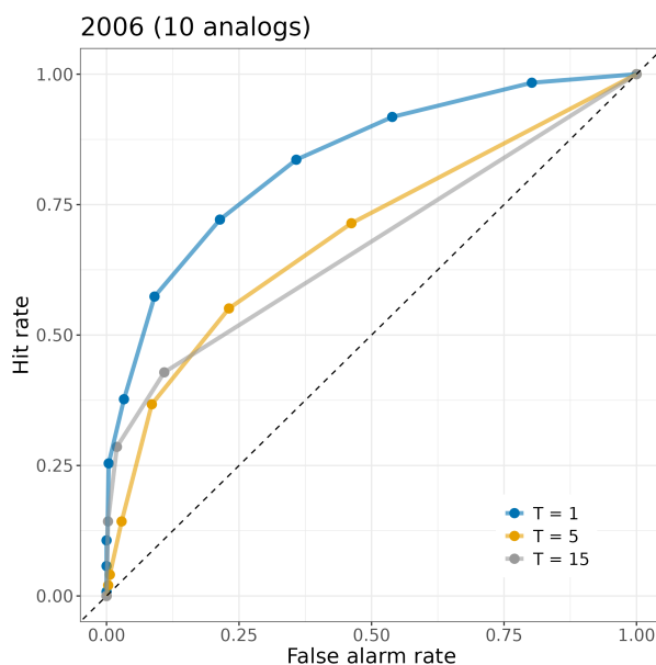
Figure 9. Examples of ROC curves for common and rare events. ROC curves and corresponding AUCs for precipitation forecasts with event thresholds: 1 mm, 5 mm, and 15 mm per 24h (2006, 10-member ensemble).
