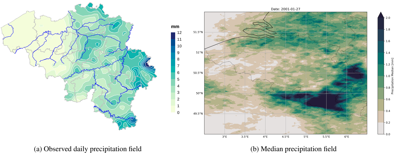
Figure 15. Comparison of observed daily precipitation accumulation and the median accumulation derived from the 25 best analog days.
