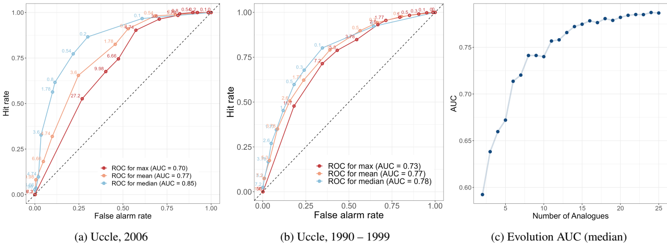
Figure 8. From left to right: (a) ROC curve for Uccle for 2006 for models based on different summary statistics using the 10 best analogs; (b) ROC curve for Uccle for the period 1990 - 1999 for models based on different summary statistics using the 10 best analogs; (c) The evolution of AUC values in relation to the increasing number of analog days per target day in 1990-1999, using the median as the predictive measure.
