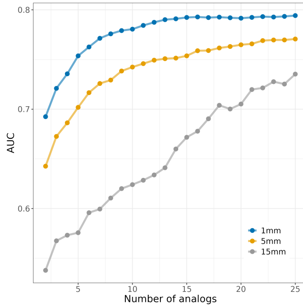
Figure 12. Evolution of AUC values based on the median with increasing number of ensemble members for the three considered event thresholds 1 mm, 5 mm and 15 mm per 24h for the 10-year period 1990 – 1999.
