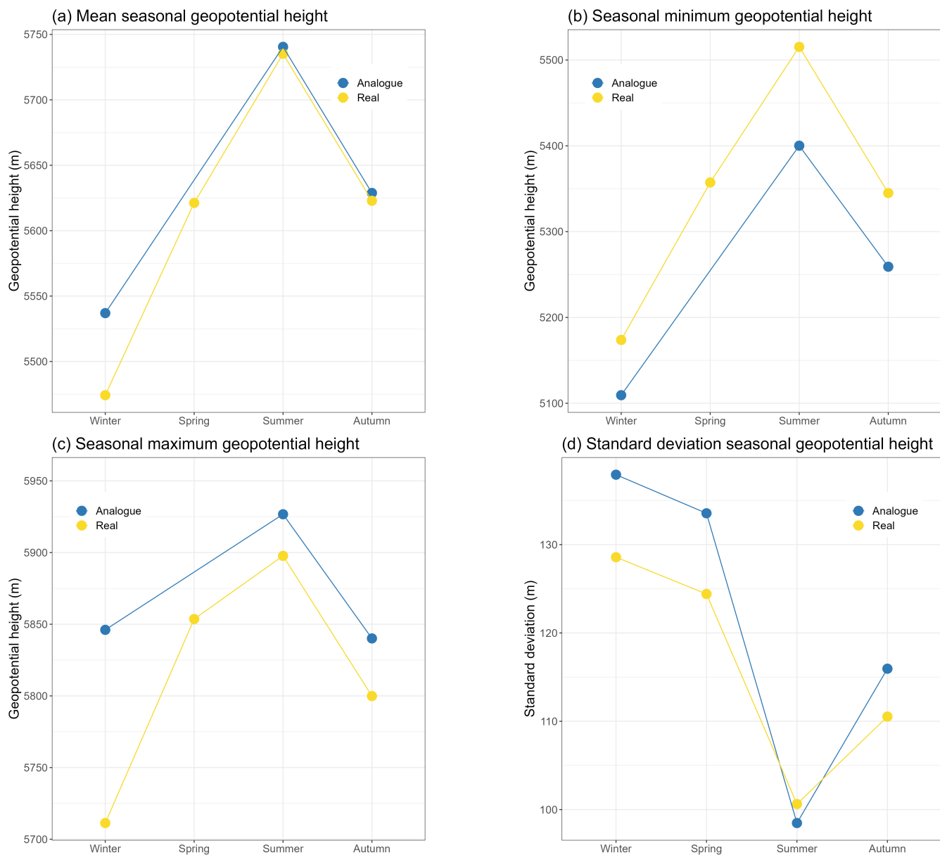
Figure 6. Seasonal statistics of geopotential height at 500 hPa in Uccle at 12UT in 2006. Top left to bottom right: (a) mean, (b) minimum, (c) maximum and (d) standard deviation. The general pattern seems similar in the different cases.
