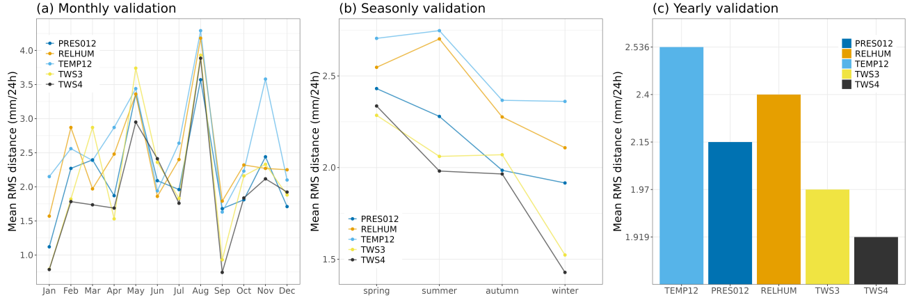
Figure 3. Monthly (a), seasonally (b) and yearly (c) performance of the different predictor sets. The five methods under consideration were assessed on a monthly, seasonal, and annual basis. For each predictor set, the mean RMSE (in mm/24h) was computed for each time period (month, season, and year). The average of these summary statistics serves as an indicator of the overall performance of each predictor set. As showed in all three figures, it is clear at a glance that the TWS3 and TWS4 methods exhibit superior performance compared to RELHUM and TEMP12.
