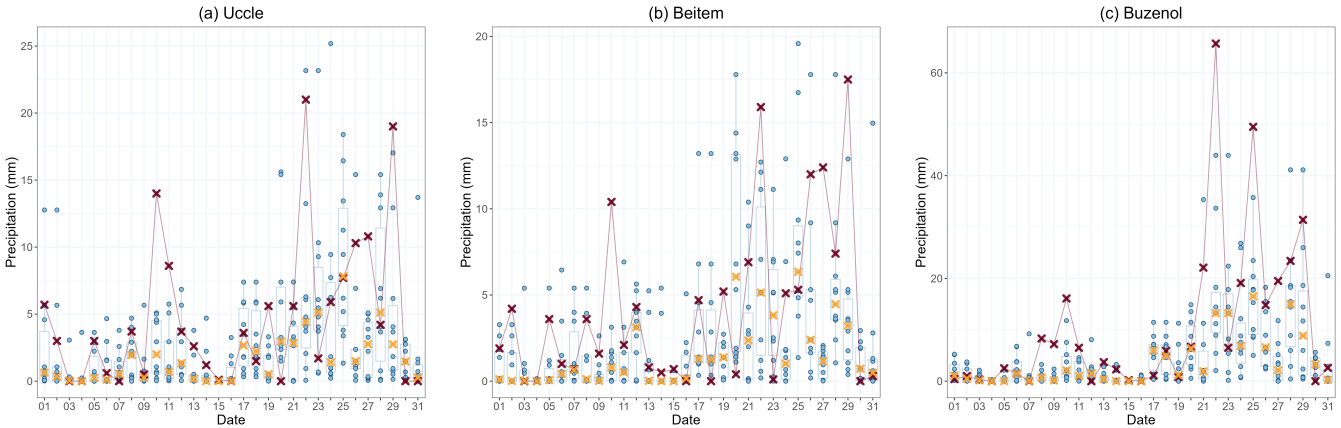
Figure 13. Daily precipitation accumulation patterns (distributions) for January 1995 using the ten most similar analog days using radar values indicated by the blue dots. The daily observations obtained from the pluviometer in (a) Uccle, (b) Beitem and (c) Buzenol indicated by the purple markers. The yellow crosses represent the median precipitation value for each day based on these 10 best analog days.
