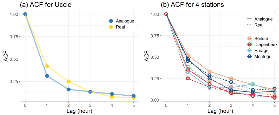
Figure 14. (a) Autocorrelation Function (ACF) for hourly data from Uccle in 2006, comparing real hourly AWS data with median hourly radar data based on the 10 best analogs in Uccle in 2006. (b) ACF for hourly data from Beitem, Mont Rigi, Ernage en Diepenbeek in 2006 on real and best analog days using lag period of 5.
