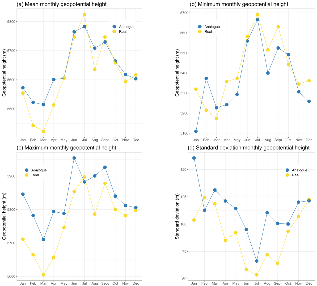
Figure 5. Monthly statistics of geopotential height at 500 hPa pressure level in Uccle at 12 UT in 2006. Top left to bottom right: (a) mean, (b) minimum, (c) maximum and (d) standard deviation. The general pattern between real and analog days seems similar across all four summary measures.
