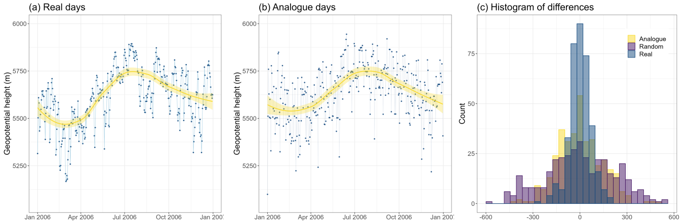
Figure 4. The temporal evolution in geopotential height at the 500 hPa pressure level at 12 UT in Uccle in 2006 (panel a); the corresponding data on the best analog days in 2006 (panel b); differences in geopotential height on analog days, real days and random days (panel c). The yellow curves in the first two plots aid the eye in seeing patterns in the presence of overplotting by fitting a smooth curve to the data.
