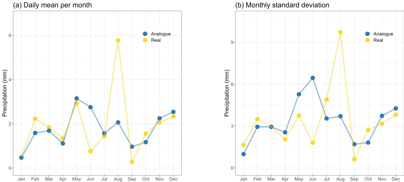
Figure 7. Evolution of (a) daily mean per month and (b) monthly standard deviation of 24h precipitation accumulation in Uccle in 2006.
