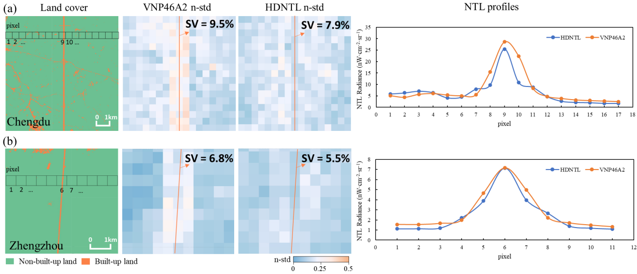
385 Figure 5: Spatial mismatch correction effectiveness in less-angular effect areas within highway cases. (a) Chengdu Tianfu Avenue, (b) Zhengzhou section of Beijing-Hong Kong-Macao Expressway. Land cover data from the European Space Agency (ESA) WorldCover 10 m 2020 product © ESA WorldCover Consortium.
