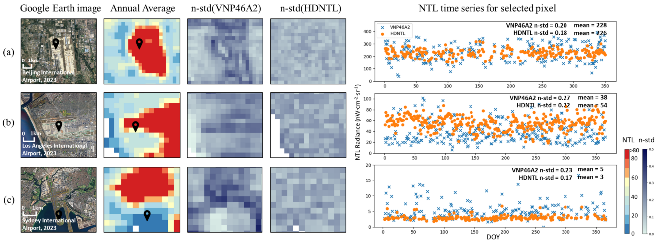
370 Figure 4: Spatial mismatch correction effectiveness in less-angular effect areas within airport cases. (a) Beijing International Airport, (b) Los Angeles International Airport, (c) Sydney International Airport. Google Earth images © 2025 Google LLC.
