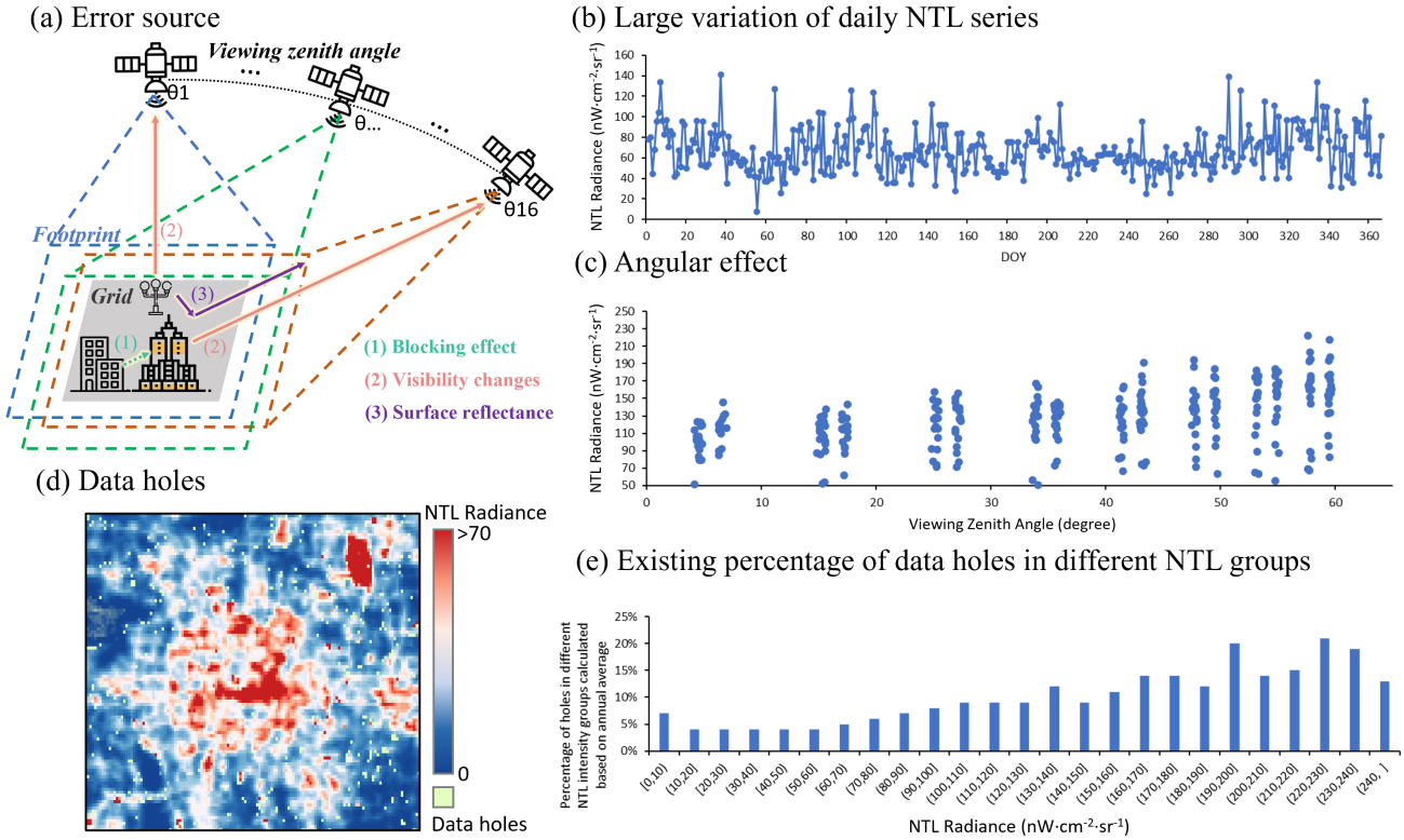
95 Figure 1: An illustration of spatial mismatch error, angular effect error and data holes of VNP46A2. (a) Error source: Schematic diagram illustrating the existence of spatial mismatch and angular effects, (b) The instability of daily NTL series, (c) Angular effect: The changing trend of daily NTL intensity along with VZA changes within one year, (d) Data holes existence in cloud-free NTL image of Beijing on October 1, 2018, (e) The percentage of data holes in different NTL intensity groups calculated based on annual averages.
