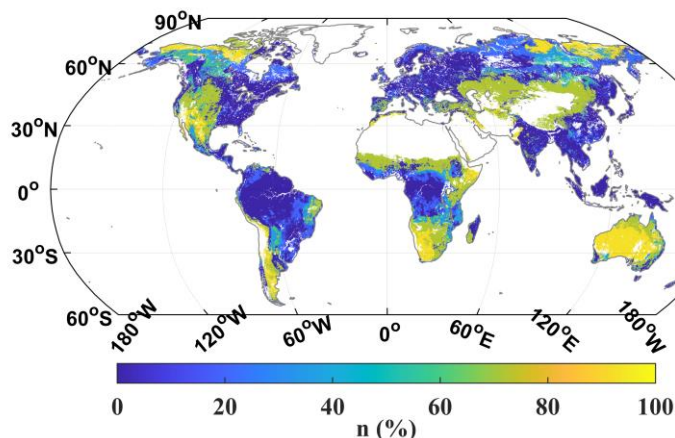
Figure 5: Global map of the parameter n on vegetation areas covering 9 land cover types.
