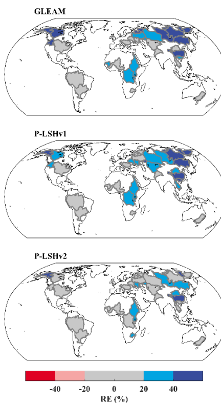
475 Figure 13: Spatial patterns of relative deviations of multiyear average ET from three remote sensing datasets on 32 global large basins.
