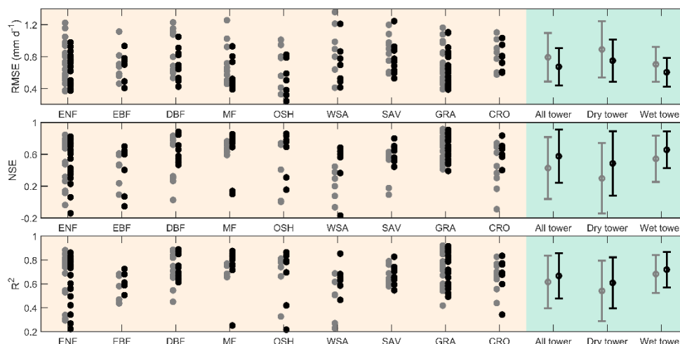
370 Figure 7: Comparison of ET estimations from the P-LSHv2 algorithm (black circles) and the P-LSHv1 algorithm (gray circles) at 106 flux towers. Each circle represents a flux tower and the classified statistical values are plotted in the right panels. RMSE: root mean square error; NSE: Nash-Sutcliffe efficiency coefficient; R 2 : coefficient of determination.
