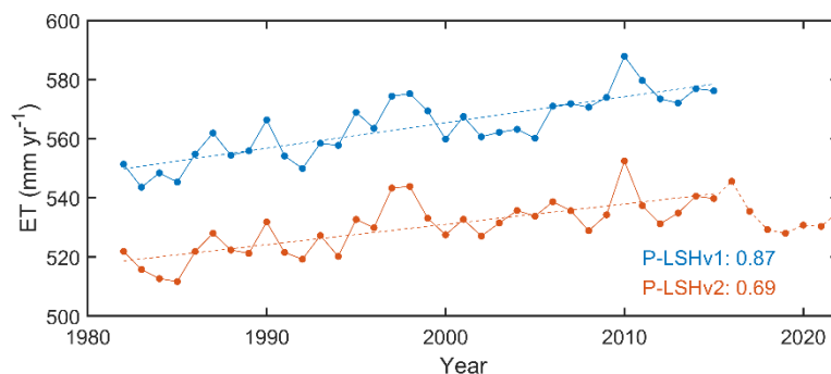
500 Figure 15: Annual global ET estimates derived from P-LSHv1 and P-LSHv2.
