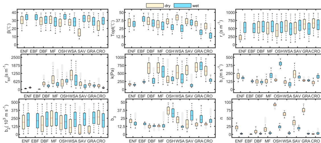
320 Figure 4: Boxplots of the parameter posterior distributions with 95% high probability across diverse land cover types and climate zones. The red line represents the median and the gray dots represent outliers.
