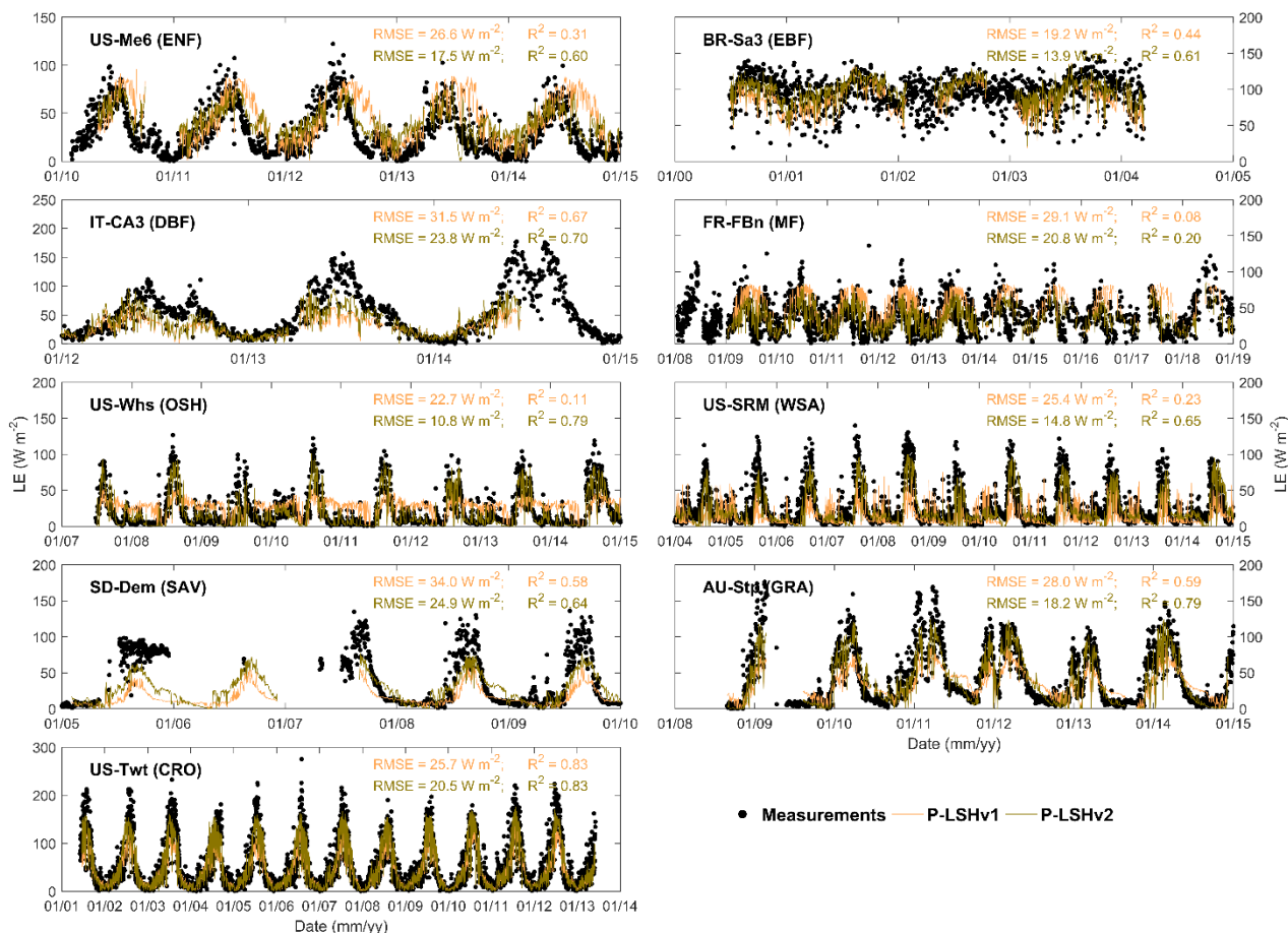
Figure 8: Time series of daily measured and modelled latent heat flux (LE: W m -2 ) using the P-LSHv2 and P-LSHv1 algorithms for typical dry towers.
