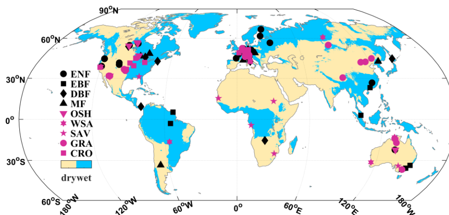
235 Figure 2: Locations of 106 flux towers used for ET algorithm development and validation. The symbols represent land cover types and colored backgrounds represent climate zones.
