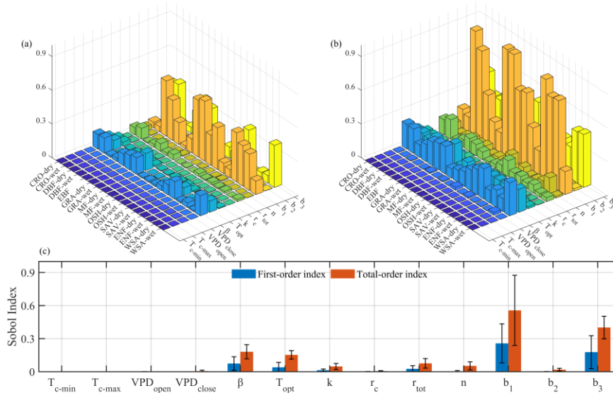
310 Figure 3: The (a) first-order sensitivity index and (b) total-order sensitivity index of the parameters across diverse land cover types and climate zones. The average values of diverse zones are shown in (c).
