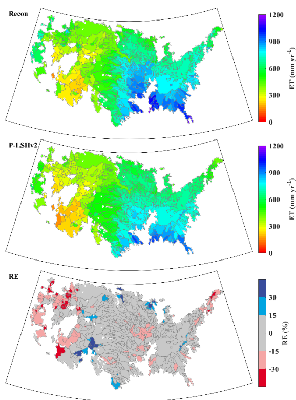
445 Figure 11: Spatial patterns of multiyear average ET from ET_{\text{recon}} and P-LSHv2 and their difference (RE) on 592 basins of CONUS.
