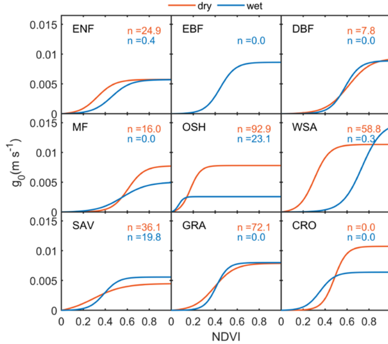
370 Figure 6: The sigmoid-type response curve between g_0 and NDVI. The colors represent climate zones and n is the parameter to control soil moisture constraints.
