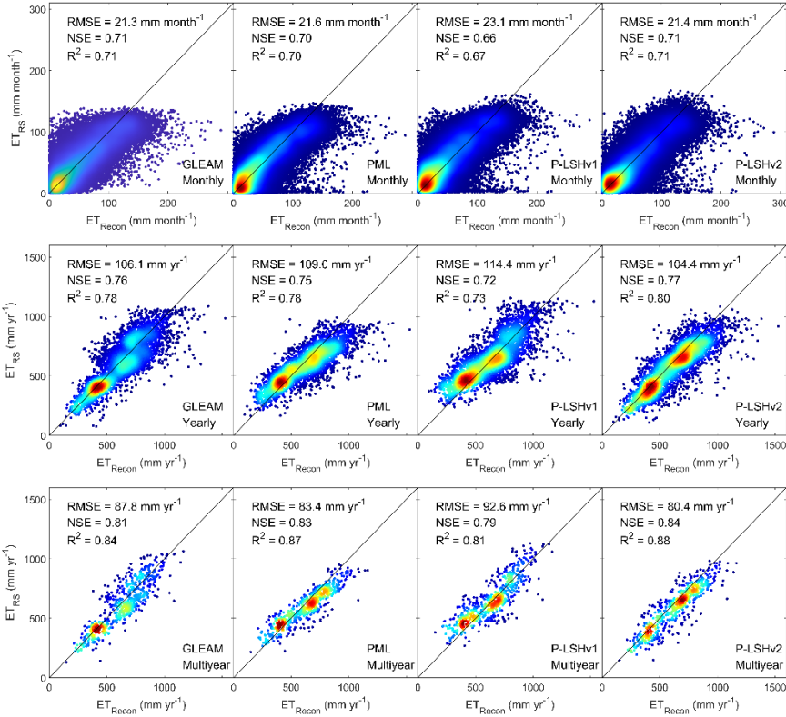
Figure 10: Comparison of monthly, yearly, and multiyear average ET derived from four remote sensing datasets (ET RS ) and ET recon on 592 basins of CONUS. Colors are used to represent density, with red representing high density and blue representing low density.
