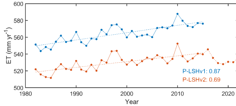
515 Figure 15: Annual global ET estimates derived from P-LSHv1 and P-LSHv2.
