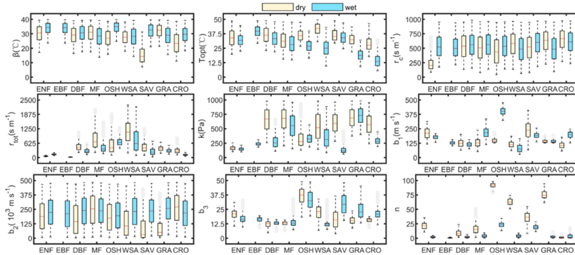
Figure 4: Boxplots of the parameter posterior distributions with 95% high probability across diverse land cover types and climate zones. The red line represents the median and the gray dots represent outliers.
