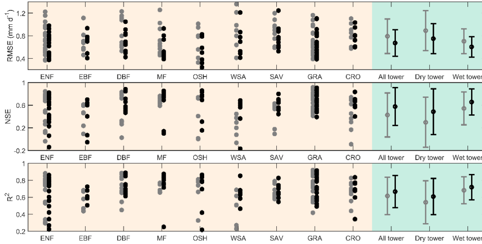
385 Figure 7: Comparison of ET estimations from the P-LSHv2 algorithm (black circles) and the P-LSHv1 algorithm (gray circles) at 106 flux towers. Each circle represents a flux tower and the classified statistical values are plotted in the right panels. RMSE: root mean square error; NSE: Nash-Sutcliffe efficiency coefficient; R^2 : coefficient of determination.
