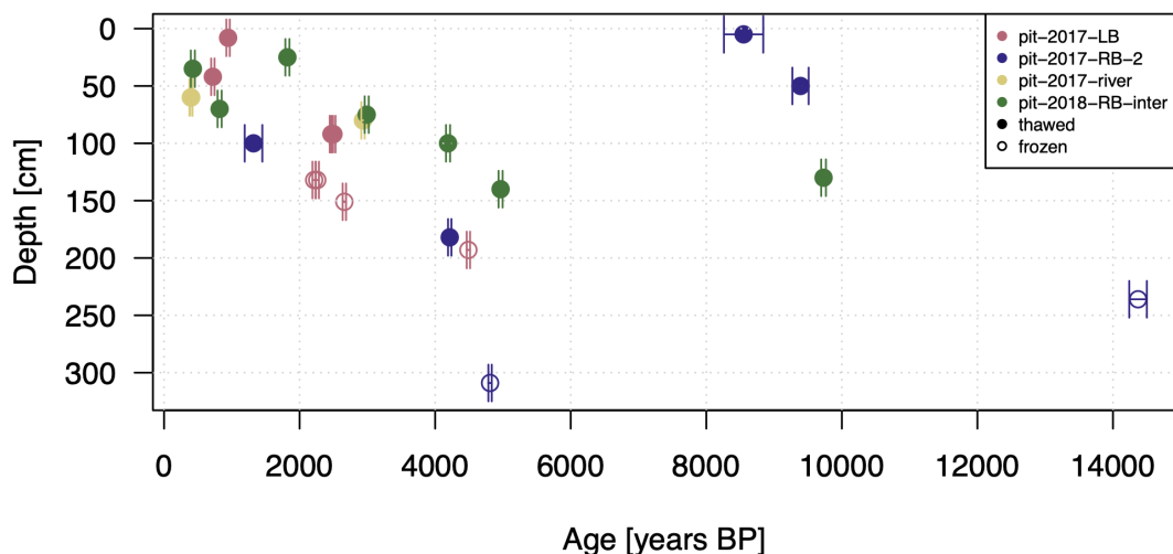
Figure 11. Radiocarbon dating ( ^{14}\text{C} ) at Site 2. Ages are derived from F^{14}\text{C} using the conversion of Stuiver and Polach (1977)(see main text). Error bars represent \pm 1 standard deviation, calculated by first-order propagation of uncertainties through the logarithmic age transformation. Frozen samples likely represent permafrost; however, this interpretation is based on measured thaw depths rather than verified active layer depths (see Section,4.1.3).
