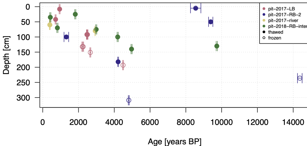
Figure 11. Radiocarbon dating ( ^{14}\text{C} ) at Site 2. Error bars represent \pm 1 standard deviation.
