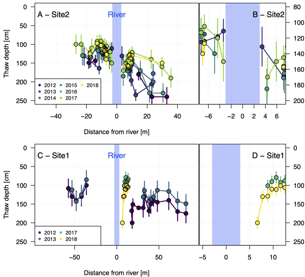
Figure 6. Thaw depths in the active layer at two cross-sections at the two main locations Site 2 (A) and Site 1 (C) with zoomed-in detail views (B and D, respectively). Error bars represent unverified assessment of measurement errors of different techniques as explained in the text. Date of measurement for individual years varied - information is contained in the data files and in the geopackage files of the GIS database.
