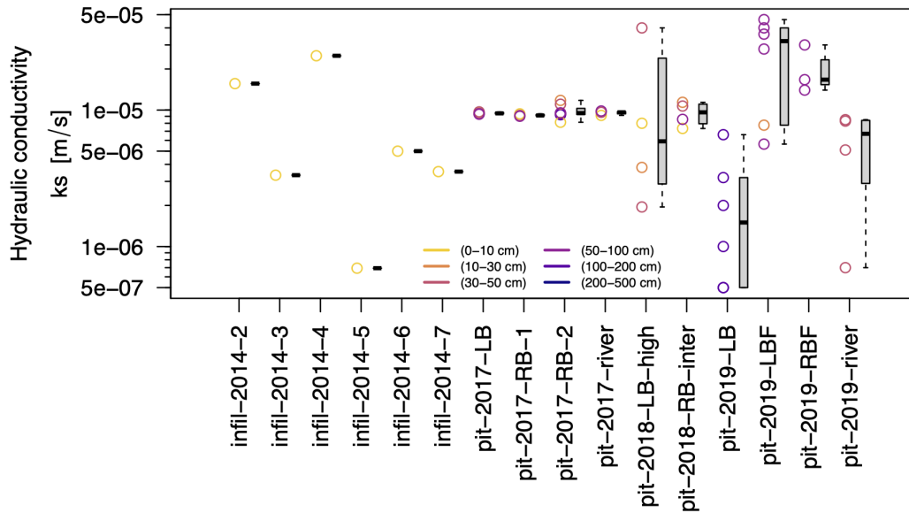
Figure 9. Hydraulic conductivity estimates determined by infiltration tests and laboratory analysis of grain size distributions using the Rosetta3 algorithm (Zhang and Schaap, 2017), at the surface and various depths within soil pits.
