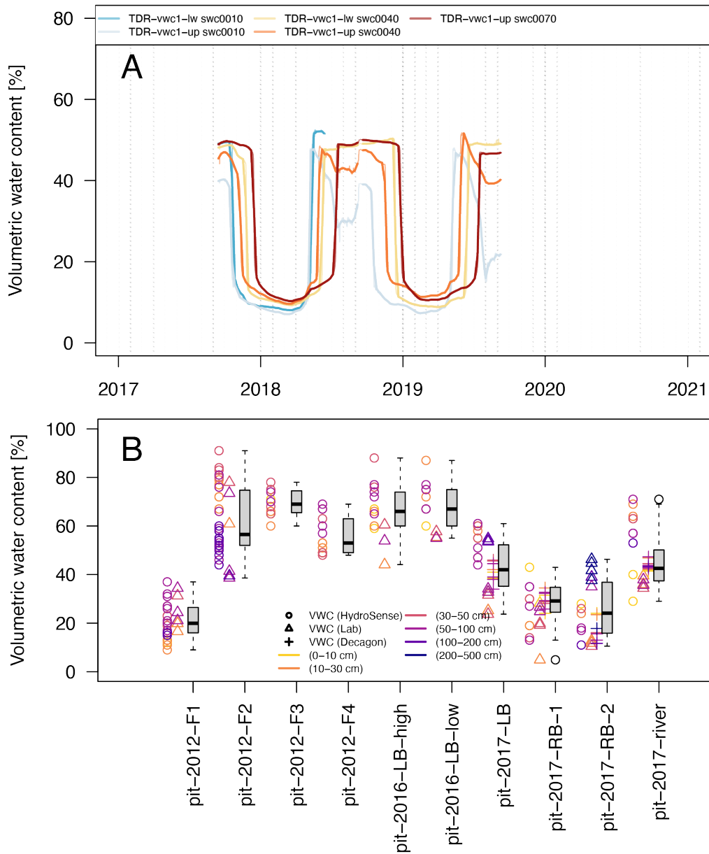
Figure 7. Soil water content measurement time-series using EC-5 probes from Decagon (A), and individual tests made in soil pits or from soil samples analysed analyzed in the field and the laboratory using multiple instruments (B).
