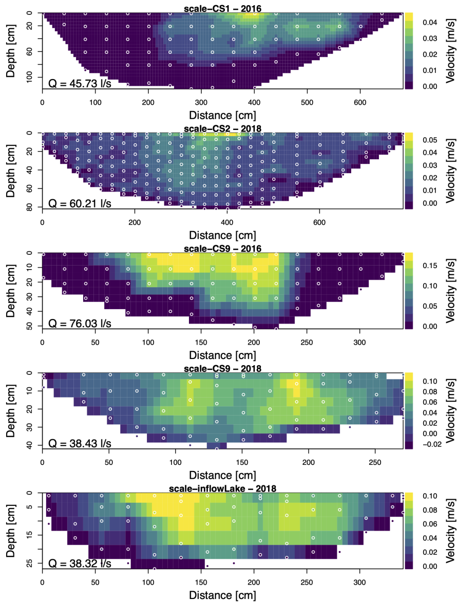
Figure 16. Water velocities at different cross-sections and years. White-circled points represent point-wise measurements made with an electromagnetic current profiler. The regular grid is produced by linear interpolation to a regular grid size resolution of 5 cm. The script to calculate the discharge ("auxiliary/scripts") allows to set different interpolation resolutions.
