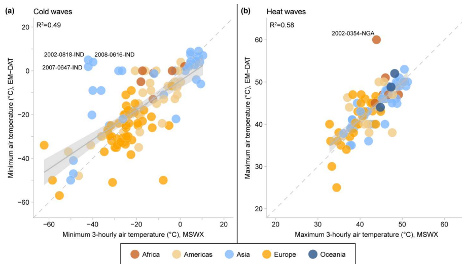
2 Figure 98 Comparison of extreme temperatures between EM-DAT and MSWX. The scatter plots illustrate the relationship between 4 reported temperature extremes in EM-DAT and the corresponding 3-hourly minimum (a) and maximum (b) temperatures from MSWX for 120 cold waves and 94 heat waves, respectively. Each point represents a disno, with colours indicating the continent.
