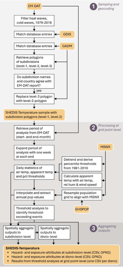
4 Figure 2. Flowchart illustrating the main steps of integrating data from multiple sources to derive SHEDIS-Temperature. (1) A total 6 of 382 temperature-related impact records from EM-DAT were successfully matched to subnational locations by GDIS, which we used to identify 2,835 subdivision boundaries at level 1 (province/equivalent) and level 2 (county/district/equivalent) from GADM. (2) Within these identified geographical extents, daily statistics of meteorological variables (absolute values and percentiles) were computed from MSWX.
