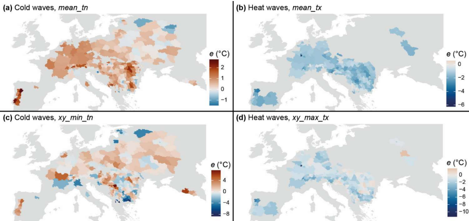
Figure B13 Spatial distribution of administrative level 1 subdivisions included in the technical validation against the E-OBS dataset. Colours indicate the error e as defined in Eq. (5), where positive values represent overestimation by MSWX relative to E-OBS. Some subdivisions are associated with multiple records per hazard type, for which mean e values are shown. Only level 1-units are visualized to avoid spatial overlap and because they constitute the majority of the sample, although level 2-units were also included in the validation analysis.
