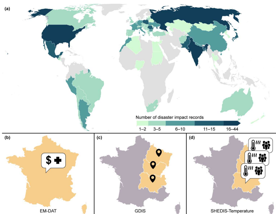
Figure 1 Introduction to SHEDIS-Temperature. (a) The 382 national-level disaster records from 1979 to 2018 in 71 countries that underpin the dataset. These records comprise EM-DAT records (b) that have been geocoded to administrative subdivisions by GDIS (c). SHEDIS-Temperature expands on this by providing an extensive catalogue of hazard- and exposure-related attributes for each subdivision and disno (d), as well as data on grid point level.
