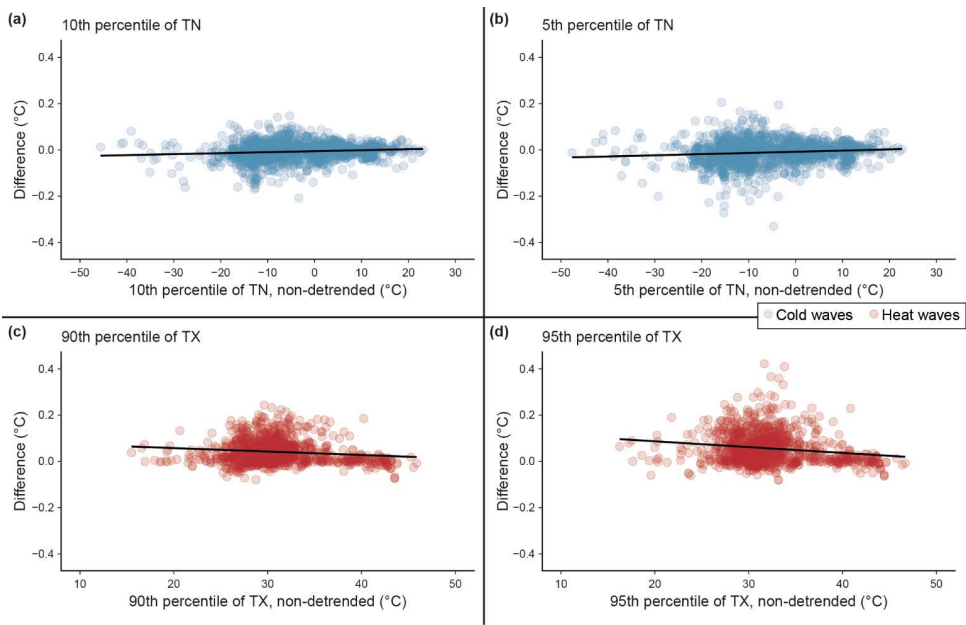
6 Figure C1 Scatter plots of percentile differences (°C) across temperature levels. Panels (a) and (b) illustrate percentiles used for cold wave records (pct10 and pct05 from TN), and panels (c) and (d) show for heat-wave records (pct90 and pct95 from TX). Each dot represents a SHEDIS-Temperature record at the subdivision level, with percentile values averaged across its spatiotemporal domain. Differences are defined as percentile values from the non-detrended time series minus those from the detrended time series. Black lines denote linear trend fits.
