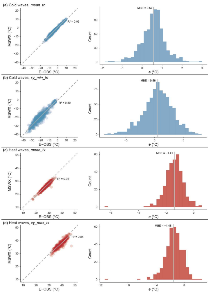
2 Figure 8 Validation of MSWX against E-OBS for extreme daily temperatures. Panels (a) and (b) represent minimum temperature 4 agreement for cold wave records, and panels (c) and (d) show maximum temperatures for heat wave records (covered by the E-OBS grid). Scatter plots illustrate agreement between the datasets, and histograms show the distribution of errors. Each dot in the scatter plots represents a subdivision-level record. The variables mean_tn and mean_tx represent spatiotemporally averaged values across each record's domain.
