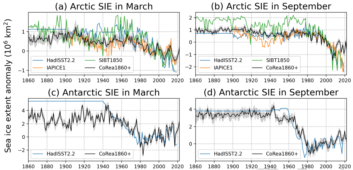
Figure 5. Time series of the anomalies of SIE in the Arctic (a, b) and Antarctic (c, d) in March (a, c) and September (b, d). The anomaly refers to the climatology from 1980 to 2017. Note that IAPICE1 and SIBT1850 provide sea ice data only in the Northern Hemisphere.
