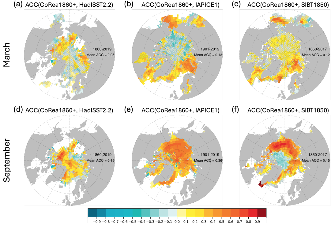
Figure R4: ACC of Arctic sea ice concentration in March or September of CoRea1860+ against HadISST2.2, IAPICE1, and SIBT1850. Grids that fail the significance test are marked with a slash. The period used to compute ACC corresponds to the overlapping period between CoRea1860+ and the specific reference dataset and is shown in Eurasia. The spatially averaged ACC is also shown in Eurasia.
