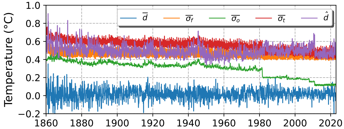
Figure R1: Global assimilation diagnostics for the assimilated variable – monthly SST anomalies: bias (blue line), background error (orange line), observation error (green line), total error (red line), and RMSE (purple line).
