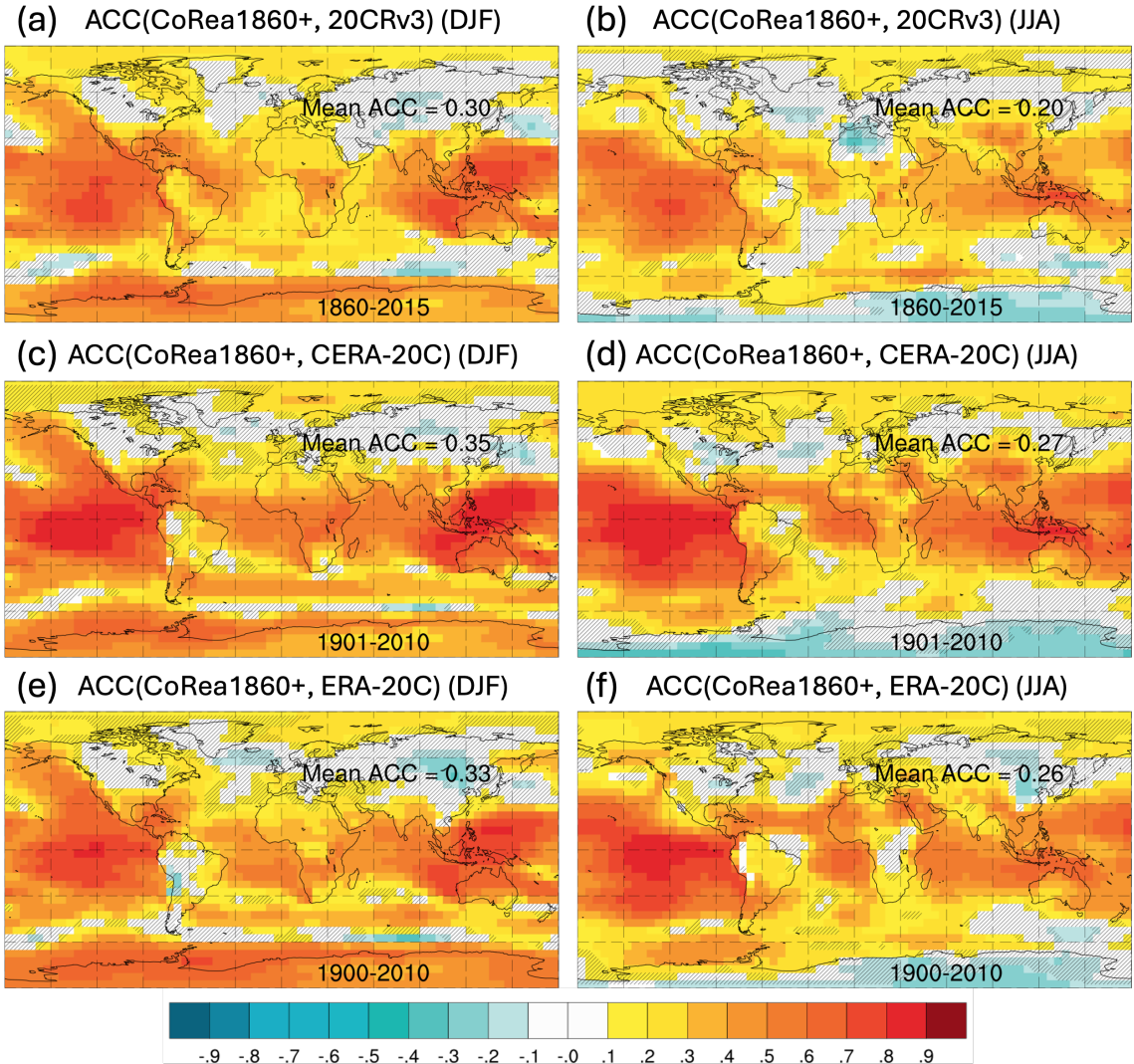
Figure R7: ACC of SLP in DJF or JJA of CoRea1860+ against 20CRv3, CERA-20C and ERA-20C. Grids that fail the significance test are marked with a slash. The period used to compute ACC corresponds to the overlapping period between CoRea1860+ and the specific reference dataset and is shown in Antarctica. The spatially averaged ACC is shown in Eurasia.
