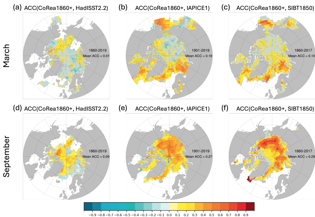
Figure R5: Same as Figure R4 but for detrended timeseries.
