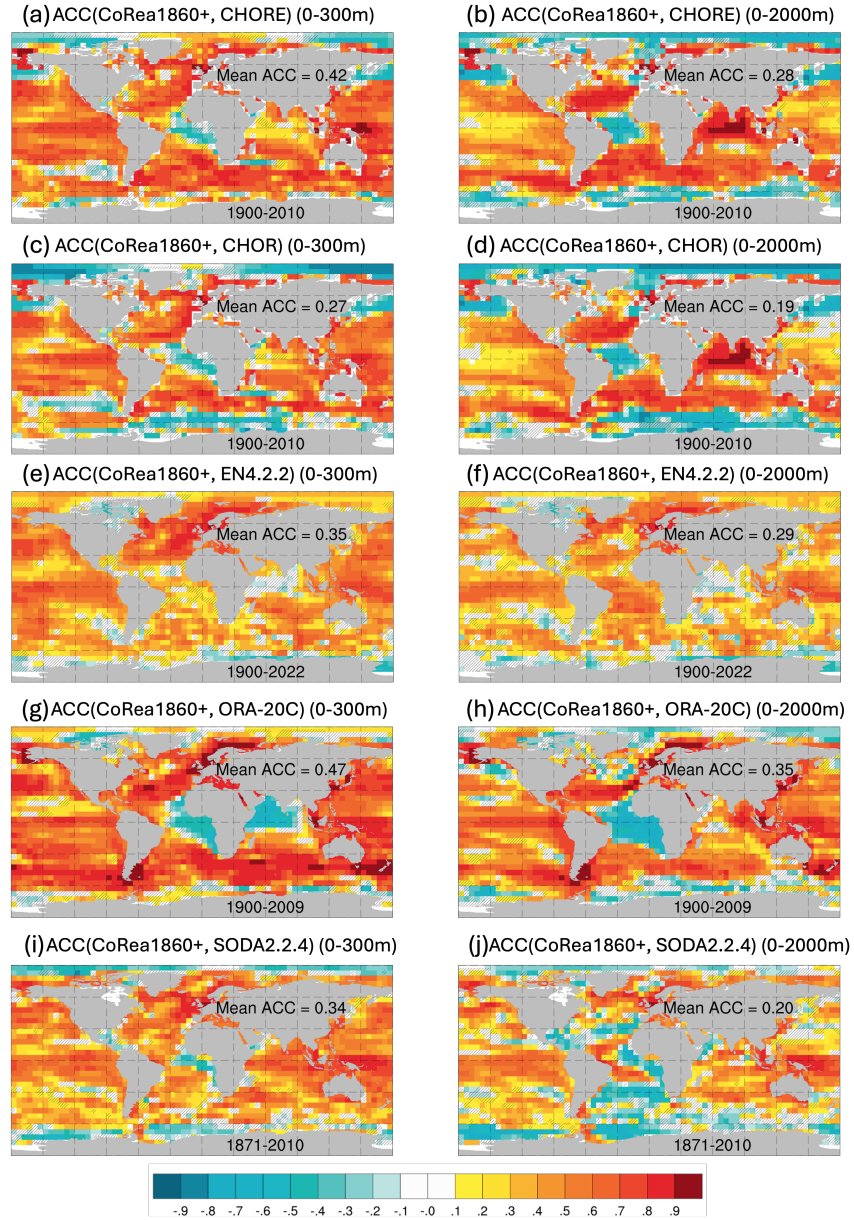
Figure R2: ACC of yearly OHC in 0-300m or 0-2000m of CoRea1860+ against different reference datasets. Grids that fail the significance test are marked with a slash. The period used to compute ACC corresponds to the overlapping period between CoRea1860+ and the specific reference dataset and is shown in Antarctica. The spatially averaged ACC is shown in Eurasia.
