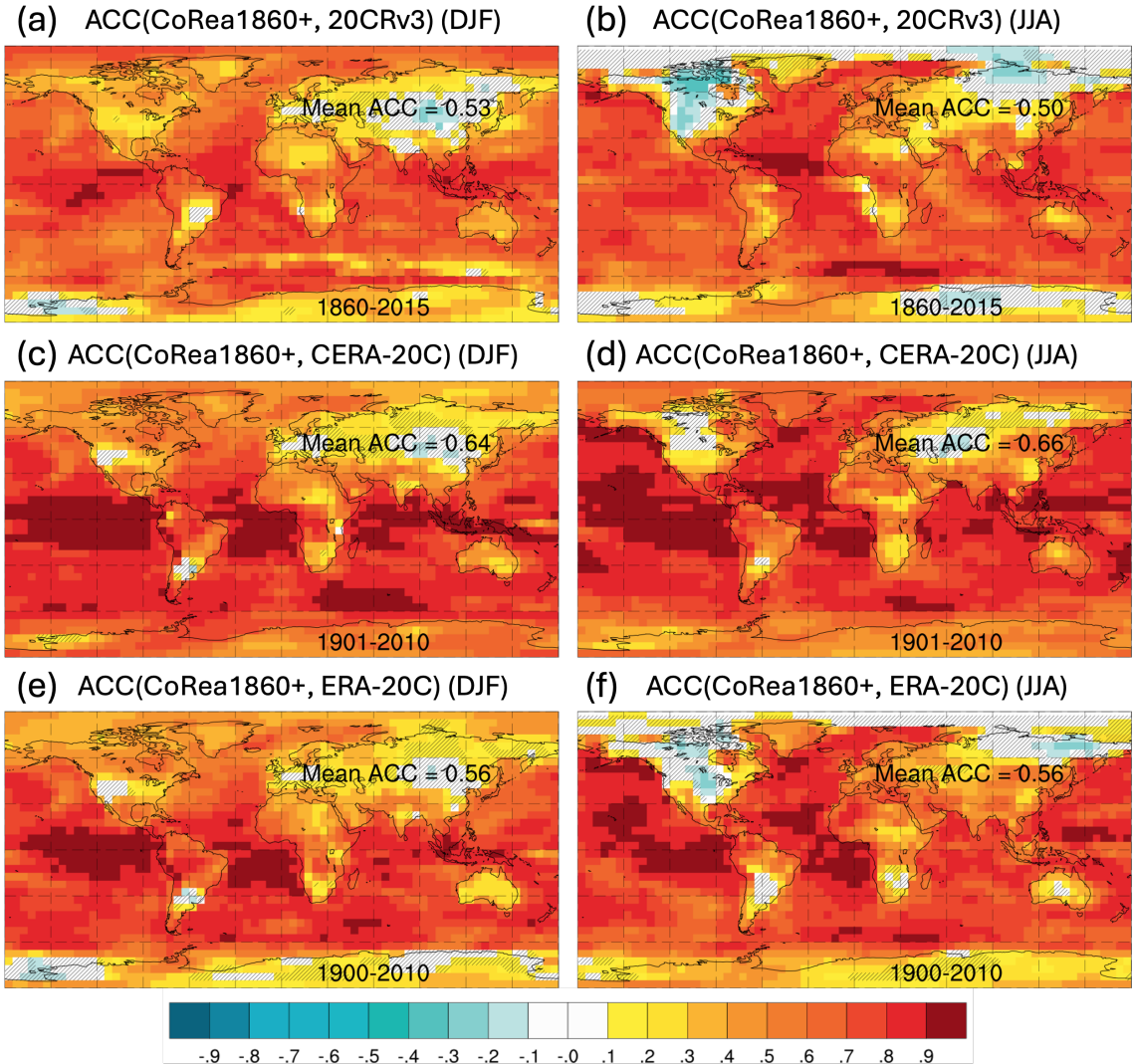
Figure R5: ACC of SAT in DJF or JJA of CoRea1860+ against 20CRv3, CERA-20C and ERA-20C. Grids that fail the significance test are marked with a slash. The period used to compute ACC corresponds to the overlapping period between CoRea1860+ and the specific reference dataset and is shown in Antarctica. The spatially averaged ACC is shown in Eurasia.
