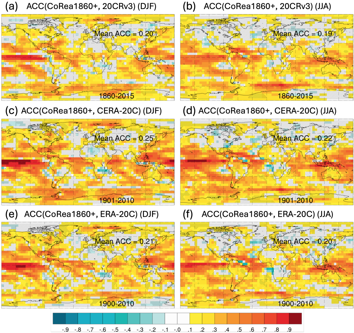
Figure R6: ACC of PRECIP in DJF or JJA of CoRea1860+ against 20CRv3, CERA-20C and ERA-20C. Grids that fail the significance test are marked with a slash. The period used to compute ACC corresponds to the overlapping period between CoRea1860+ and the specific reference dataset and is shown in Antarctica. The spatially averaged ACC is shown in Eurasia.
