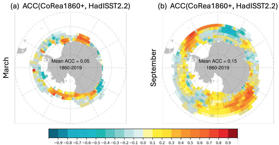
Figure R4: ACC of Antarctic sea ice concentration in March or September of CoRea1860+ against HadISST2.2. Grids that fail the significance test are marked with a slash. The period used to compute ACC corresponds to the overlapping period (i.e., 1860-2019) and is shown in Antarctica. The spatially averaged ACC is also shown in Antarctica.
