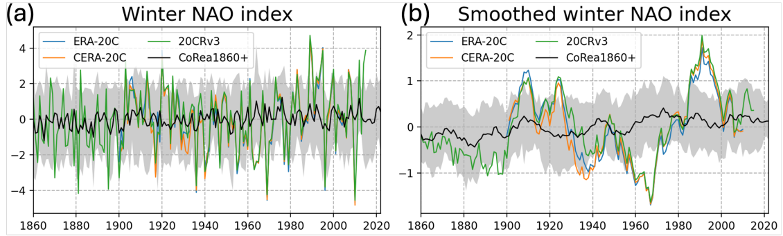
Figure R1: (a) Winter (December-March) station-based index of the NAO. (b) 10-year running average of the winter NAO index.
