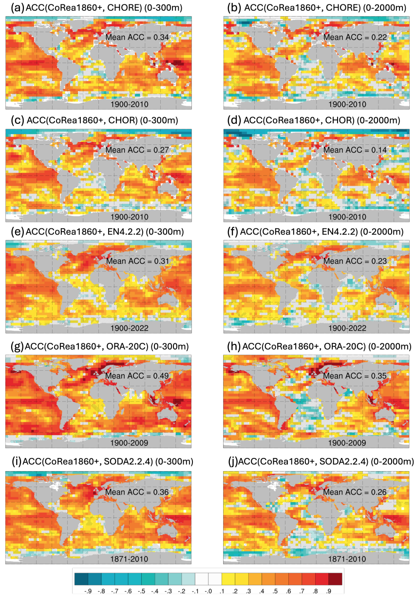
Figure R3: Same as Figure R2 but for detrended yearly OHC.
