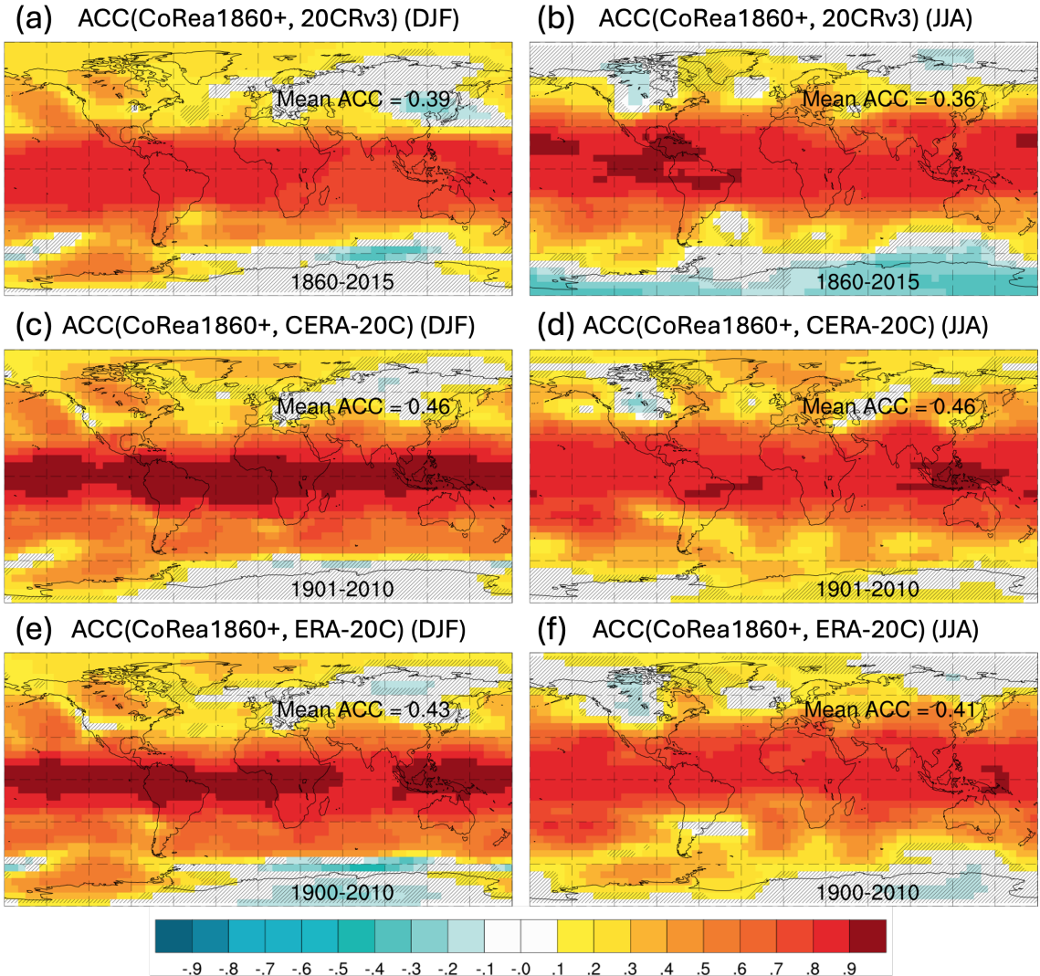
Figure R8: ACC of Z500 in DJF or JJA of CoRea1860+ against 20CRv3, CERA-20C and ERA-20C. Grids that fail the significance test are marked with a slash. The period used to compute ACC corresponds to the overlapping period between CoRea1860+ and the specific reference dataset and is shown in Antarctica. The spatially averaged ACC is shown in Eurasia.
