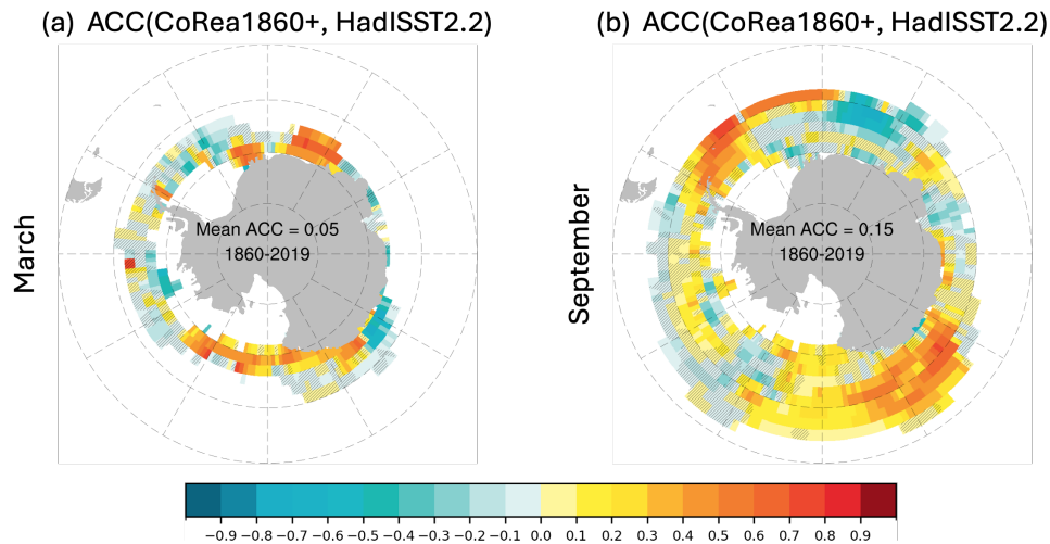
Figure R6: ACC of Antarctic sea ice concentration in March or September of CoRea1860+ against HadISST2.2. Grids that fail the significance test are marked with a slash. The period used to compute ACC corresponds to the overlapping period (i.e., 1860-2019) and is shown in Antarctica. The spatially averaged ACC is also shown in Antarctica.
