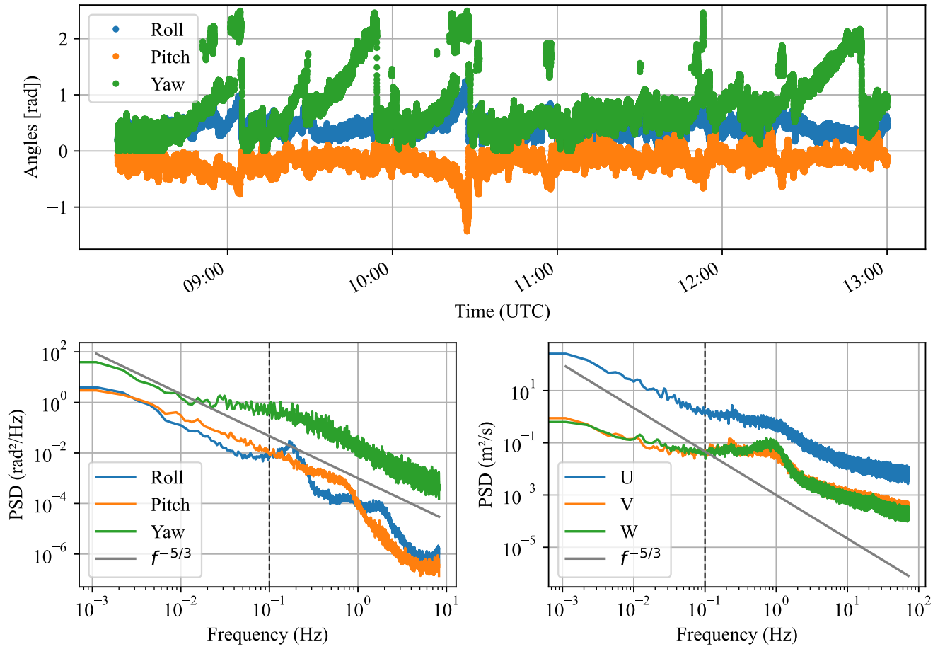
Figure 9. Time series of Euler angles measured by BNO1 on WinDart WD1-1 during flight 20220920.0750 (08:20–13:00 UTC) and corresponding power spectral density (PSD) of angles and velocity components. Spectral peaks above 0.1 Hz indicate platform motion effects on measured velocity fluctuations.
