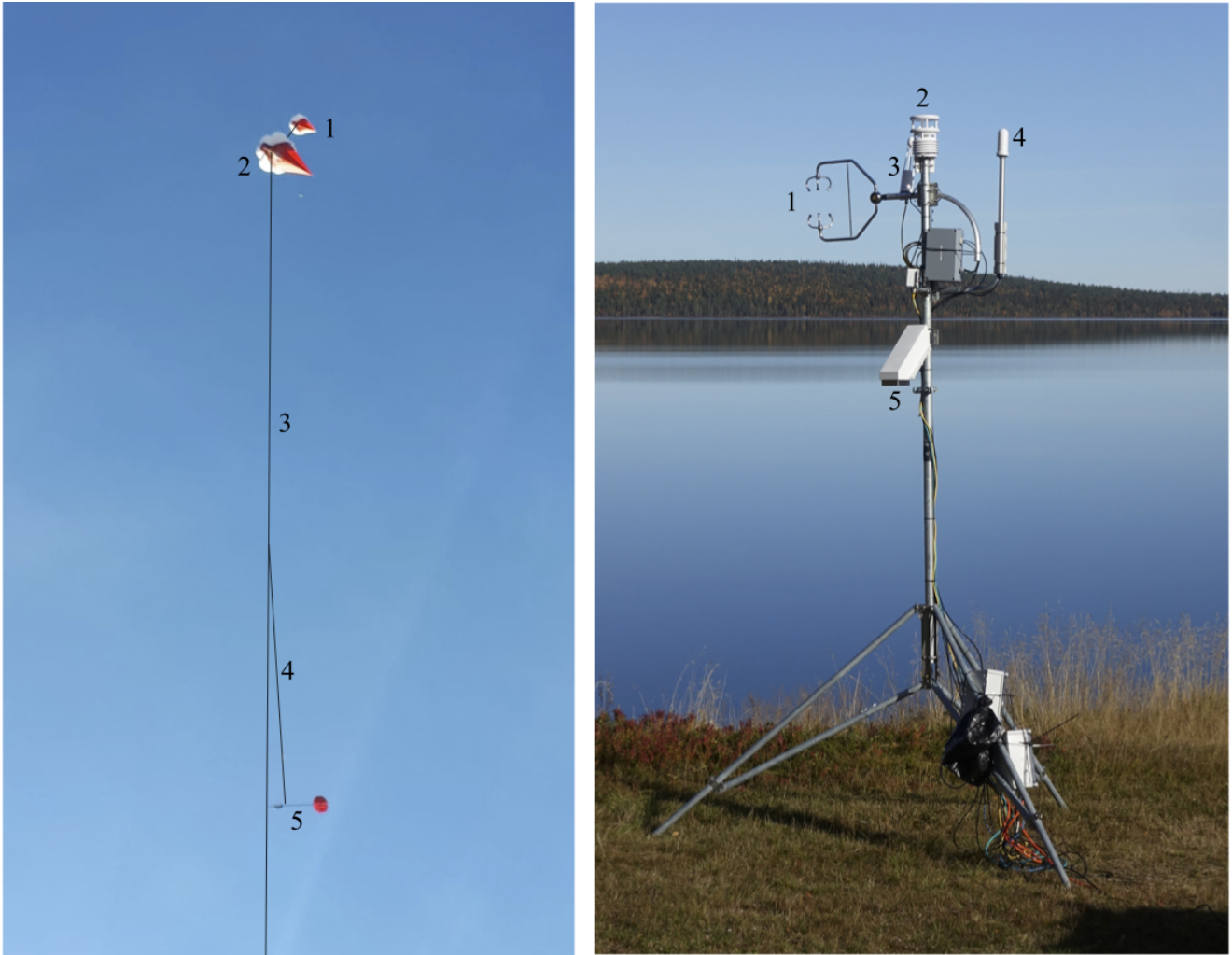
Figure 3. (Left) The Helikites of the MPCK platform (1, 2) lift a WinDart (5), which is connected to a line (4) and stabiliser, both attached to the main tether of the MPCK platform (3). (Right) The ground weather station with its main components: (1) Metek uSonic3 Class A-MP anemometer, (2) Lufft WS500UMB weather station including pressure, temperature, humidity and 2D wind velocity sensor, (3) Li-Cor LI-7500DS fast trace gas and humidity sensor, (4) Boltek LD-250 lightning detector, and (5) Campbell Scientific CS110 electric field meter.
