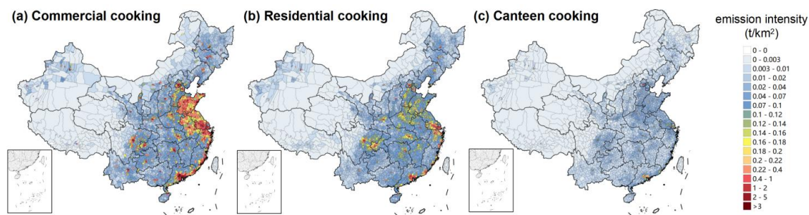
Figure. S6. Sector-specific spatial distributions of cooking emissions in 2021.
