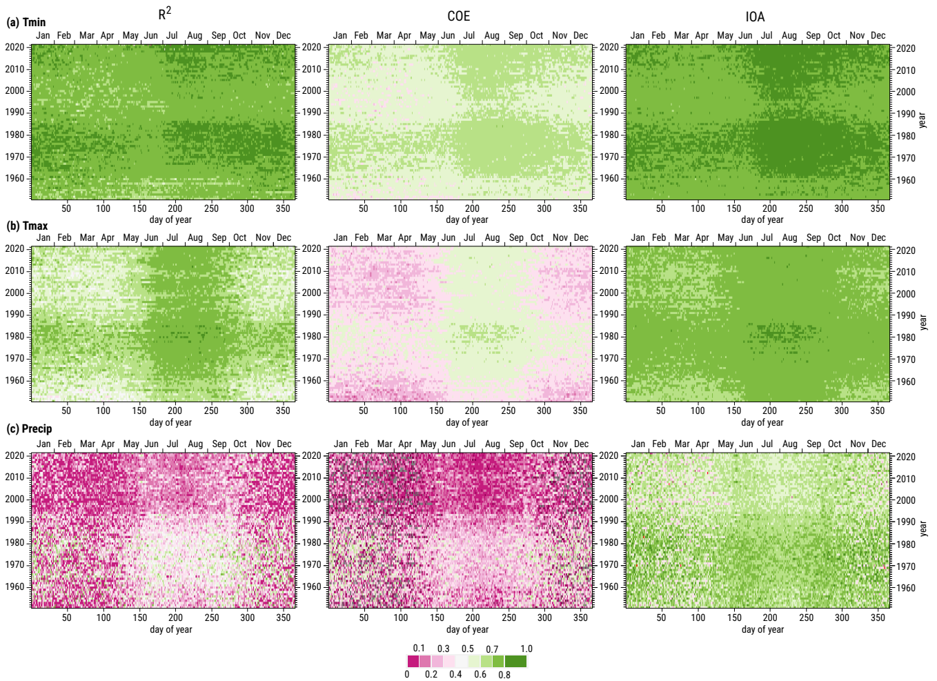
Figure 6. Performance indices – coefficient of determination (R 2 ), Coefficient of Efficiency (COE) and Index of Agreement (IOA) – for the daily interpolations developed in this work: (a) Minimum Temperature, (b) Maximum Temperature, and (c) Precipitation.
