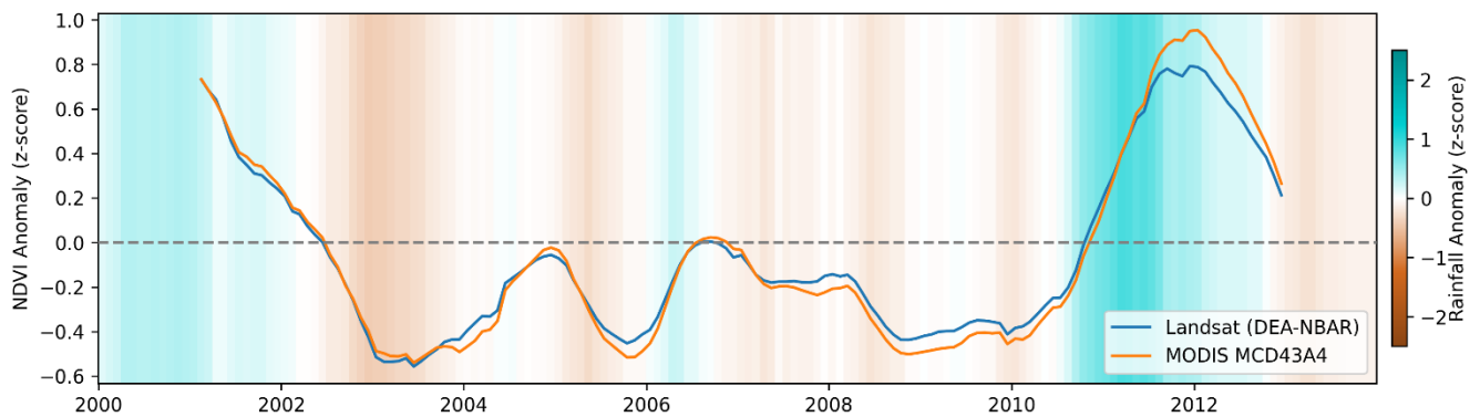
650 Figure A2: Standardised anomalies of the overlapping period between MODIS MCD43A4 NDVI and DEA's Landsat NDVI derived from the common baseline period of 2000-2012. Rainfall anomalies are derived from a longer baseline of 1982-2022.
