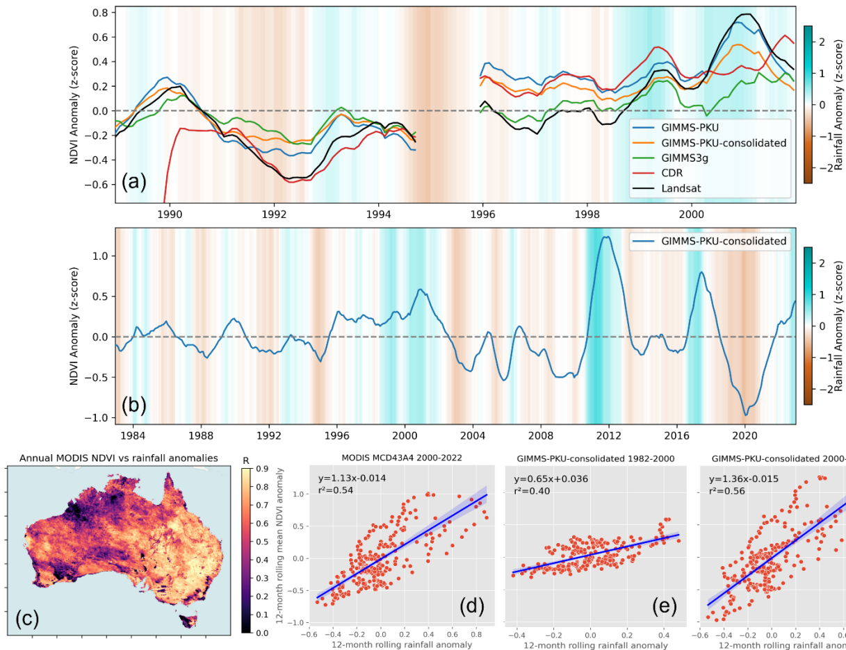
330 Figure 4: a) Twelve-month rolling mean standardised anomalies of Landsat, CDR, GIMMS3g, GIMMS-PKU, and GIMMS-PKU- consolidated NDVI, based on a common 1988-2012 climatology. Background shading represents twelve-month rolling mean standardised rainfall anomalies. All datasets, besides rainfall, have matching data gaps. b) Twelve-month rolling mean standardised anomalies of the NDVI_{PKU-consolidated} product (1982-2022 climatology). c) Pearson correlations between annual NDVI_{MCD43A4} anomalies and annual rainfall anomalies, shown here to demonstrate the strongly water limited nature of Australia’s vegetation. d- 335 f) Relationships between twelve-month standardised rainfall and NDVI anomalies averaged across Australia for different periods and different products. In (d) NDVI_{MCD43A4} and rainfall anomalies have been calculated against a 2000-2022 baseline. In (e-f) rainfall and NDVI_{PKU-consolidated} anomalies have been calculated against a 1982-2022 baseline. The relationships y=mx+c denotes the linear regression slope between rainfall and NDVI anomalies where y is NDVI anomalies, x is rainfall anomalies, and m is the slope coefficient. The slope coefficient can be considered an approximation of the sensitivity of NDVI to anomalous water supply aggregated over the continent. 340
