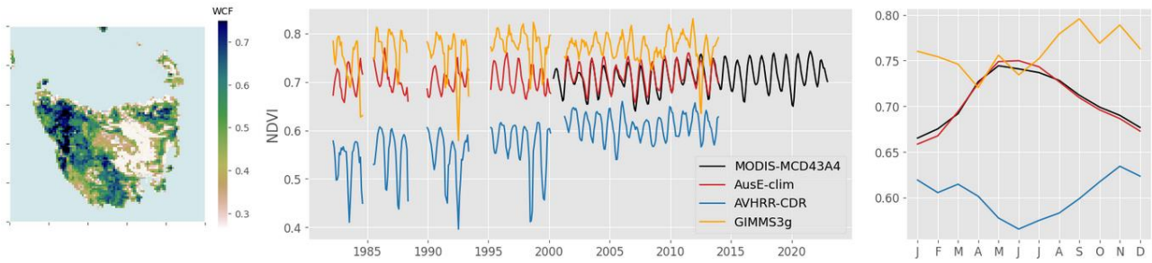
675 Figure A6: Same as Figure 6d-f but including NDVI_{GIMMS3g} to demonstrate that the very strong increasing trend in NDVI_{CDR} is likely an artefact of sensor transitions and poor calibration.
