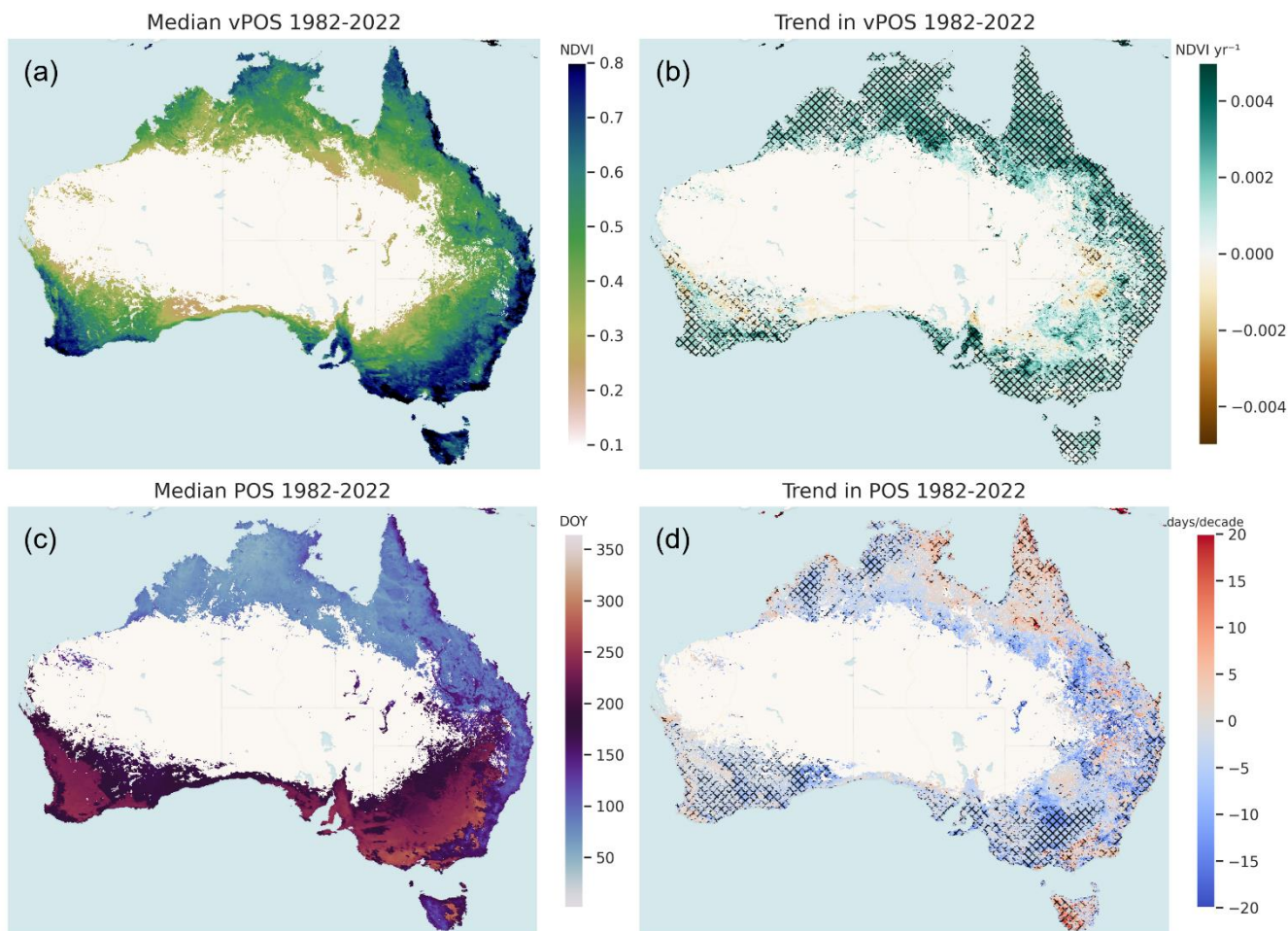
485 Figure 11: a) The median annual peak NDVI value (vPOS) from 1982-2022. b) Theil-Sen robust regression trends in vPOS. c) Median day-of-year that peak NDVI occurs (POS), 1982-2022. d) Theil-Sen robust regression trends in POS. Hatching on trend plots indicates significance at \alpha=0.05 using a Man-Kendall test. All plots are derived from the gap-filled ‘clim’ NDVI AusE dataset. Non-seasonal areas have been masked using the method described in section 2.4.
