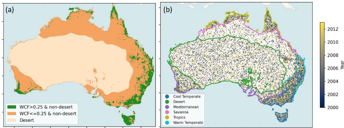
200 Figure 2: a) Regions delineating the spatial extent of the three modelling domains: desert, low woody cover fraction (WCF) and high WCF. b) The distribution of all independent validation points used to assess the model fits across the three modelling domains in (a); points are coloured by the year they are drawn from. Figure is overlaid with outlines of the six bioclimatic regions used to both stratify training points and for aggregating trends in later analysis.
