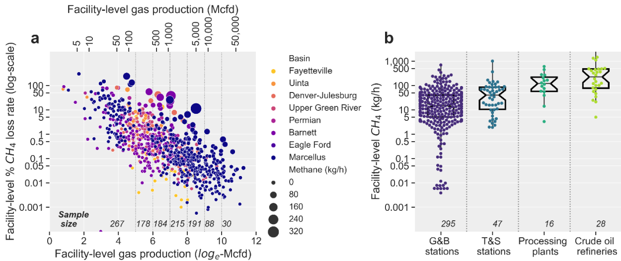
Figure 1. Previously reported facility-level measurement-based methane emissions data. a. Facility-level methane emissions data (percent methane loss rate) as a function of gas production rate ( n = 961 non-low production well sites). The bottom x -axis shows the log-normalized gas production rates, with dashed vertical lines delineating the seven production cohorts used to model total methane emissions. Sample sizes for each production cohort are shown at the bottom of the Fig. panel above the bottom x -axis tick labels. The top x -axis shows the same production data in Mcfd. Each point is color-coded by basin and sized by the quantified methane emission rate in kg/h. Not shown are measurements that were reported as below the method detection limits. b. Absolute methane emission rate data (kg/h) for gathering and boosting (G&B) compressor stations ( n = 295 ), transmission and storage (T&S) compressor stations ( n = 47 ), natural gas processing plants ( n = 16 ), and crude oil refineries ( n = 28 ). The swarm plots show individual facility-level measurements, while the notched box plots show the distribution, where the boxes represent the 25 th and 75 th percentiles and the whiskers extend to 1.5\times the interquartile range.
