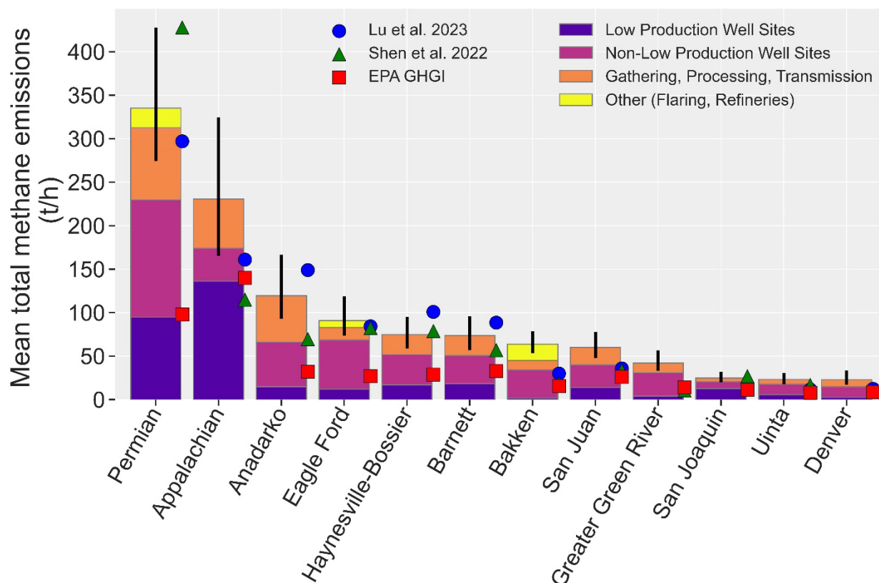
430 Figure 5. Basin-level differences in modelled mean total methane emissions and comparison with the EPA GHGI (Maasackers et al., 2023), TROPOMI-derived estimates (Shen et al., 2022) and GOSAT-derived estimates (Lu et al., 2023). See Supplementary Fig. 11 for a similar chart showing the state-by-state breakdown for the top 10 US emitting states based on the EI-ME inventory estimates.
