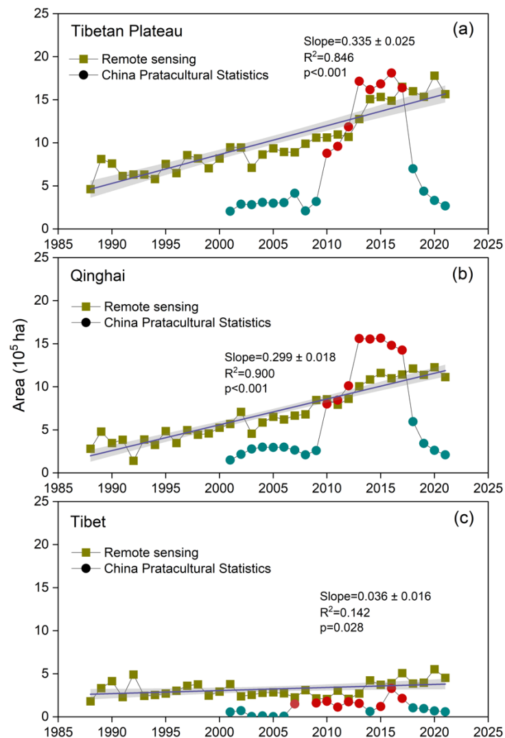
345 Figure 11. The time series of cultivated pasture areas based on remote sensing and the government statistics data for (a) the Tibetan Plateau, (b) Qinghai Province, and (c) the Tibet Autonomous Region. The red dots in the China Pratacultural Statistics time series correspond to the years when the cultivated pasture statistical caliber aligned with our definition of cultivated pasture in the remote sensing mapping efforts.
