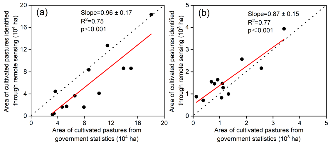
Figure 8. Comparison of the areas of cultivated pastures mapped using remote sensing with those from the government statistics at the county level for 2021 in (a) Qinghai Province and (b) the Tibet Autonomous Region. The government statistics of cultivated pasture areas were from Qinghai Forestry and Grassland Bureau and the Tibet Autonomous Region Agriculture and Rural Affairs Department.
