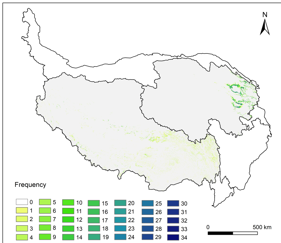
340 Figure 10. The number of years that cultivated pasture existed in each 30-m grid in Qinghai Province and the Tibet Autonomous Region from 1988 to 2021.
