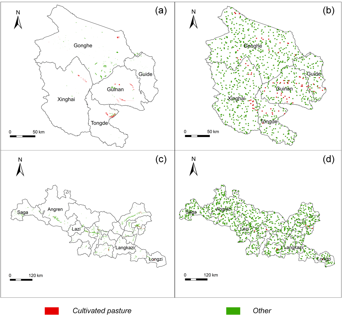
175 Figure 3. The spatial distribution of the training polygons and the validation points in the pilot study regions. The training polygons (a, c) were recorded during the 2021 field campaign, and the 1,000 independent random validation points (b, d) in each pilot study region were labelled with the aid of high-resolution images on Google Earth.
