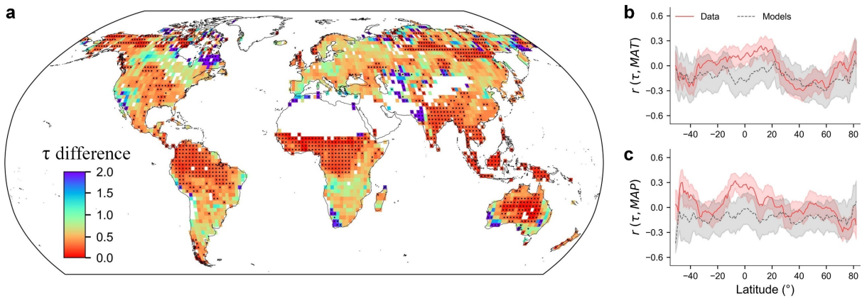
Figure 8: Comparisons of soil organic carbon turnover times ( \tau ) from our data-derived estimates and from Earth system models (ESMs). a , Biases in \tau represented by ratios of between data-derived to model-derived values across the global grid cells. Black points indicate locations where \tau from ESMs are outside the 0.05 and 0.95 quantiles from the prediction uncertainty in our data-derived estimations. b , c , Comparisons of associations of data- and models (ESMs)-derived \tau to mean annual temperature (MAT) ( b ) and mean annual precipitation (MAP) ( c ) along latitude gradients. The y-axis shows partial correlations ( r ) of \tau with two climate factors, controlling for precipitation when calculating the correlation between \tau and temperature (and vice versa).
