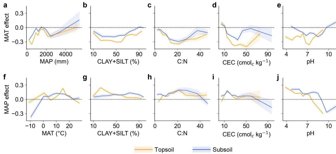
Figure 6: The climatic effects on top- and subsoil organic carbon turnover time ( \tau ) interacted by other factors. The lines show the mean annual temperature (MAT) effect and mean annual precipitation (MAP) effect on \tau in response to another climatic variable and four important soil physio-chemical (including the fine particle-size fraction [CLAY+SILT], carbon-to-nitrogen ratio [C:N], cation exchange capacity [CEC] and soil pH) variables. The variables on the x-axis can be considered as “interactive factors”, which influence the MAT and MAP effect on \tau . The values on the lines above or below dashed horizontal lines indicate the positive or negative climatic effect on top- or subsoil \tau (the MAT/MAP effect was calculated by the partial regression coefficient between MAT/MAP and \tau ) in response to the corresponding values of interactive factors. The shaded areas on the lines represent confidence intervals for the results of partial correlation analysis.
