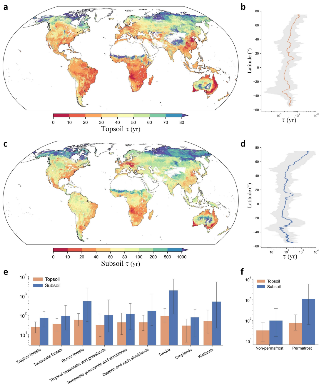
Figure 3: Global patterns of top- and subsoil organic carbon turnover times ( \tau , yr). Global distributions of \tau at top- (0–0.3 m) (a) and subsoil (0.3–1 m) (c) layers. The predicted maps with a spatial resolution of 30 arcsec ( \sim 1 km at the Equator) were generated \tau -environment relationships using a machine learning model trained from global soil profile observations and their environmental covariates. b, d, Latitudinal patterns of top- and subsoil \tau . Orange and blue lines represent the average \tau at top- and subsoil over latitudes, respectively. The shaded grey areas represent the variations of \tau between 2.5 th and 97.5 th percentiles along latitudes. e, f, Average \tau at two layers in different main biomes. Error bars show the 95% percentile intervals of the spatial predictions within each biome.
