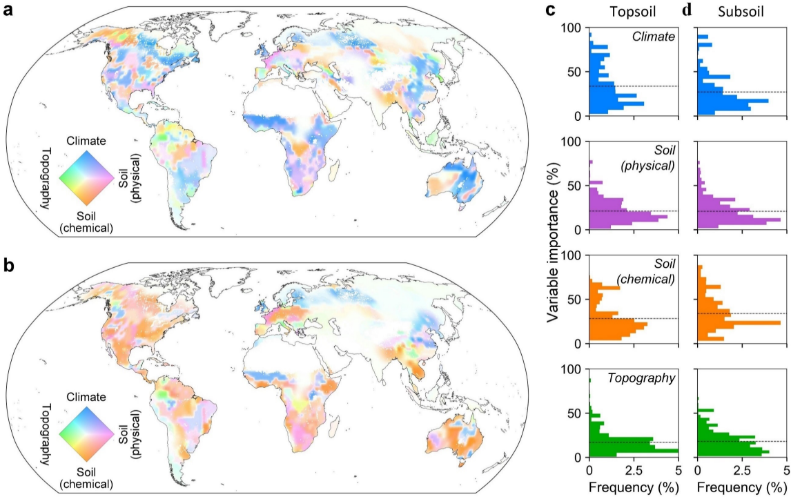
Figure 7: Local-level analysis of dominating factors of top- and subsoil organic carbon turnover time ( \tau ). Global maps of dominant factors controlling \tau in top- (a) and subsoil (b) at the local scales. Maps were created by interpolating all results of factor importance from modelling using the sample data within each local area stratified by the ecoregion map. The lighter color would be displayed if the reliability of the local result is low with a smaller number of available samples for analysis. Histograms of the local-level percentage contribution of each variable category in controlling top- (c) and subsoil (d) \tau across all local areas, respectively. Dashed lines represent the mean values.
