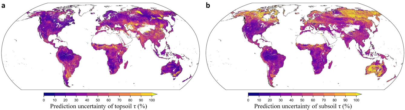
Figure 4: Uncertainty maps of predicted soil organic carbon turnover time ( \tau ) in top- (a) and subsoil (b) layer. The uncertainty was quantified by using quantile regression forests. The values shown in the maps represent the prediction interval ratio (PIR), which is the ratio of the range between lower and upper limit (90% prediction interval bounded by the lower [0.05 quantile] and upper [0.95 quantile] limits) over the median (0.50 quantile) of the predictions. 305
