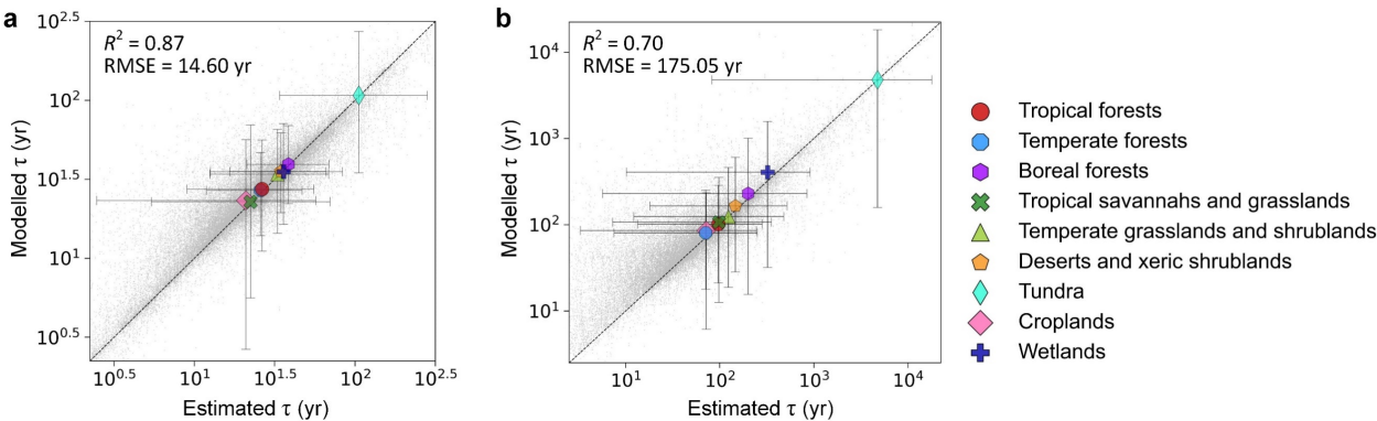
265 Figure 2: Validation plots for predictions of soil organic carbon turnover time ( \tau , yr) in top- (a) and subsoil (b) layer. Predictions were generated using random forest regression models. Grey dots are the estimated \tau values based on observations at soil profiles and the predicted values for all validation samples using 10-fold cross-validation. Colored points represent biome-level validation plot. Error bars show 95% percentile intervals of \tau in each biome. Black lines indicate the regression lines between predicted and measured values. Axes are log 10 -transformed to account for high skewness of \tau .
