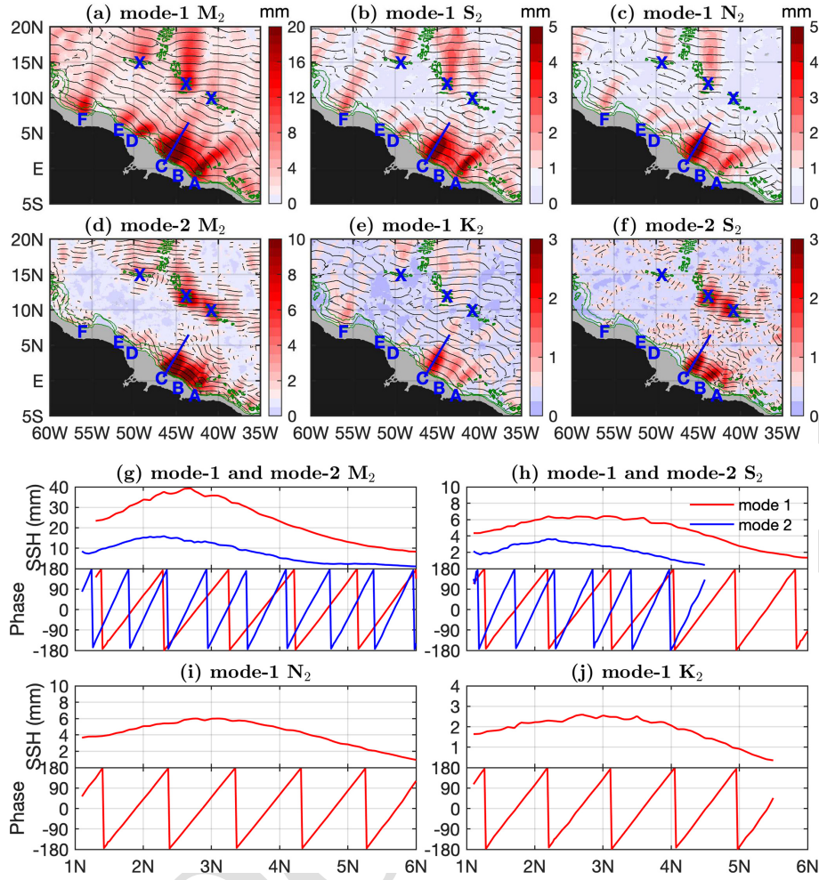
Figure 16. Northeastward semidiurnal internal tidal beams off the Amazon shelf. (a–f) Northeastward internal tide components ( -45^\circ – 135^\circ ). Black lines indicate the 0^\circ co-phase charts. Green contours indicate the 1000, 2000, and 3000 m isobaths. Each constituent has up to six isolated beams off the Amazon shelf (a–f). Blue lines highlight the strongest beams generated at the mouth of the Amazon River. Beams generated at the Mid-Atlantic Ridge are marked. (g–j) Along-beam amplitudes and phases.
