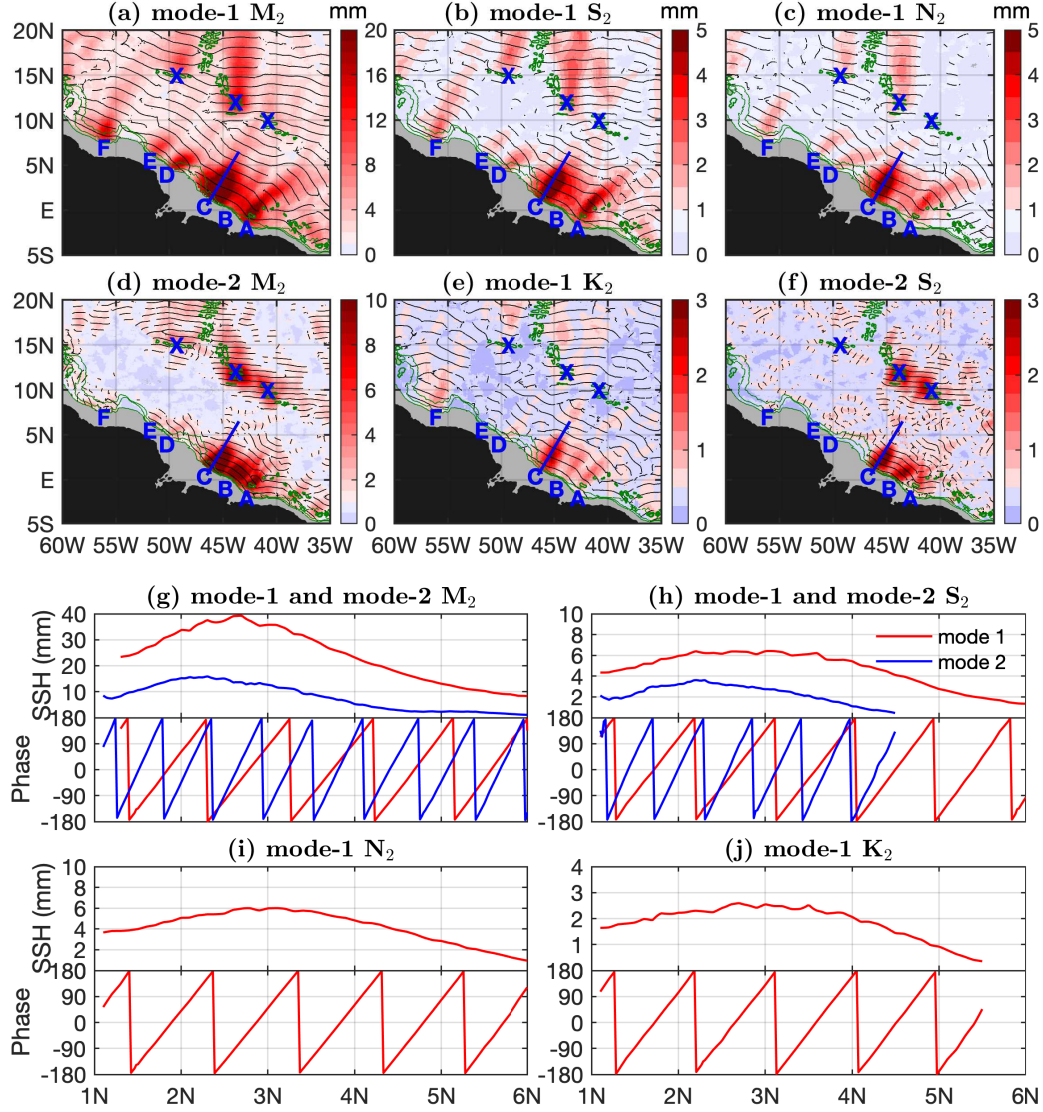
Figure 16. Northeastward semidiurnal internal tidal beams off the Amazon shelf. (a)-(f) Northeastward internal tide components ( -45^\circ – 135^\circ ). Black lines indicate the 0^\circ co-phase charts. Green contours indicate the 1000-, 2000-, and 3000-m isobaths. Each constituent has up to 6 isolated beams off the Amazon shelf (labeled A–F). Blue lines highlight the strongest beams generated at the mouth of the Amazon River. Beams generated at the Mid-Atlantic Ridge are marked. (g)-(j) Along-beam amplitudes and phases.
