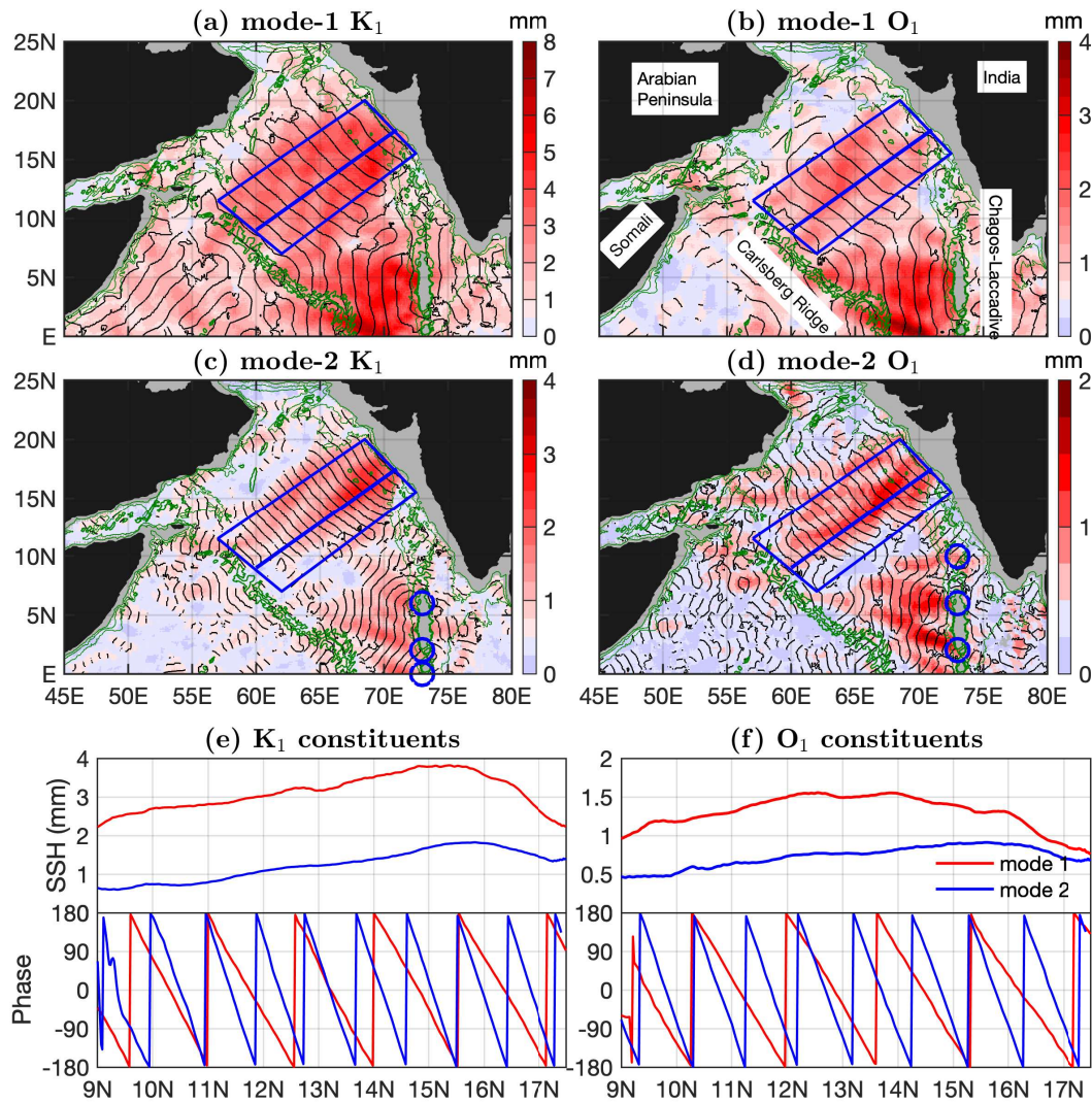
Figure 17. Westward diurnal internal tidal beams in the Arabian Sea. (a)-(d) Westward internal tide components ( 90^\circ – 270^\circ ). Black lines indicate the 0^\circ and 180^\circ co-phase charts. Internal tides with amplitudes lower than 0.5 mm are shown in light blue. Green contours indicate the 1000-, 2000-, and 3000-m isobaths. Blue circles mark some isolated mode-2 beams at the Chagos–Laccadive Ridge. (e, f) Along-beam amplitudes (averaged across the beam) and phases (along the central line).
