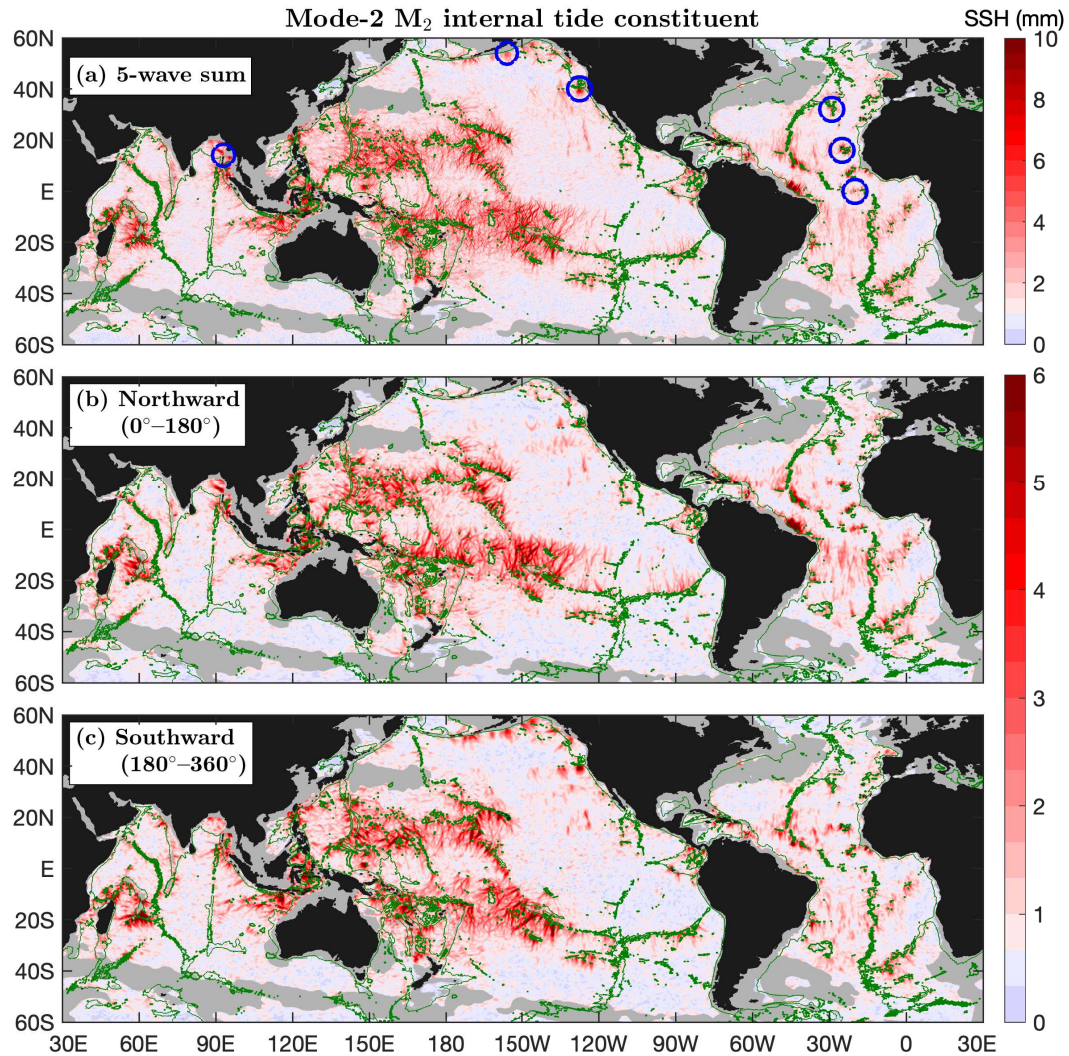
Figure 5. As in Figure 4 but for the mode-2 M_2 internal tide constituent. Well-defined long-range internal tidal beams are associated with notable topographic features. Blue circles mark some isolated beams. Mode-2 M_2 beams are narrower and shorter than mode-1 M_2 beams.
