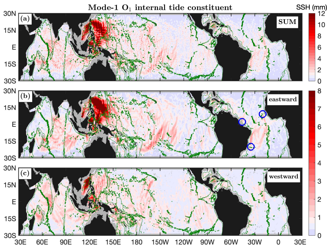
Figure 12. As in Figure 10 but for the mode-1 O_1 internal tide constituent. Blue circles mark isolated mode-1 O_1 beams.
