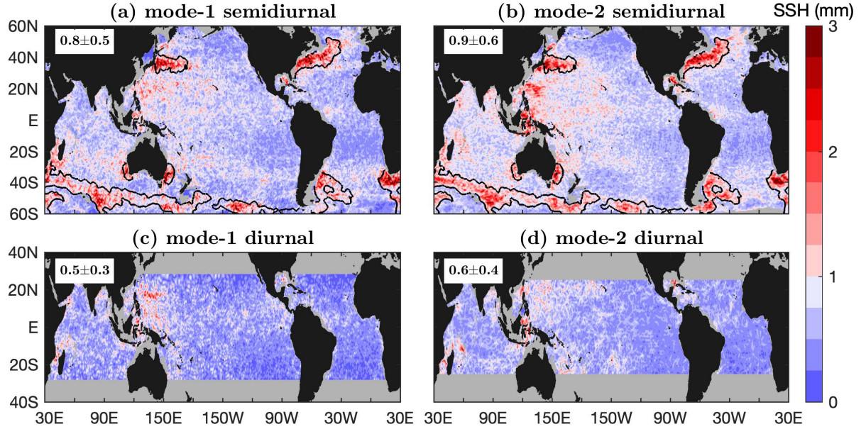
Figure 2. Model errors. For each constituent, the global mean and one standard deviation are given in the upper left corner. Black contours indicate regions of large model errors due to mesoscale contamination.
