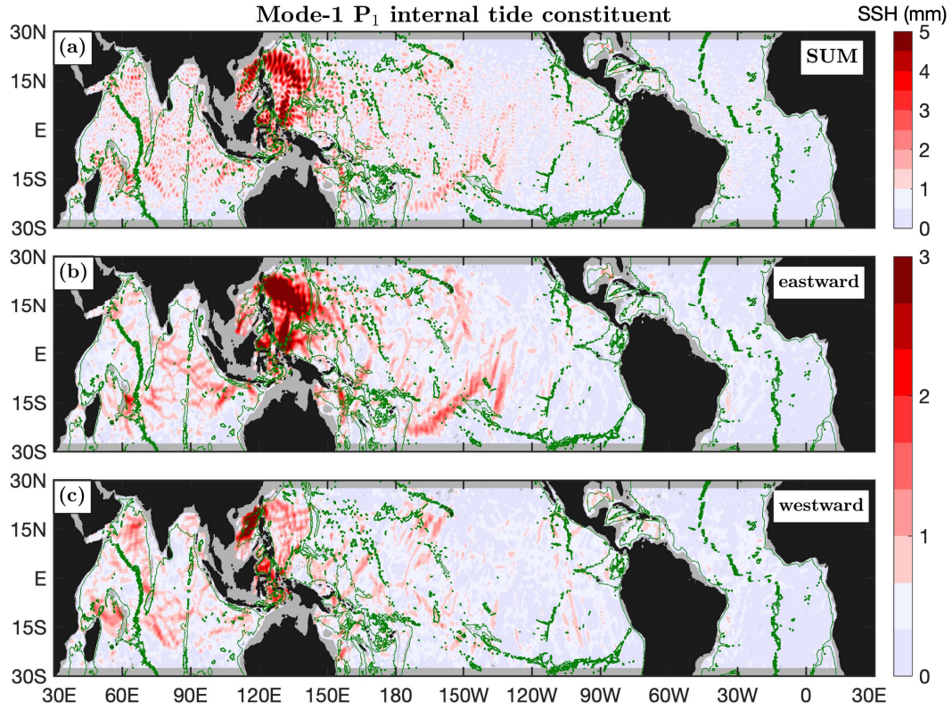
Figure 14. As in Figure 10 but for the mode-1 P_1 internal tide constituent.
