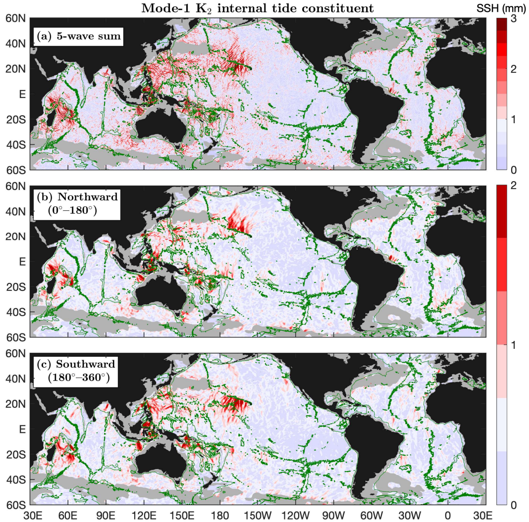
Figure 9. As in Figure 4 but for the mode-1 K_2 internal tide constituent.
