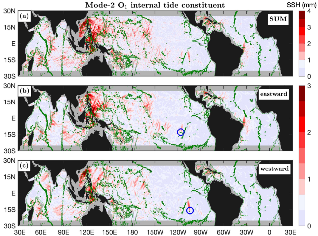
Figure 13. As in Figure 11 but for the mode-2 O_1 internal tide constituent. Blue circles mark two isolated beams in the eastern Pacific Ocean.
