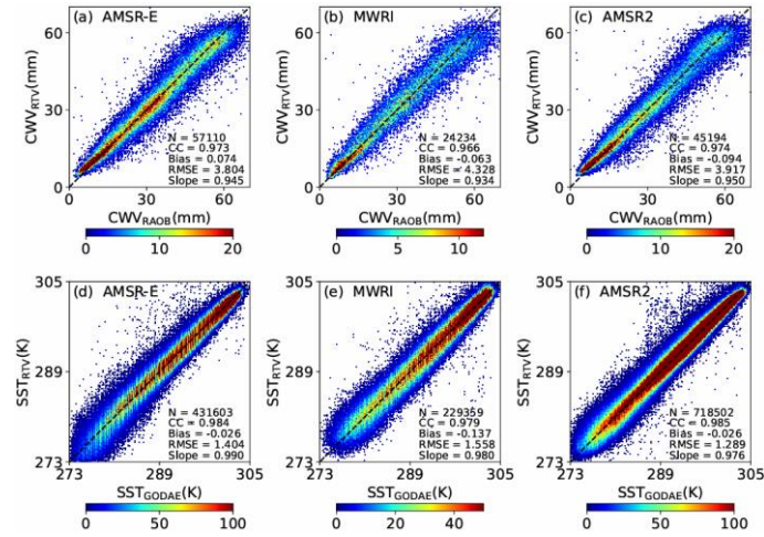
Figure 5: Density scatter diagram of retrieved CWV (top) and SST (bottom) versus in-situ measurements ( CWV_{RAOB} and SST_{GODAE} ). From left to right: AMSR-E, MWRI, and AMSR2. The black dotted lines represent the diagonal. (N: Sample number; CC: Correlation coefficient; RMSE: Root mean square error; Slope: Slope of linear regression).
