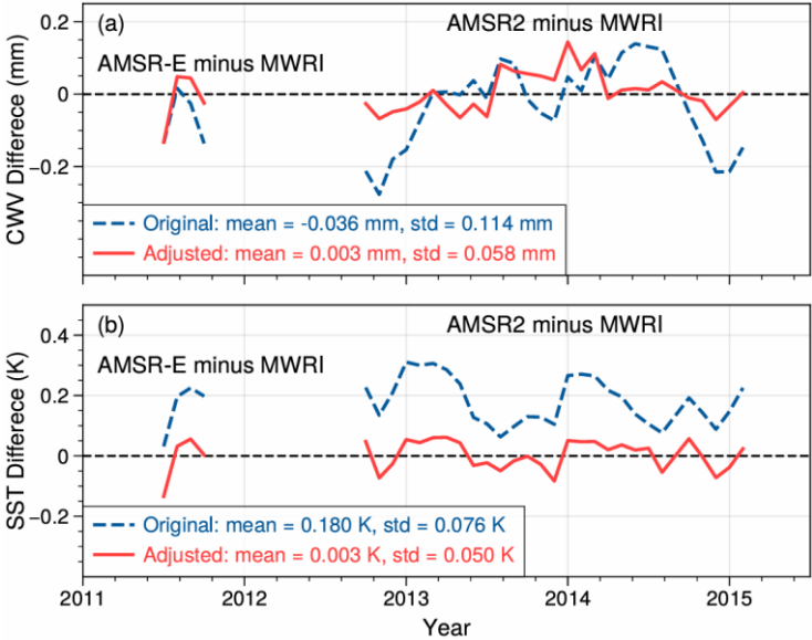
Fig. 4 Monthly mean differences between MWRI and the other two instruments for (a) CWV and (b) SST over the global ocean during their overlapping period. The blue dashed and red solid lines indicate the differences before and after diurnal adjustment, respectively. The mean biases and standard deviations are shown in the legends.
