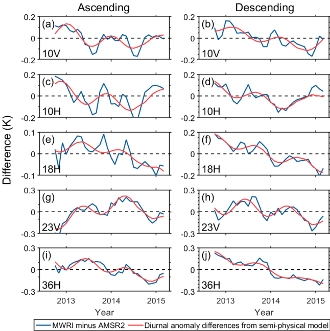
290 Figure 3: Inter-satellite differences ( TB_{MWRI}(X, t, m) - TB_{AMSR}(X, t, m) ) before diurnal drift adjustment (blue lines) ( \Delta TB' = TB'(X, t, m) - TB_{AMSR}(X, t, m) , blue lines) and diurnal anomaly differences ( D_{MWRI}(X, m, L) , red lines) derived from the semi-physical model over the global ocean. The differences are grouped into (left) ascending and (right) descending data separately, with the channels shown from (top) to (bottom): 10V, 10H, 19H, 23V, and 37H.
