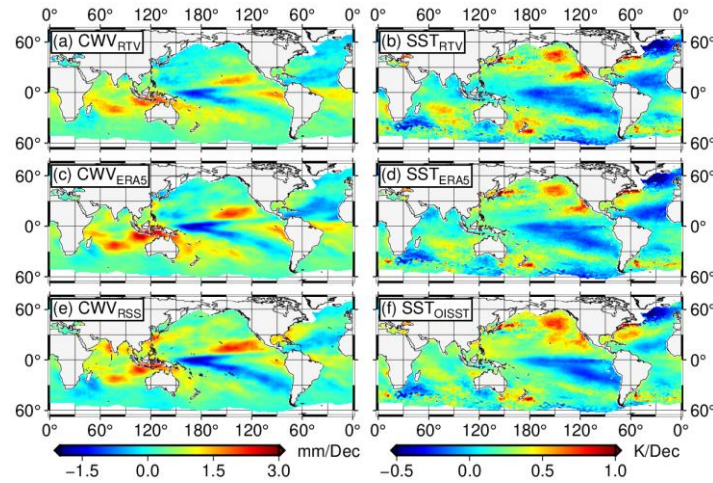
475 Figure 10: Global trend distribution for CWV (left) and SST (right) from 2002 to 2022. From top to bottom: CDR RTV , ERA5, and RSS or OISST.
