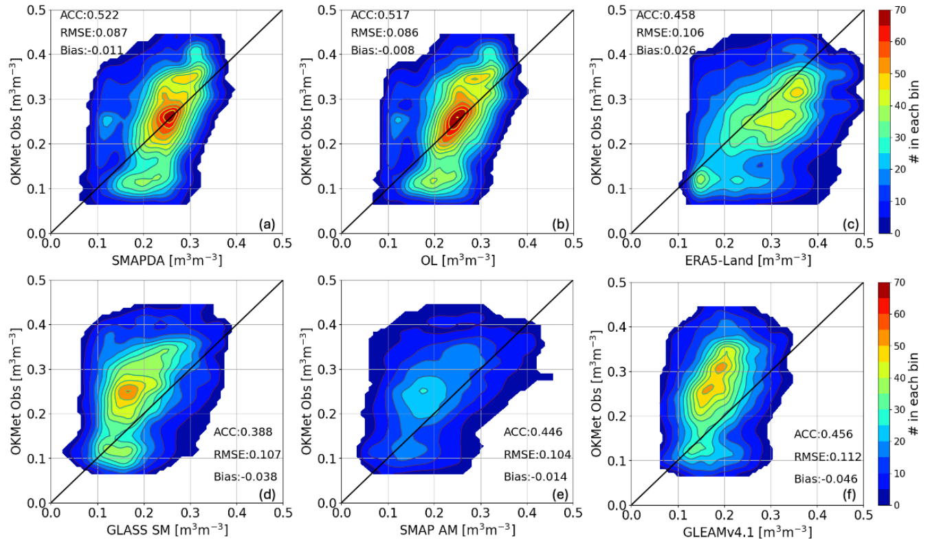
485 Figure 9 Similar to Figures 4 and S1, but for results computed against the OKMet observations.
