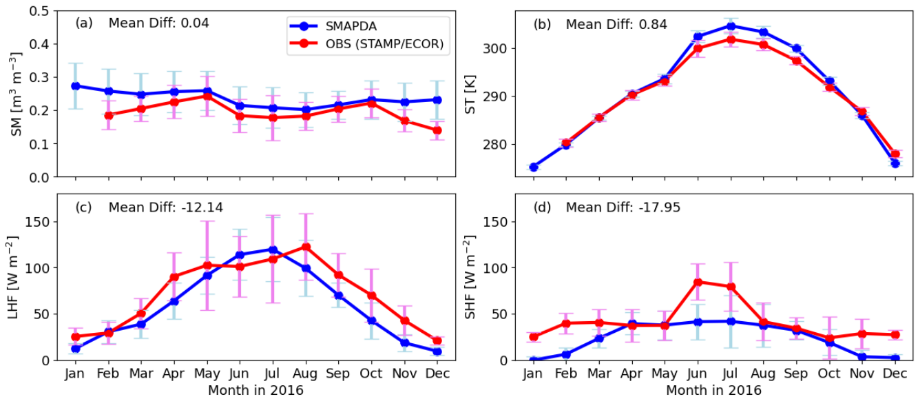
515 Figure 11 Timeseries of monthly mean of (a) SM, (b) ST, (c) LHF, and (d) SHF. Blue (red) line with circles represents results obtained from SMAPDA simulations (ARM SGP observations [STAMP/ECOR]) as computed across six ARM SGP sites (Figure 1a)
