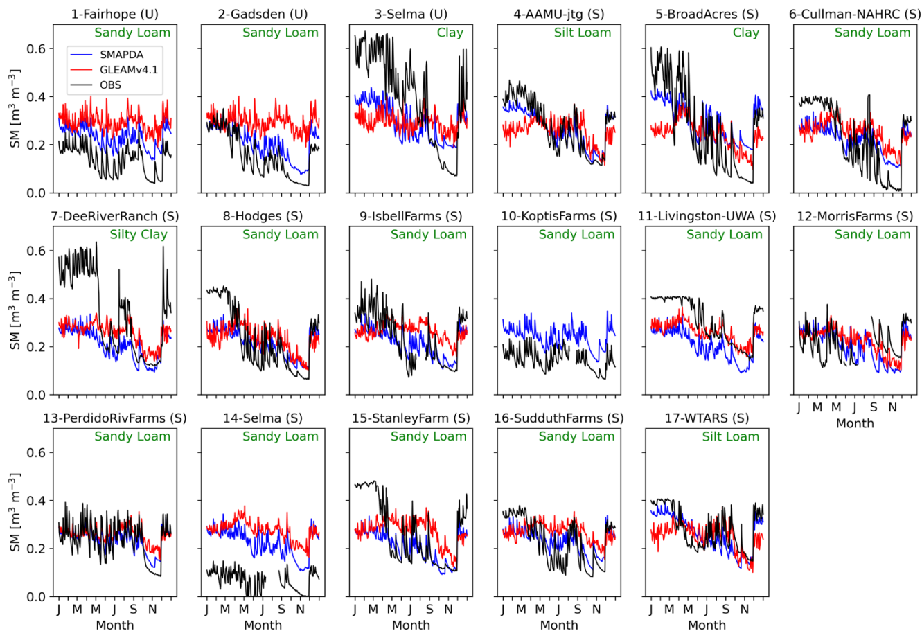
585 Figure 15 SM daily timeseries comparison at each in-situ observation location. The numbers given in the title above each panel correspond to the locations as marked by the numbered white circles in Figure 12. The site names and the corresponding observational networks (as indicated by either U (USCRN) or S (SCAN) in the parenthesis) are readable from the titles. Soil texture type is indicated by green texts in the top right corner of each panel.
