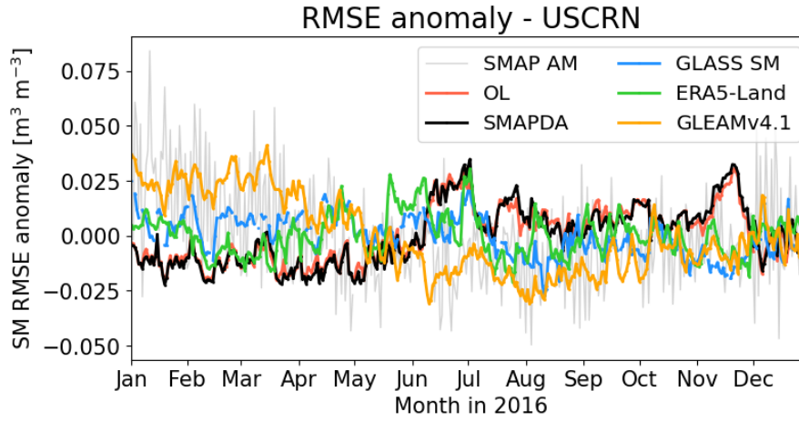
Figure 8 The SM RMSE anomaly timeseries computed against USCRN observations during 2016. Results of SMAP AM, OL, SMAPDA, ERA5-Land, GLEAMv4.1, and GLASS SM are denoted by colored lines as indicated in the legend.
