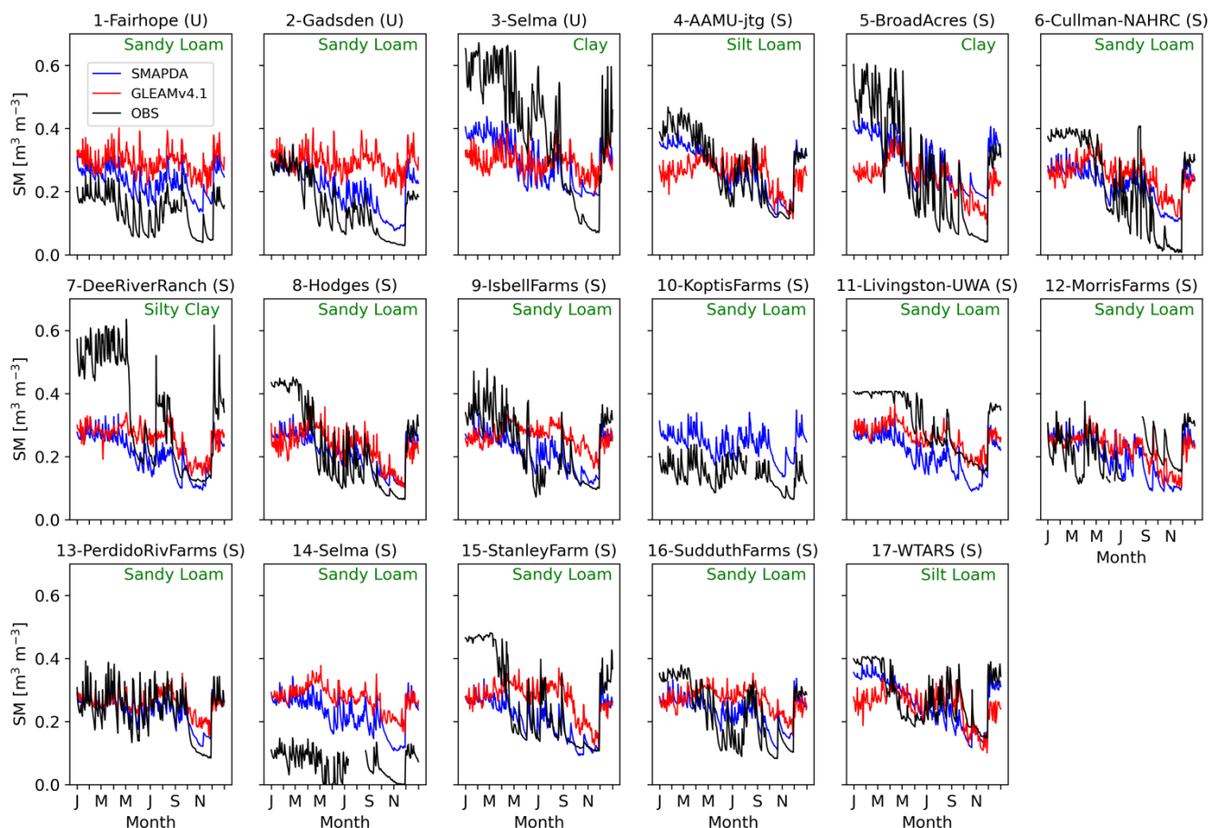
Figure 13-15 SM daily timeseries comparison at each in-situ observation location. The numbers given in the title above each panel correspond to the locations as marked by the numbered white circles in Figure 4-12. The site names and the corresponding observational networks (as indicated by either U (USCRN) or S (SCAN) in the parenthesis) are readable from the titles. Soil texture type is indicated by green texts in the top right corner of each panel.
