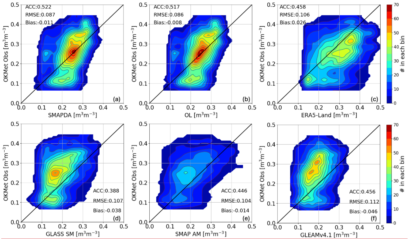
Figure 8-9 Similar to Figures 4 and S1, but for results computed against the OKMet observations.
