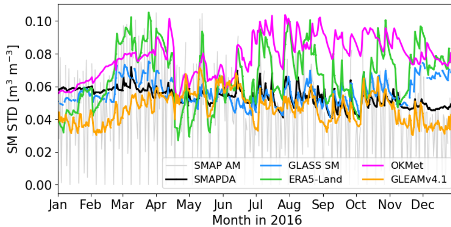
Figure 9-10 Daily timeseries of SM standard deviation across OKMet sites computed for each SM estimate.
