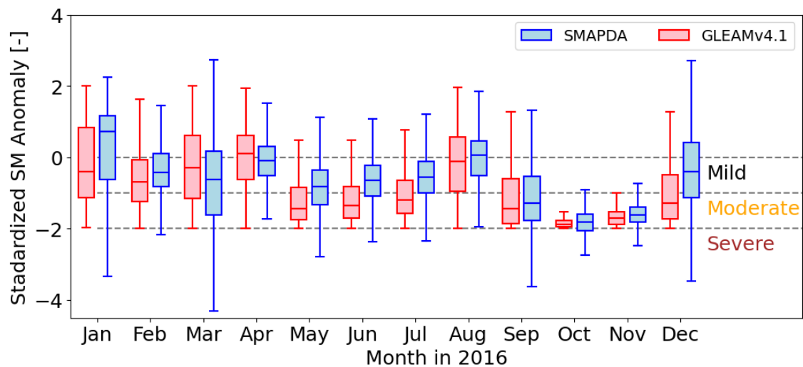
595 Figure 13 Box and whisker plot for monthly standardized SM anomaly (SSA) computed for SMAPDA and GLEAMv4.1 data in 2016 referenced by their own climatology (2012 - 2016). Dashed lines denote the thresholds for the defined drought conditions.
