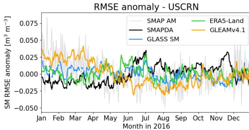
Figure 7-8 The SM RMSE anomaly timeseries computed against USCRN observations during 2016. Results of SMAP AM, ERA5-Land, SMAPDA, GLEAMv4.1, and GLASS SM are denoted by colored lines as indicated in the legend.
