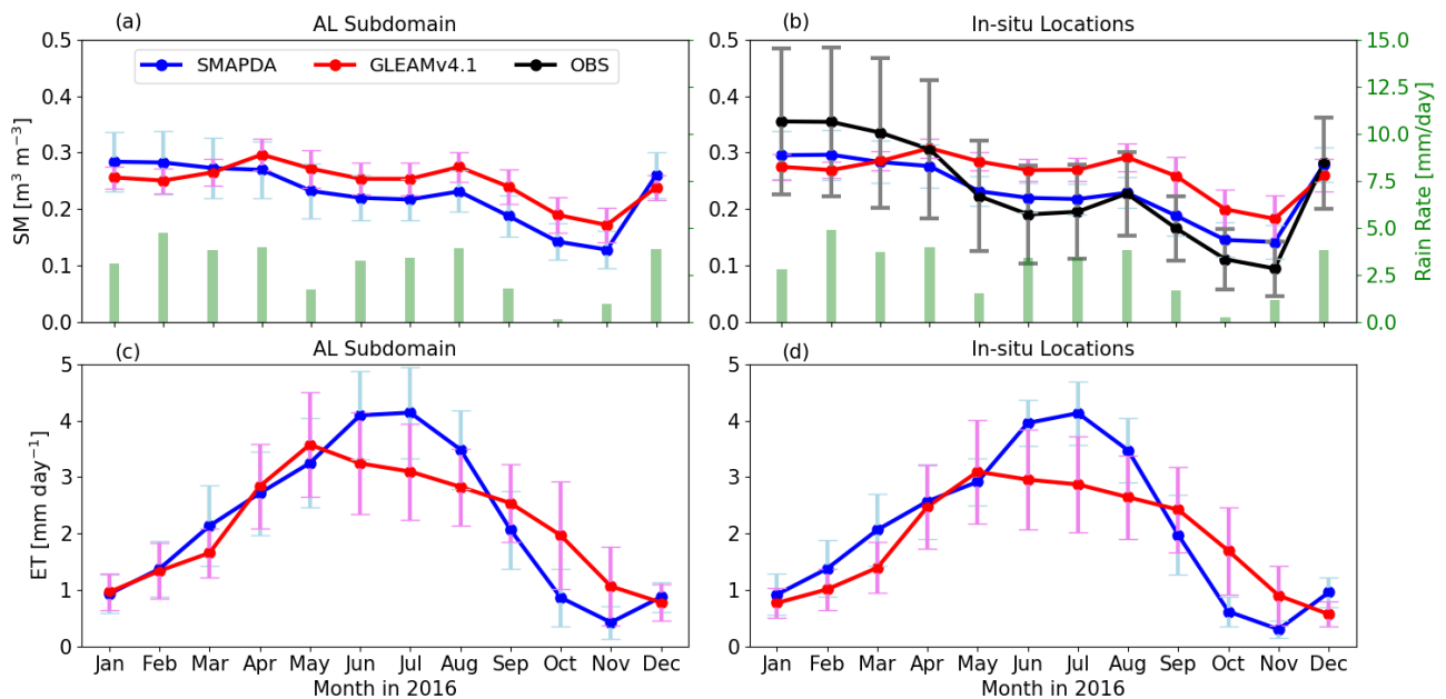
600 Figure 14 Monthly mean and standard deviation (denoted by error bars) of SM (a, b) and ET (c, d) over the AL subdomain and among 17 in-situ observation locations as denoted in Figure 4+12. The mean rain rate represented by green bars in (a) and (b) are computed from SMAPDA correspondingly.
