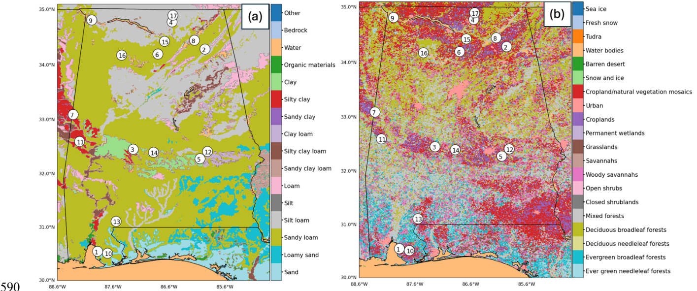
Figure 124 The zoomed-in maps of (a) soil and (b) land cover types over the AL subdomain as marked in Figure 1a. The locations of 17 valid observational sites from USCRN and SCAN are denoted by the white circles with numbers overlaid in correspondence of panels in Figure 13.
