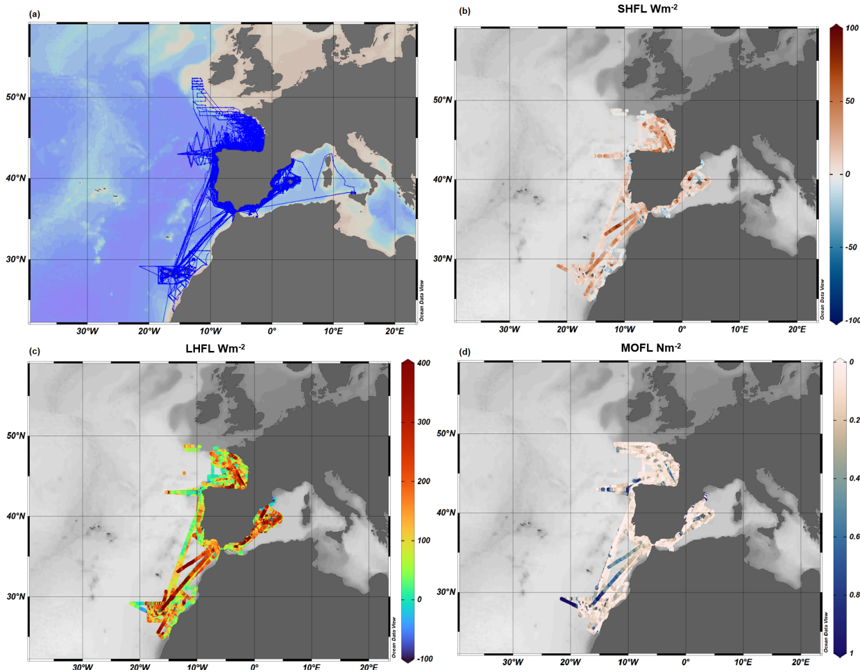
Figure 3. AJ, RM, MO and CS vessels' trajectories (a), and SHFL (b), LHFL (c) and MOFL (d) along the AJ, RM, MO, CS vessel's trajectories (a) obtained during the whole extended period 2011-2023.
