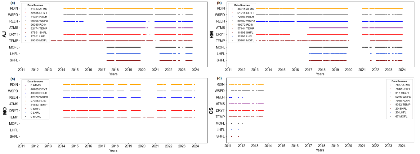
Figure 2. Data Quality controlled data records timeline from 2011 to 2023 for each meteorological and TSG variables, as well as for SHFL , LHFL , MOFL products for each vessel, AJ (a), RM (b), MO (c), CS (d). Quality-control-applied-Number The size of data sample for each magnitude-variable is indicated in the plot legend.
