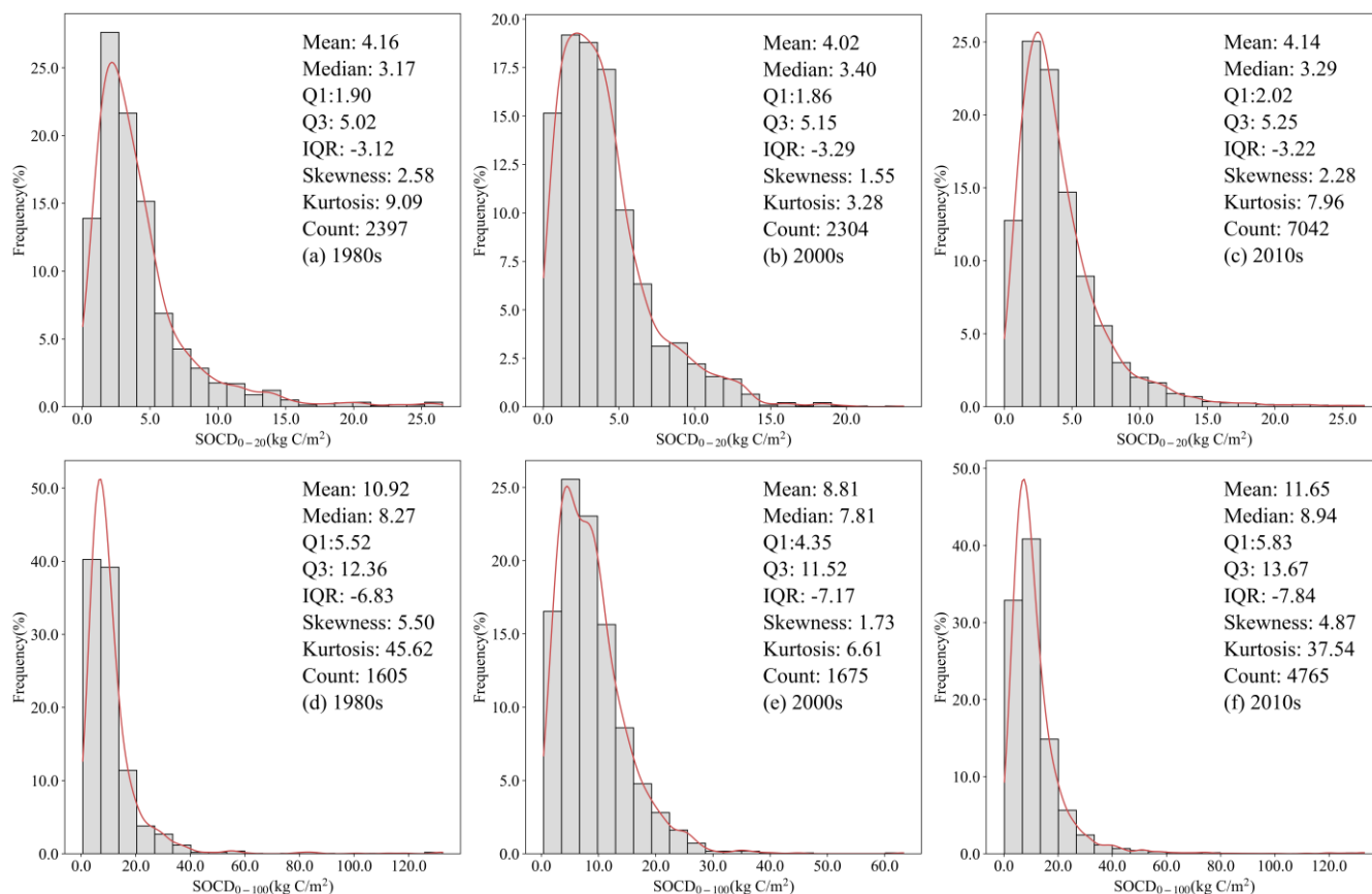
Figure 4. Statistical characteristics of soil sample points in different periods. Frequency distribution of SOCD data with the soil depth of 0-
