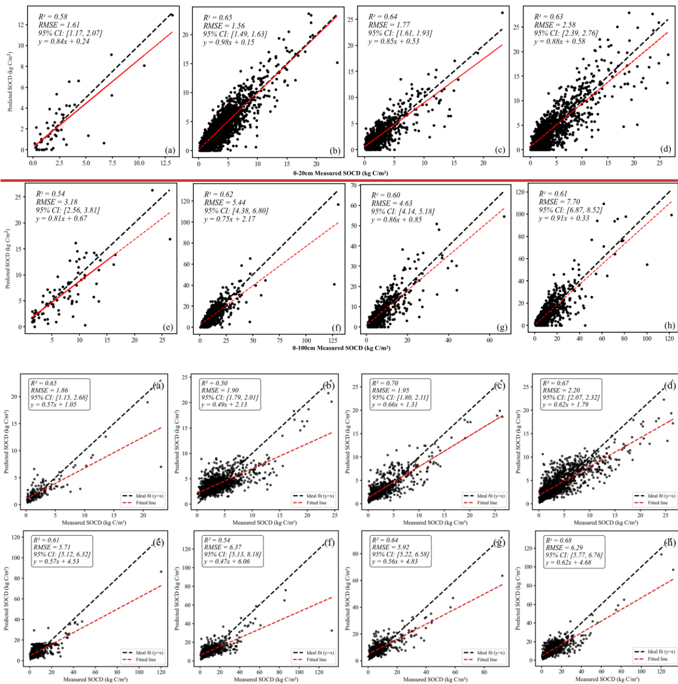
Figure 7. The model performance of different zoning models with the depth of 0-20 cm and 0-100 cm. Panels (a) and (e) depict the model performance for arid regions, where water scarcity is a predominant factor affecting SOCD. Panels (b) and (f) illustrate results for humid regions characterized by high moisture availability. Panels (c) and (g) showcase semi-arid regions, where the balance between precipitation
