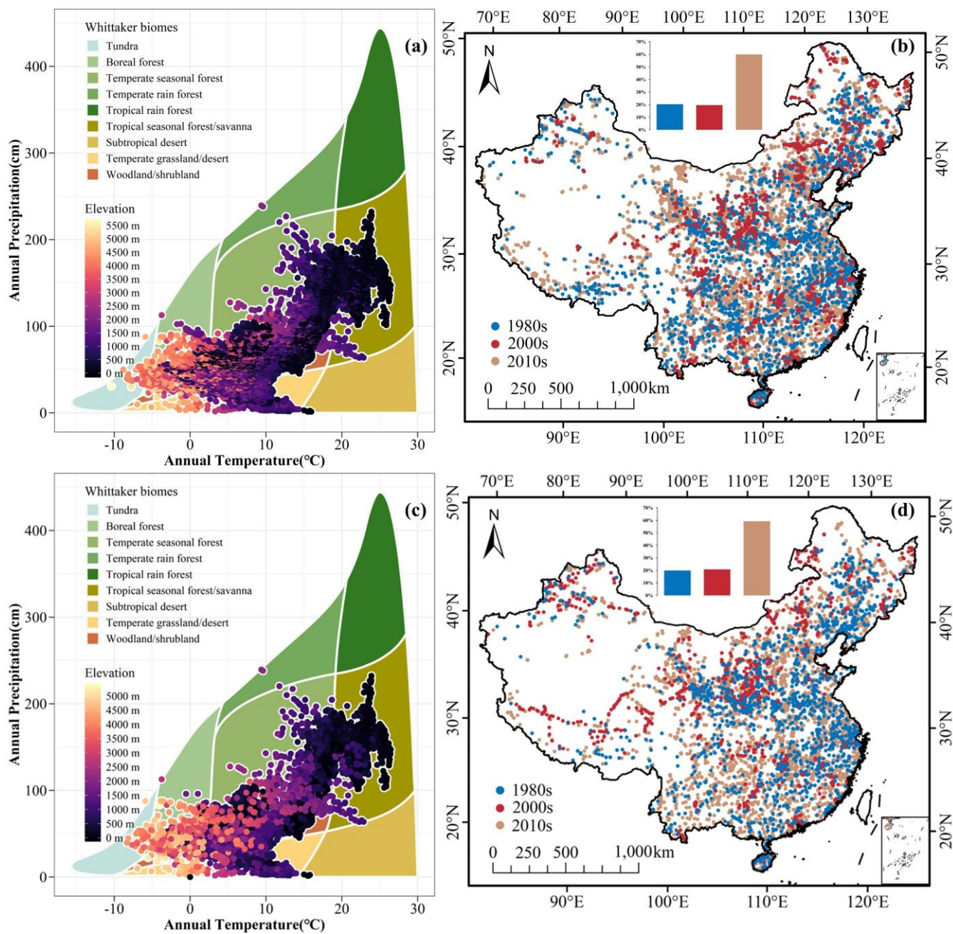
Figure 5. Spatial distribution of SOC soil sample points with depth of 0-20 cm (b) and 0-100 cm (d). And the Whittaker biomes of soil sample points with depth of 0-20 cm and 0-100 cm are shown in (a) and (c). Spatial distribution of SOC sample points. (a-d) Distribution of the SOCD sampling sites with data used in this study for (b) top 20 cm soil and (d) top 100 cm soil. The distribution of site-level training data is based on Whittaker biomes for (a) top 20 cm soil and (c) top 100 cm soil.
