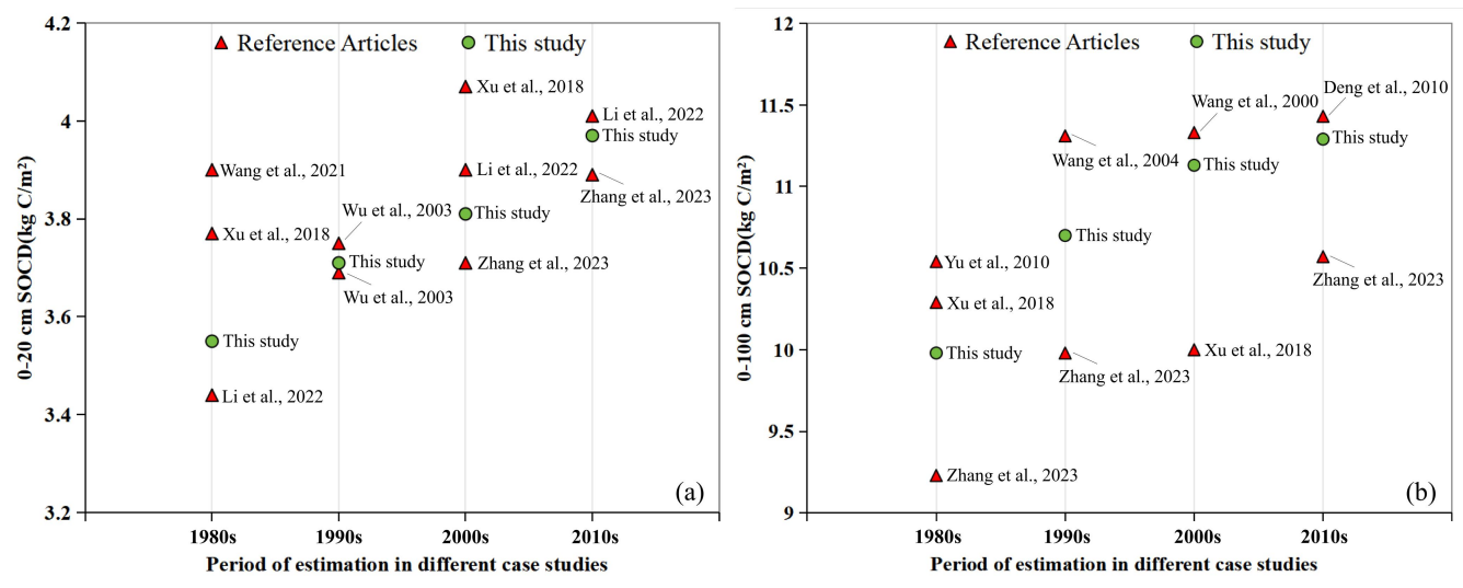
590 Figure 12. Aggregated results of estimated SOC D with the depth of 0-20 cm (a) and 0-100 cm (b) in China from this study
