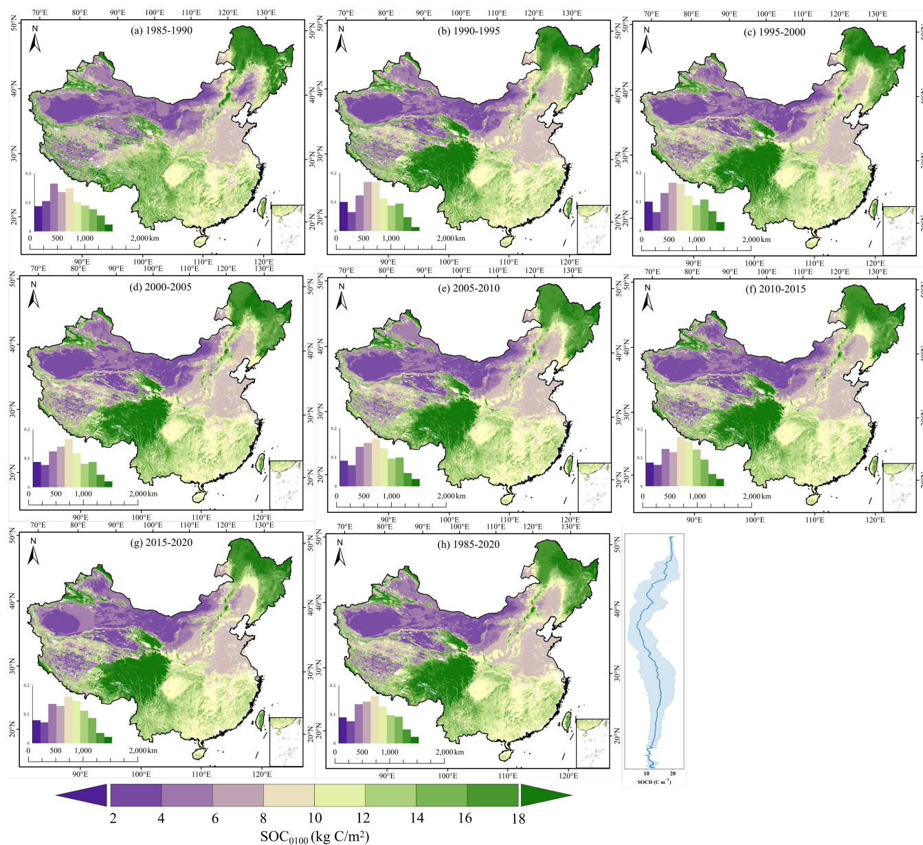
Figure 14. Spatial distribution of estimated SOC at a depth of 0-100 cm in 1985-1990 (a), 1990-1995 (b), 1995-2000(c), 2000-2005 (d), 2005-2010 (e), 2010-2015 (f), and 2015-2020 (g) and average from 1985 to 2020 (h). The lower left histograms in each panel show the
