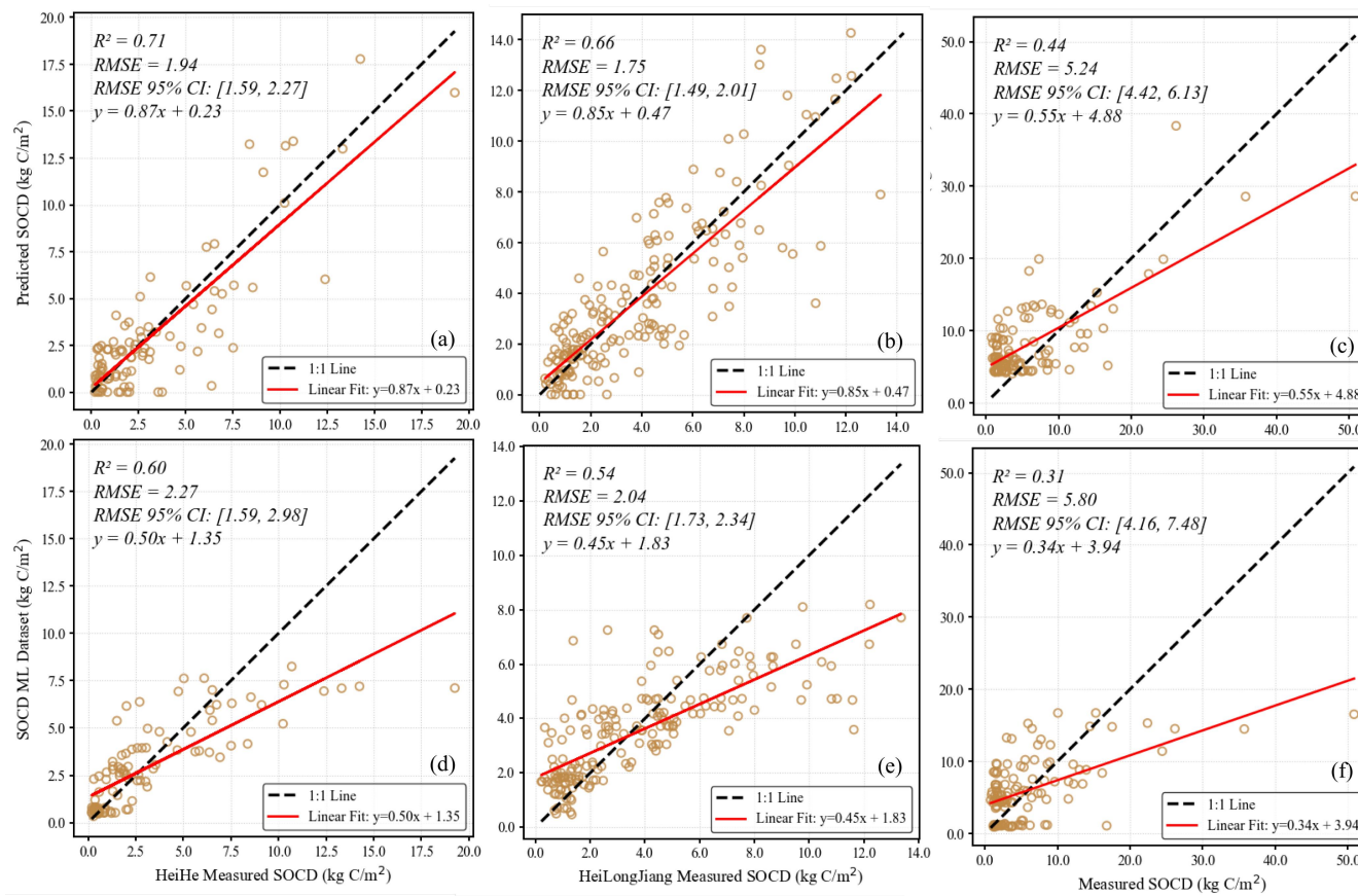
Figure 9. Comparison of predicted and machine learning (ML) derived SOCD with independent measurements at various depths. Panels (a), (b), and (c) display correlations of this study's predicted SOCD, while (d), (e), and (f) show correlations of SOC Dynamics ML dataset. Specifically, (a) and (d) are for 0-20 cm SOCD against Heihe River basin measurements. (b) and (e) compare 0-20 cm SOCD with Xu's published data. (c) and (f) present 0-100 cm SOCD correlations with measurements from Dong et al. (2024) and simulations from Li et al. (2022).
