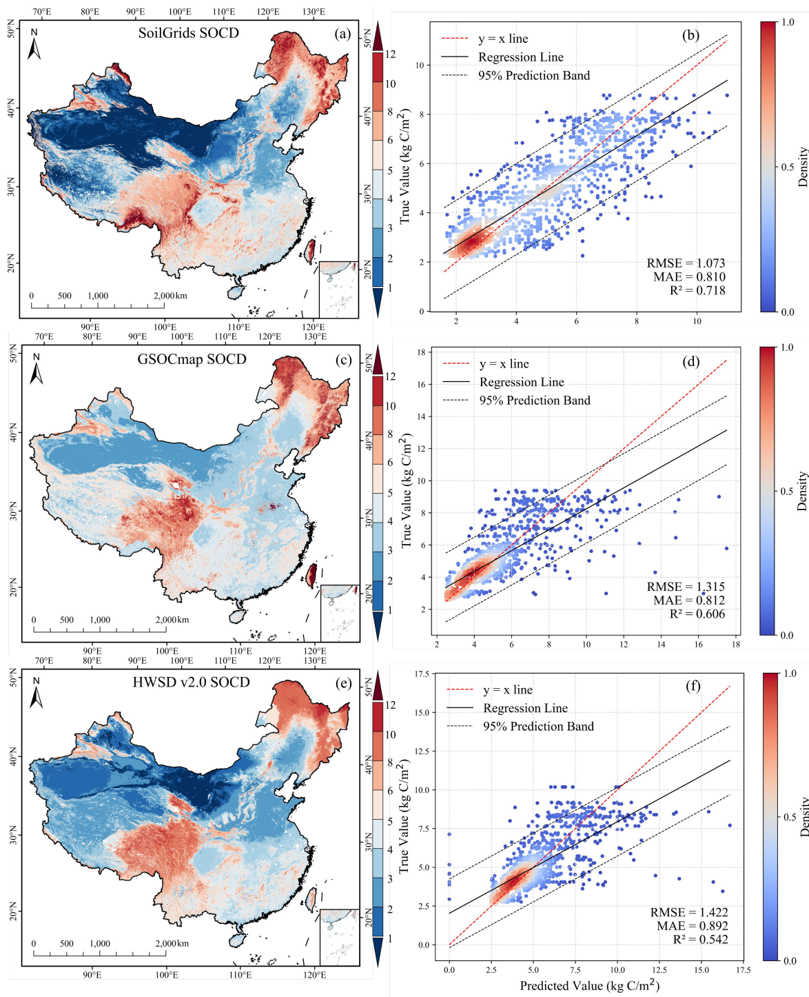
585 Figure 10. Comparison with three published global products. Our estimated SOCD is compared with the SoilGrids250m (a & b), GSOCmap (c & d), and HWSD v2.0 (e & f) datasets.
