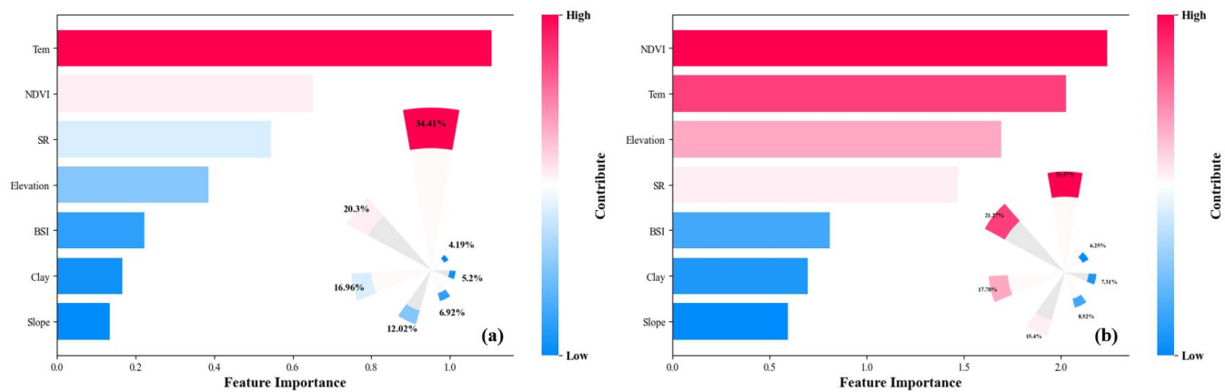
570 Figure 8. Importance ranking of features for SOCD estimation with the depth of 0-20 cm and 0-100 cm. It reports the contribution of different environmental variables to the SOCD estimation with different soil depths, including feature importance ranking for 0-20 cm depth (a) and feature importance ranking for 0-100 cm depth (b).
