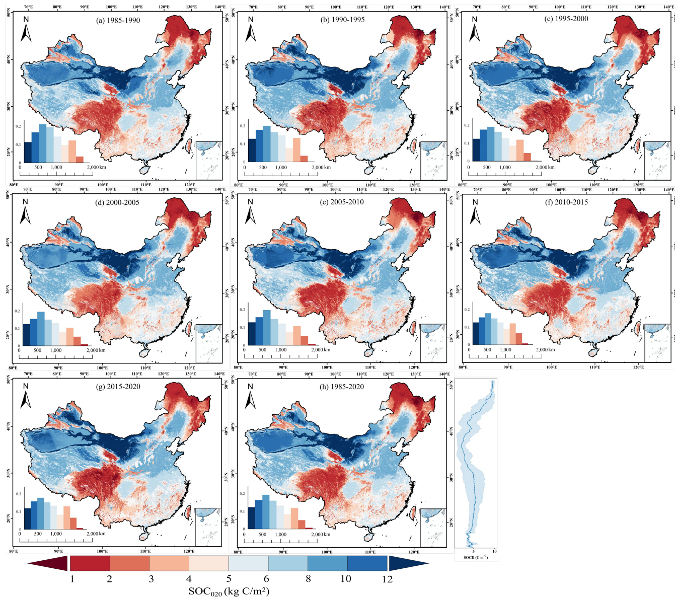
Figure 13. Spatial distribution of estimated SOC D at a depth of 0-20 cm in 1985-1990 (a), 1990-1995 (b), 1995-2000(c), 2000-2005 (d), 2005-2010 (e), 2010-2015 (f), 2015-2020 (g) and average from 1985 to 2020 (h). The lower left histograms in each panel show the area
