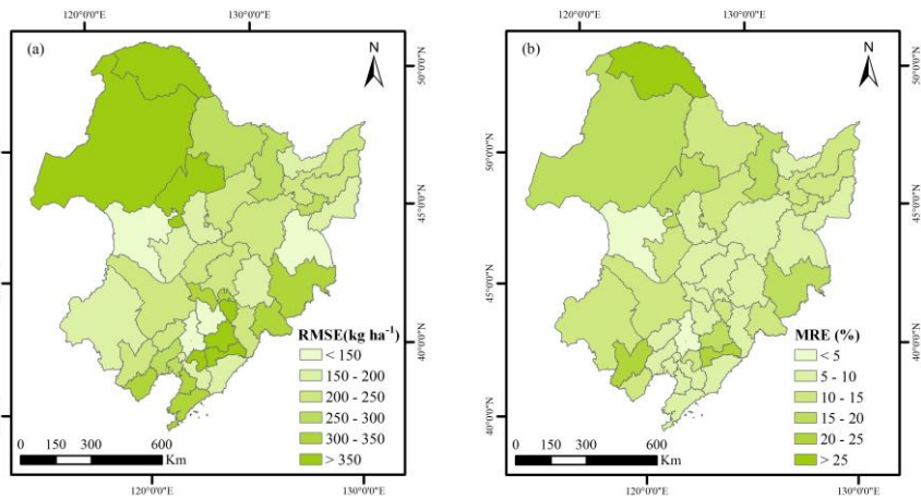
Figure 7: Spatial patterns of the mean value of the root mean squared error and mean relative error between model estimated yields from Sentinel-2 and statistical yields from 2019 to 2022 (excluding 2023 for which no statistical data was not available from the government), (a) and (b), respectively. For years from 2019 to 2021, a total of 40 cities were calculated. For 2022, 32 cities were calculated due to missing statistics.
