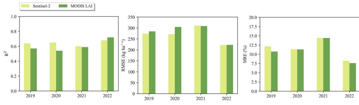
Figure 13: Comparison of accuracy evaluation results for soybean yield estimation in 2019 – 2022 (excluding 2023, for which no statistical data was reported) using Sentinel-2 and MODIS LAI data, respectively.
