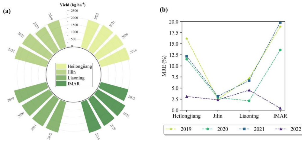
Figure 10: Accuracy of the soybean yield estimation at provincial scale in Northeast China from 2019 to 2022. (a) represents the change in estimated yield for each province through the years; (b) represents the MRE of results compared with statistical yield for each province
