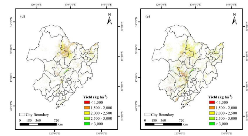
Figure A5: Spatial distribution of annual soybean yield derived from Sentinel-2 before calibration in Northeast China from 2019 to 2023.
