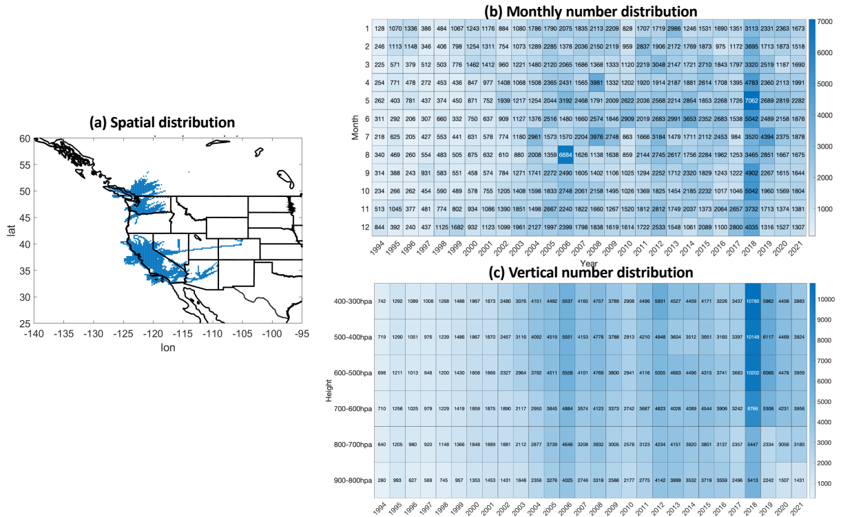
Figure 1: The distribution of defined data receptors from the data fusion product: (a) spatial pattern over WNA, (b) number of receptors by month of year across 28 years, (c) number of receptors divided by vertical layers with 100 hPa intervals across 28 years.
