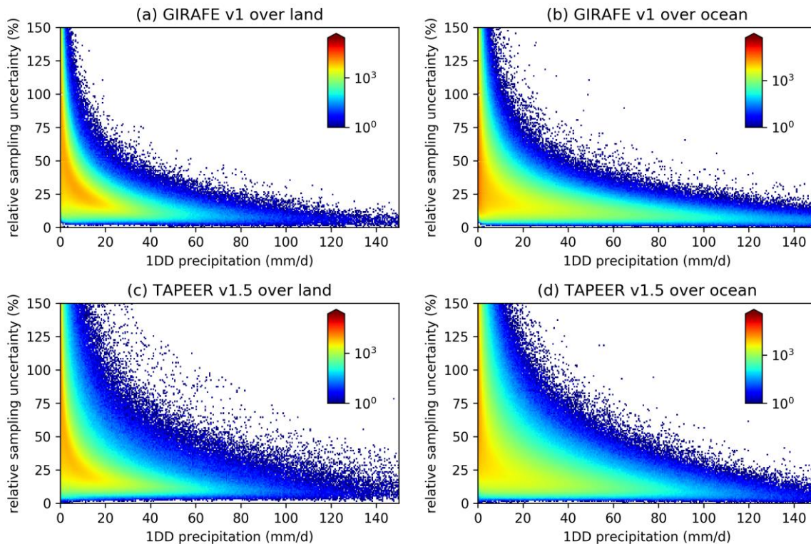
Figure 14: Two-dimensional histograms of the 1DD relative sampling uncertainties and the 1DD precipitation in GIRAFE v1 (a and b) and TAPEER v1.5 (c and d) from all 1DD grid cells in 2012-2021 inside 30°N/S (TAPEER v1.5 coverage), for which the decorrelation scales had not been replaced by default values in GIRAFE v1 (see section 4.4), separately for land (a and c) and ocean (b and d).
