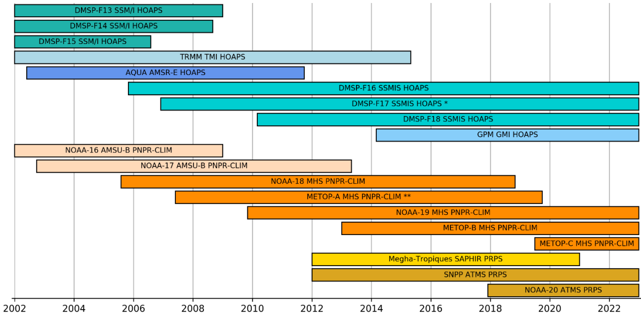
Figure 3: Overview over satellites bearing PMW sensors and their temporal availability used in GIRAPE v1. The labels indicate satellite, instrument and the corresponding precipitation retrieval algorithm, see also Table 2. Identical instruments are identified by the same colour; *quantile mapping target over ocean (section 4.2); **quantile mapping target over land.
