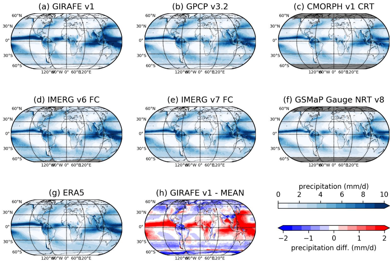
Figure 8: Spatial distributions of climatological mean precipitation (2002-2020) for various datasets (a-g); panel h: difference between GIRAFE v1 climatological mean (panel a) and the ensemble mean of the other datasets (panels b-g).
