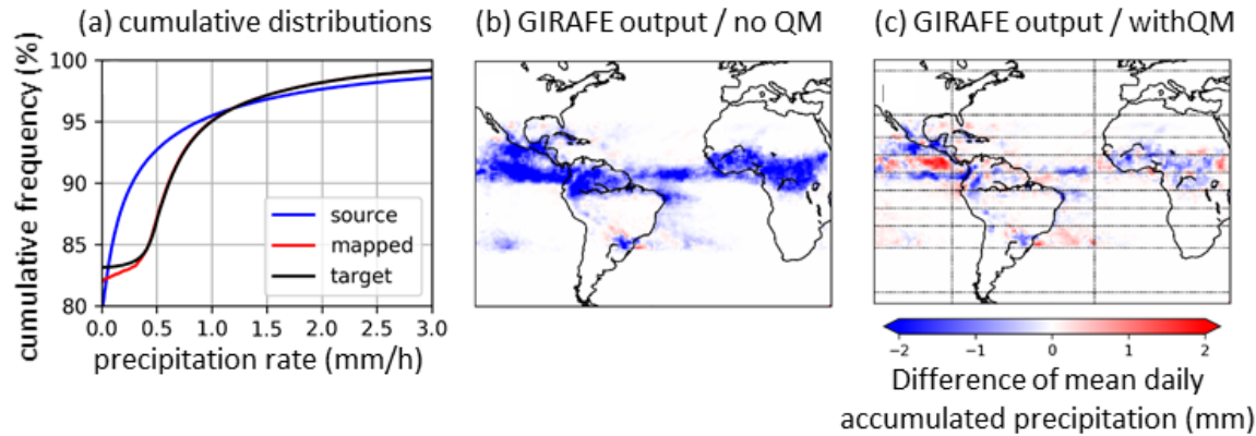
800 Figure A1: (a) Exemplary cumulative distributions for METOP-A MHS PNPR-CLIM (“target”; black) and Megha-Tropiques SAPHIR PRPS (MT from here; “source”; blue) from instantaneous observations in June at latitudes inside 4°N/S over South American land. The MT distribution after quantile mapping has been applied (“mapped”; red) is also shown. (b) Differences in GIRAFE daily accumulated precipitation with and without MT instantaneous data averaged over June 2014. Here, quantile mapping has not been applied. (c) Same as (b) but with quantile mapping applied. The lines delineate the latitude/longitude bands in which the cumulative distributions are collected. Note that the results in (b) and (c) depend not only on the data forming the distributions shown in (a), but also on those in the other latitude/longitude bands, depending on the location. 805
