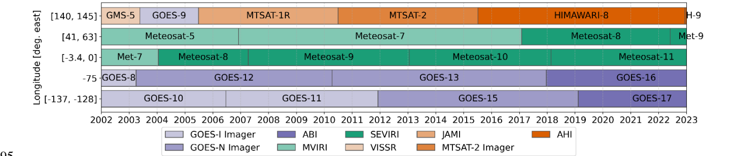
Figure 2: Geostationary platforms and their temporal coverage as used in GIRAFE v1. The respective instruments are color-coded, see also Table 1. The labels on the vertical axis indicate the sub-satellite longitude range of the platforms in the respective position. H-9 = HIMAWARI-9, Met-9 = Meteosat-9.
