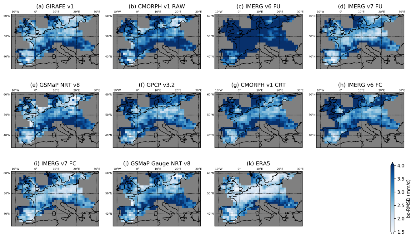
460 Figure 7 Maps of the bc-RMSD in the 1DD precipitation for the validated datasets against EURADCLIM. The datasets appear in the same order as in Table 5. Panels (a)-(e) represent the unadjusted datasets and, (f)-(j) represent the adjusted datasets, and panel (k) represents the ERA5 reanalysis. GIRAFE v1 has been analysed without the application of the snow flag. The analysis of CMORPH v1 RAW (panel (b)) ends in July 2017; all other comparisons extend over mutually available grid cells in the 2013-2020 period.
