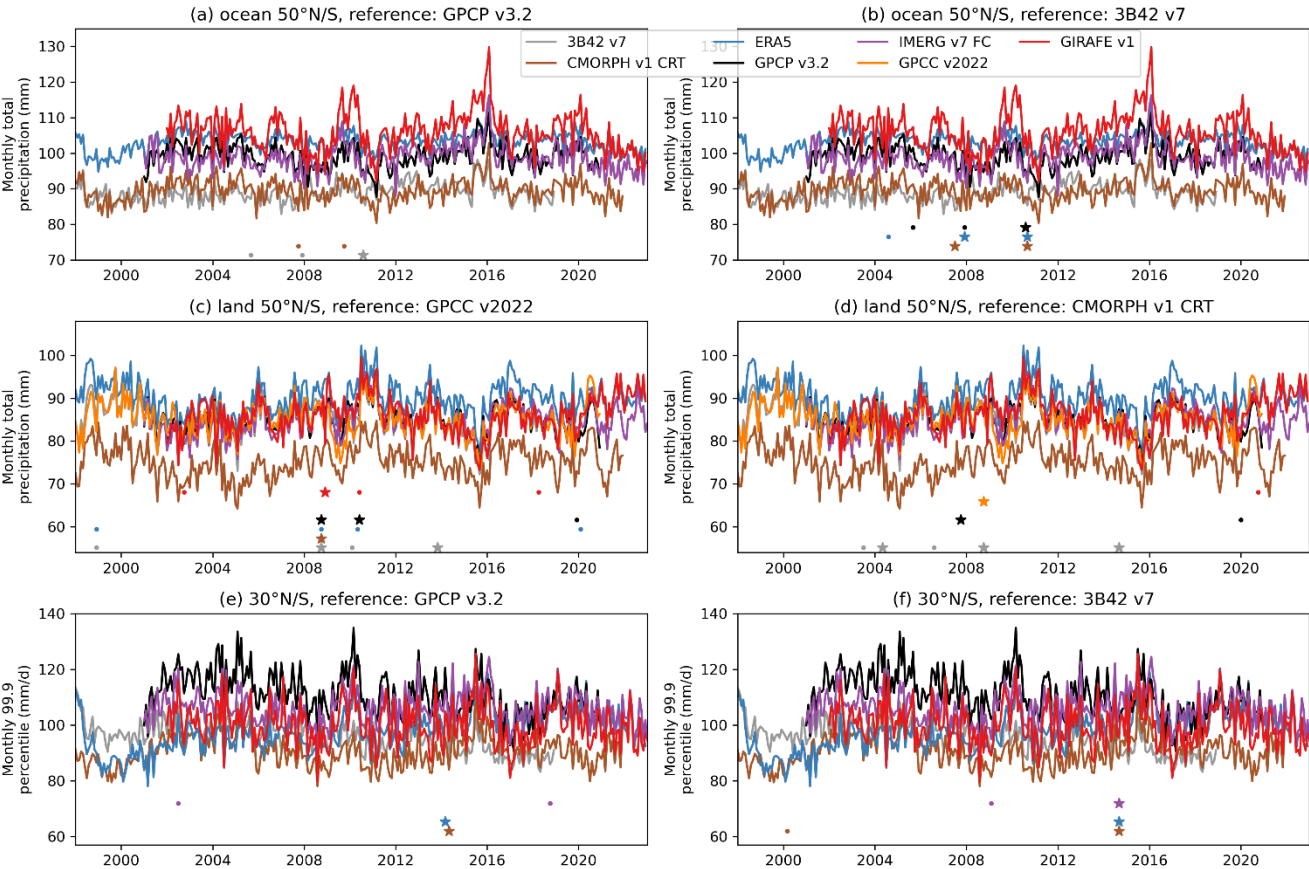
Figure 10: Homogeneity analysis. (a) Monthly total precipitation over ocean in 50°N/S with GPCP v3.2 as reference dataset for the homogeneity tests. (b) Same with 3B42 v7 as reference dataset. (c) Monthly total precipitation over land in 50°N/S with GPCC v2022 as reference dataset for the homogeneity test. (d) Same with CMORPH v1 CRT as reference dataset. (e) 99.9 percentile of precipitation over land and ocean in 30°N/S with GPCP v3.2 as reference dataset for the homogeneity test. (f) Same with 3B42 v7 as reference dataset. The timeseries (identical in left and right column per row) illustrate the anomaly in the respective dataset shifted by the respective overall mean. Small, circle-shaped markers indicate the presence of breakpoints detected by the PMF test only. Breakpoints illustrated by large, stars-shaped markers are also confirmed by the SNH test. A complete list of detected breakpoints is given in Appendix C. Note that some timeseries start between January 1998 and January 2002 or end prior to December 2022, deviating from the GIRAFE v1 coverage.
