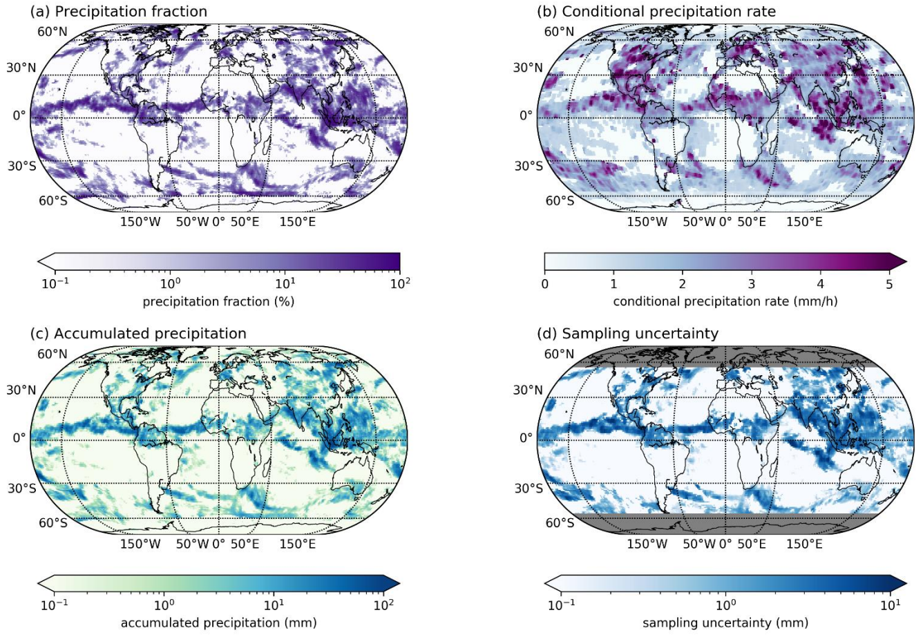
Figure 4: Example fields for the GIRAFE v1 precipitation fraction F (panel a), the conditional precipitation rate R (panel b), the resulting daily accumulated precipitation P_{acc} (panel c), and the sampling uncertainty \sigma_s (panel d) on July 13 th 2021. The minimum values of the fields illustrated in panels a, c, and d using logarithmic color-scales are zero.
