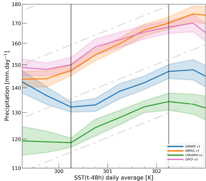
Figure 12: The 99.9th percentile of the daily distribution as a function of the 48h-lagged underlying SST for several products, including GIRAFE v1. The lines correspond to the 50-member ensemble mean and the shading represent the standard deviation. The vertical lines delineate the central section of the distributions representing the majority of the data (see main text).
