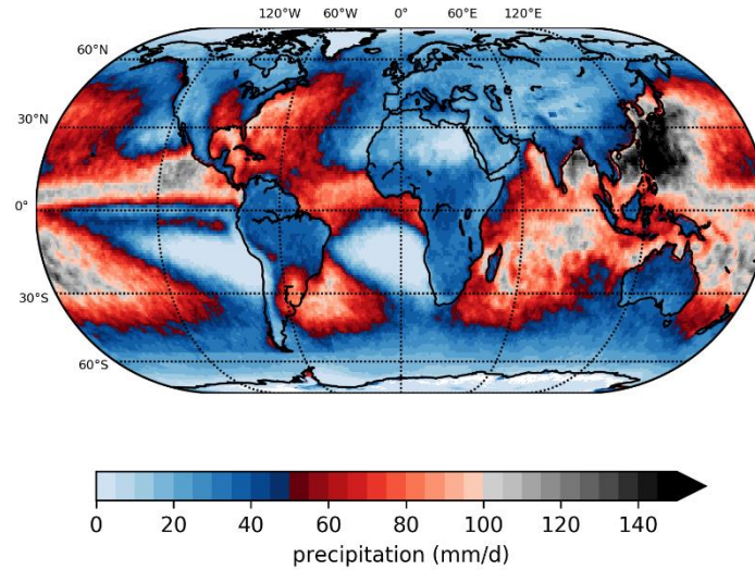
615 Figure 11: Map of the 2002-2020 multi-year mean of the annual 99.9th percentile of GIRAFE v1 daily precipitation (mm/d).
