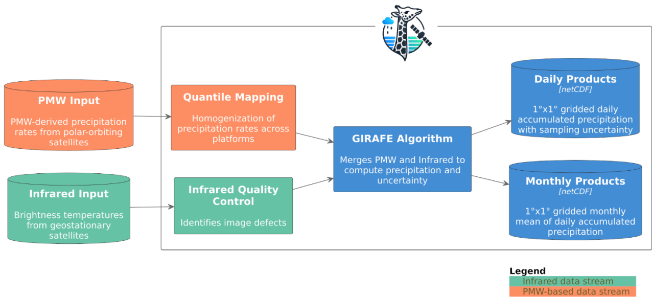
Figure 1: Overview of the algorithm and data streams.
