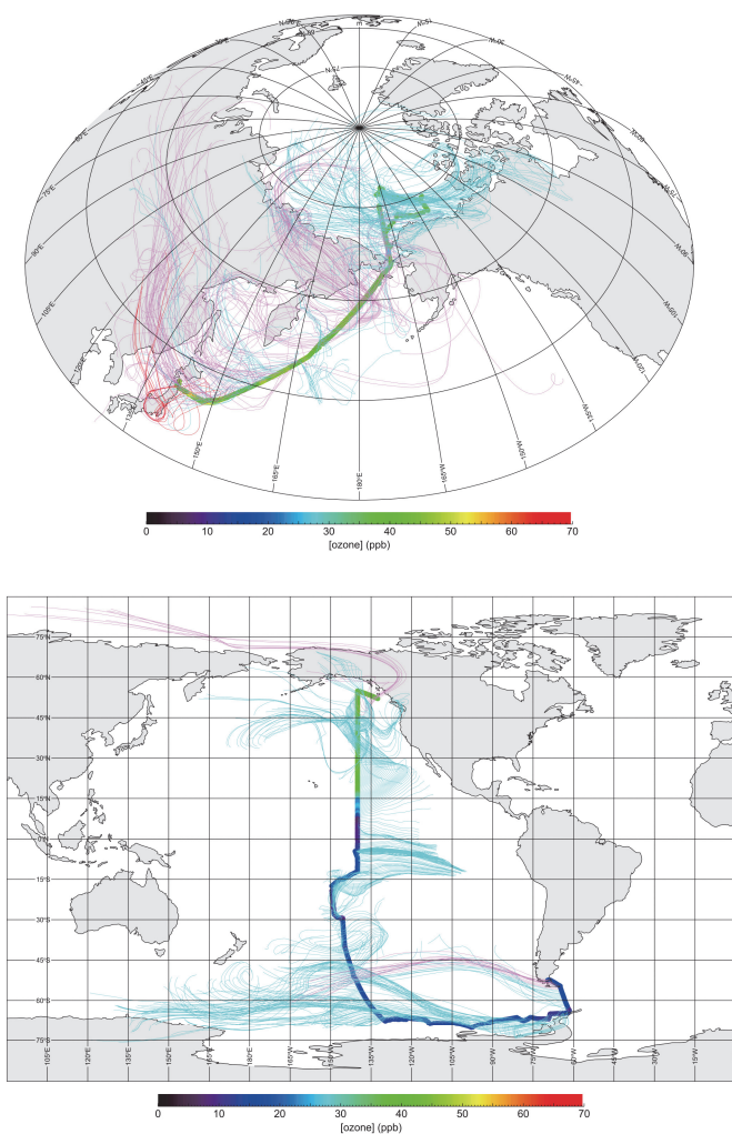
Figure 2. Backward trajectories (120-h long) for observations with oceanic conditions essentially marine (grey/light blue) and apparently land-influencing (purple) air masses conditions, as assessed with the LCL72 criterion during (top) the MR19-03C observations from 29 Sep 2019 to 10 Nov 2019 and (bottom) the RITS94 observations from 23 Nov 1993 to 6 Jan 1994. The red lines indicate cases where the observed O 3 mixing ratio is greater than 50 ppb.
