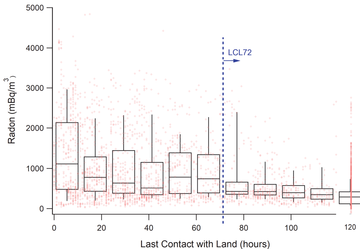
835 Figure 3. Decrease of Radon concentrations with Last Contact with Land from backward trajectory analysis. ACE-1, ACE-Asia, ATOMIC, ICEALOT, NAAMES1-4, and WACS data were used in combination. Radon data by NOAA PMEL. The blue dotted line indicates the adopted LCL72 criterion. Boxes and whiskers represent 10, 25, 50, 75 and 90 percentiles.
