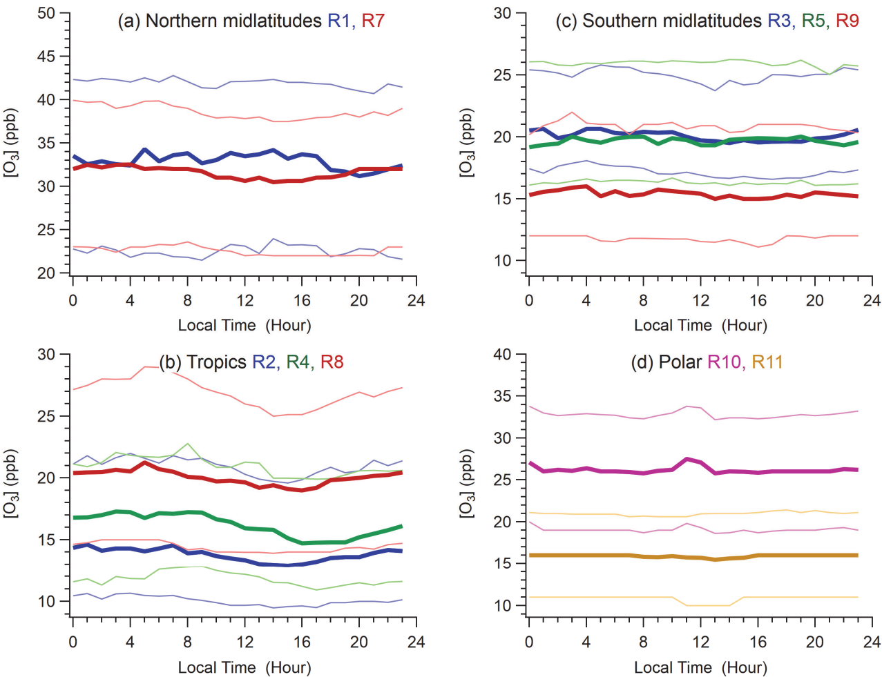
Figure 6. Hourly median (thick lines) and interquartile levels (thin lines) and their diurnal variation by regions. (a) R1 and R7 855 (Pacific and Atlantic northern midlatitudes), (b) R2, R4, and R8 (Pacific, Indian, and Atlantic low latitudes), (c) R3, R5, and R9 (Pacific, Indian, and Atlantic southern midlatitudes), and (d) R10 and R11 (Polar, i.e., Arctic and Antarctic regions). The blue, green, and red line colors correspond to the Pacific, Indian, and Atlantic Oceans.
