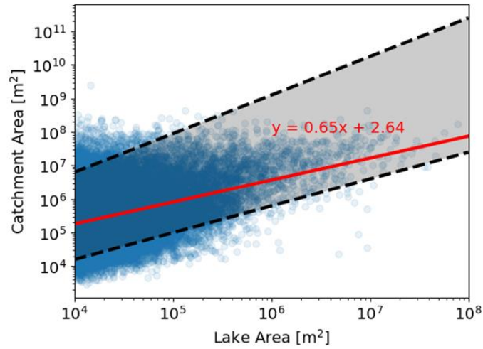
290 Figure A3: Relationship between lake/ pond and catchment area for all lakes & ponds > 10.000 m 2 (1 ha). The red line shows a fitted linear regression line between log 10 of lake area and catchment area. The shaded area represents the span of linear relationships between lake and catchment area described by Walter et al. (2020).
