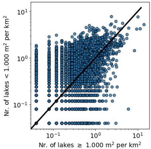
Figure A1: Relationship between density of lakes ≥ 1,000 and lakes < 1,000 m 2 . The number of lakes refers to the lakes within each 5 x 5 km grid cell, as shown in Fig.1. The black line represents the 1:1 line.
